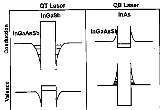
FIG. 6. Qualitative band-bending diagrams for the QT and QB lasers.
