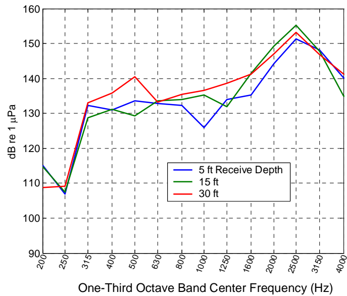
Figure C-7. Receive pressure spectrum from e LOUD™ system at 100 yard range.
