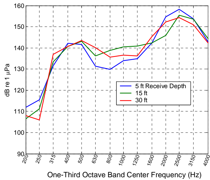
Figure C-6. Receive pressure spectrum from e LOUD™ system at 50 yard range.
