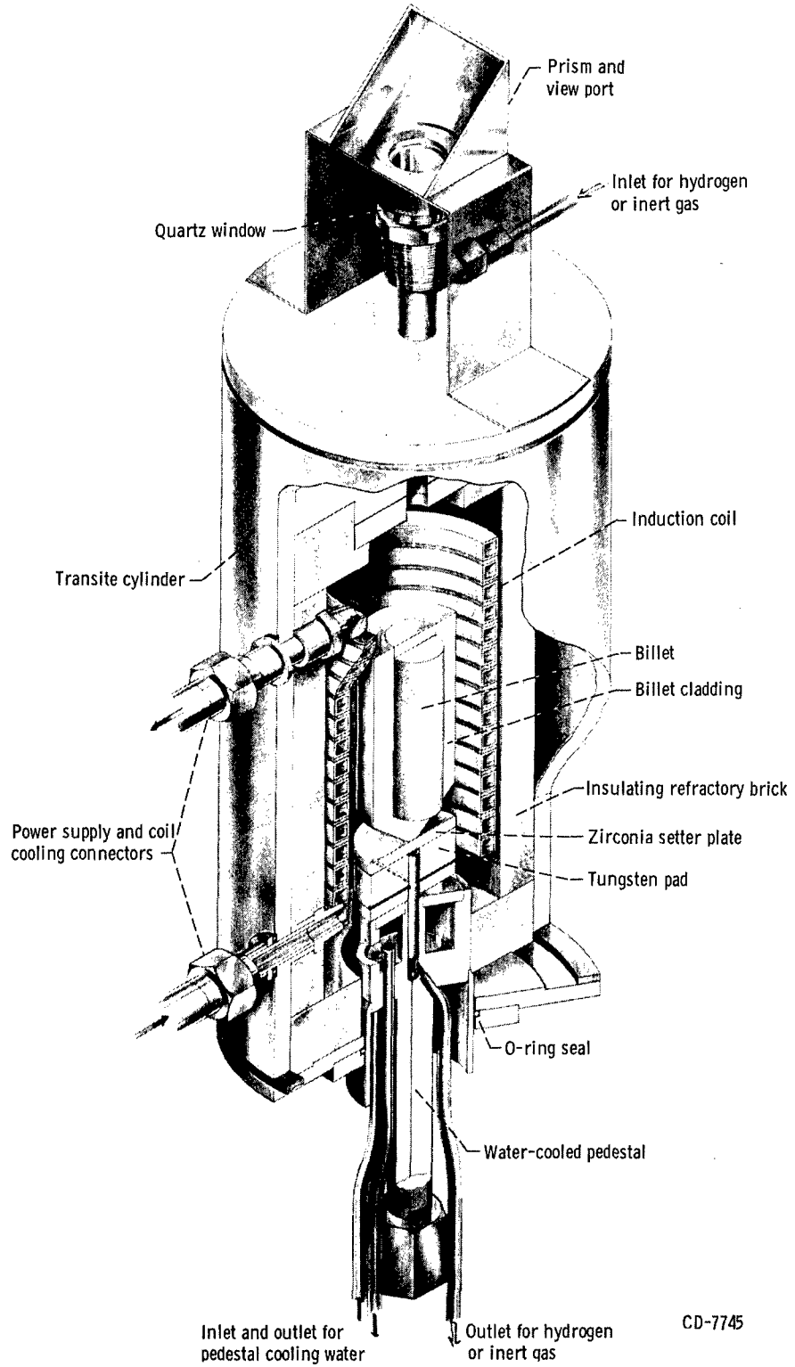
Figure 11. - High-temperature, hydrogen atmosphere, extrusion preheat furnace.
