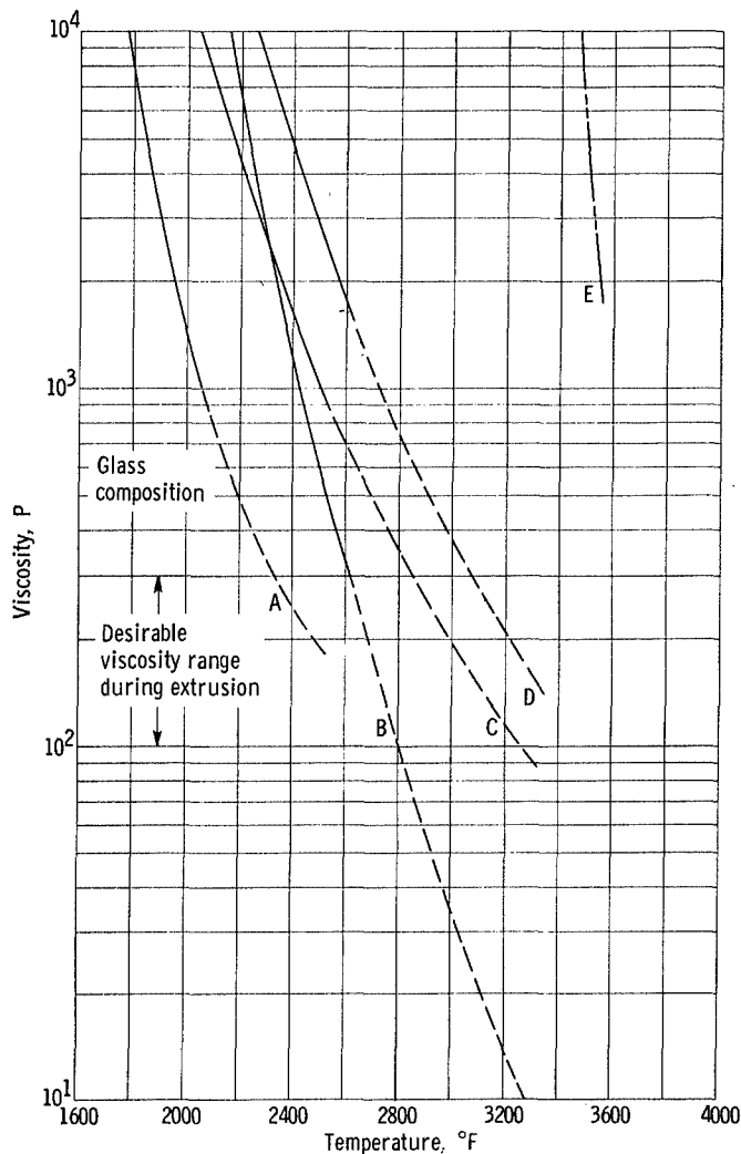
Figure 10. - Viscosity of various glasses as a function of temperature. (Data from ref. 2.)
