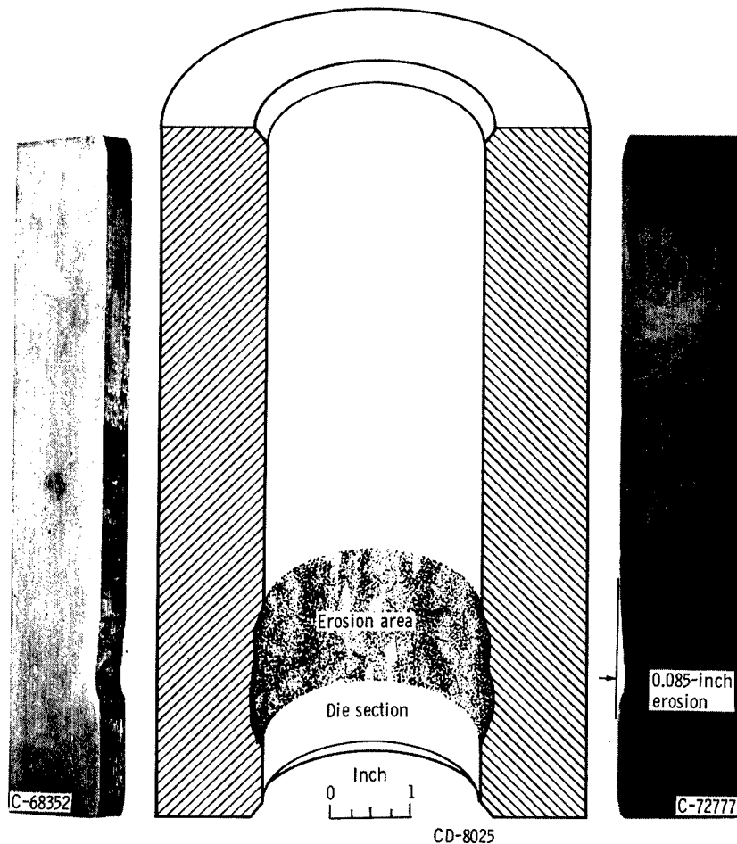
Figure 4. - Nominal 2-inch-diameter container liner number 6 eroded 0.085 inch at juncture of billet and die after 106 high-temperature extrusions.
