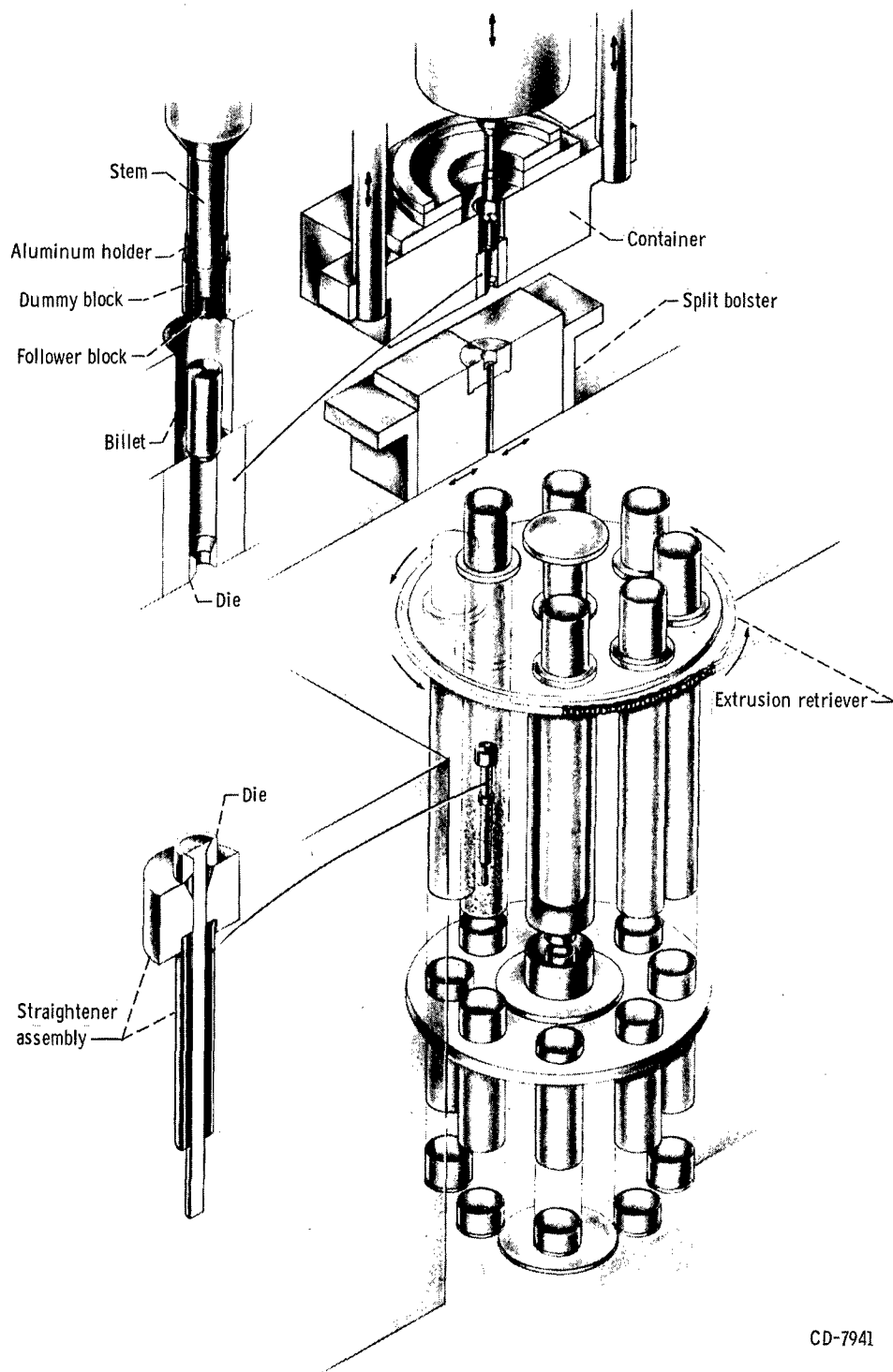
Figure 6. - Extrusion-tooling alinement.
