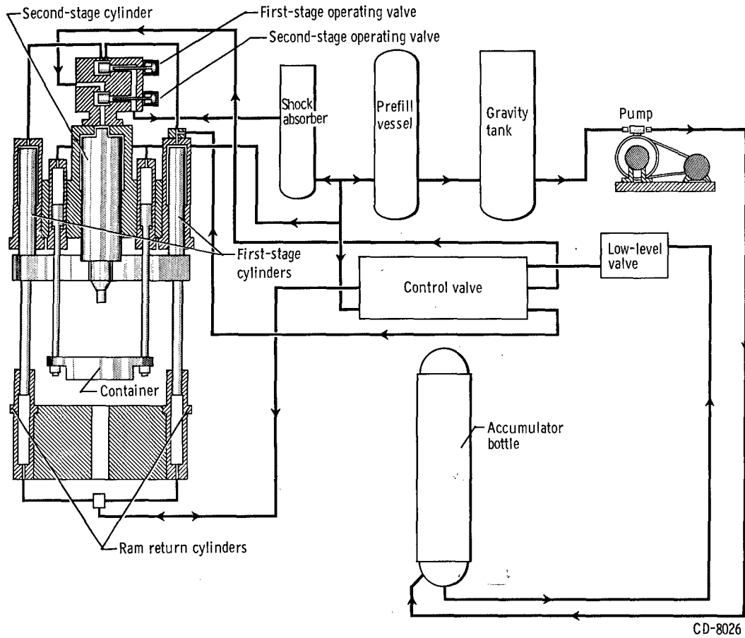
Figure 2. - Hydraulic diagram for 1020-ton extrusion press.
