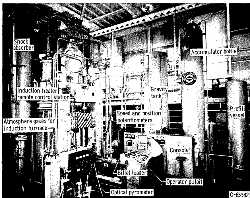
Figure 1. - 1021-Ton water hydraulic extrusion-forging press.
