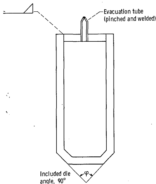
Figure 9. - Schematic drawing of canned billet. Type of canning material, as required by billet.
