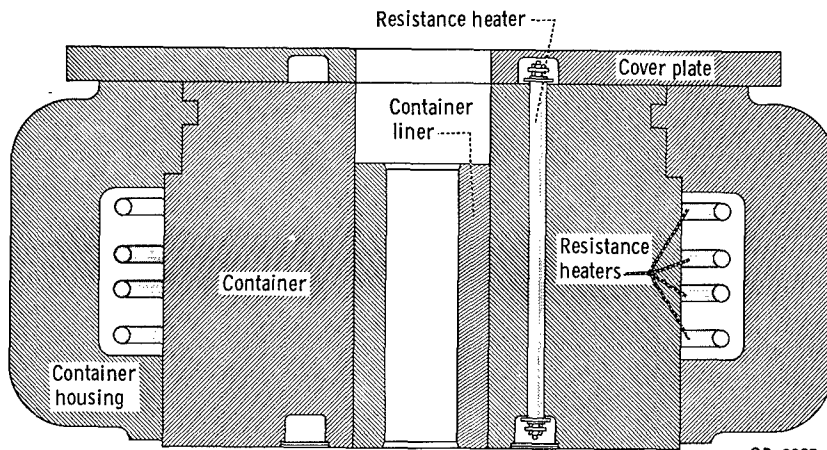
Figure 3. - Schematic drawing of container assembly used in extrusion.
