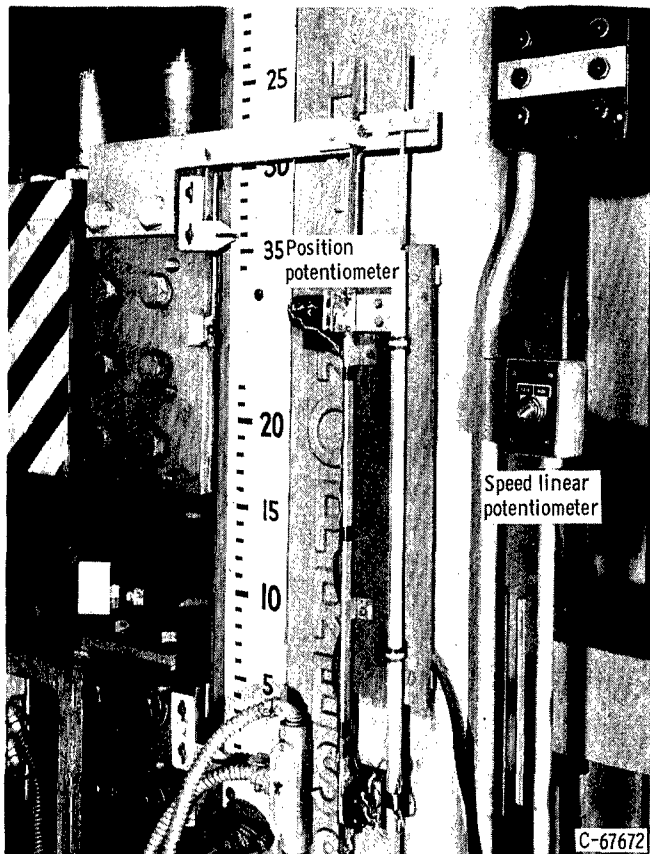
Figure 12. - Stem position and velocity potentiometers.
