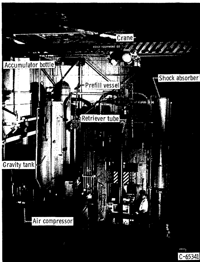
Figure 8. - Rear view of press with retriever retracted from extrusion pit.
