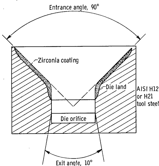
Figure 5. - Cross section of coated extrusion die.
