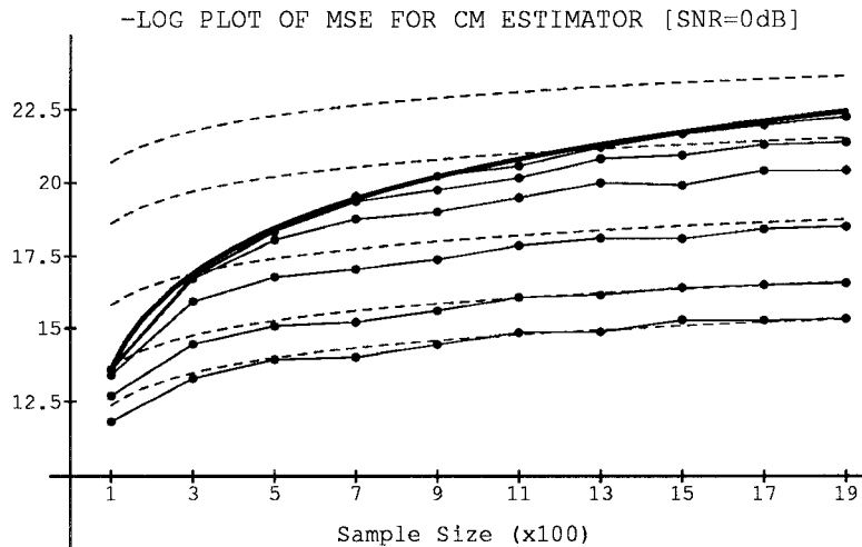
Figure 1: -\text{Log} plot of MSE of the CM estimator for (from the bottom) \eta=0.85, 0.90, 0.95, 0.98, 0.99, \text{ and } 0.999 . The dashed lines (---) are asymptotic variances of the CM estimator for (from the bottom) \eta=0.85, 0.90, 0.95, 0.98, \text{ and } 0.99 . The solid line is the asymptotic variance of the NLS.
