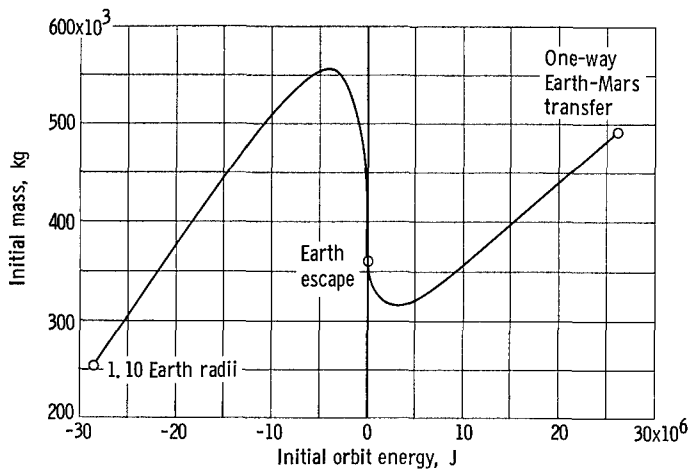
Figure 21. - Nature of optimums obtained with initial high-thrust assist. Mission time, 450 days; wait time, 40 days; specific powerplant mass, 7 kilograms per kilowatt; Earth atmospheric entry velocity, 15 820 meters per second; specific impulse, 425 seconds.
