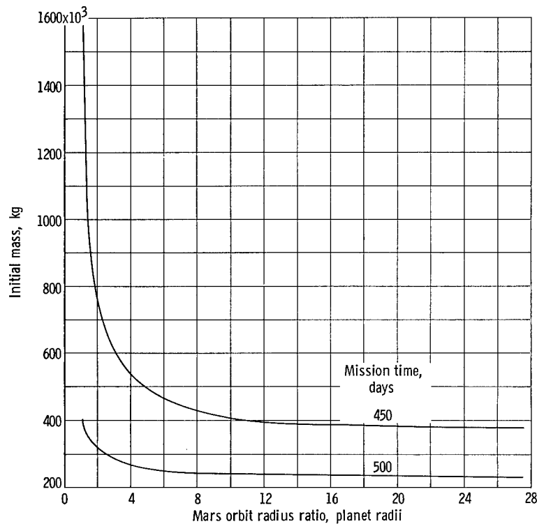
Figure 15. - Effect of Mars orbit radius on initial mass. Wait time, 40 days; specific powerplant mass, 7 kilograms per kilowatt; Earth atmospheric entry velocity, 15 820 meters per second.
