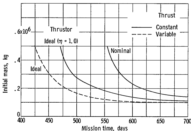
Figure 12. - Effect of thrustor type and efficiency. Wait time, 48 days; specific powerplant mass, 7 kilograms per kilowatt; unmanned belt traversal.
