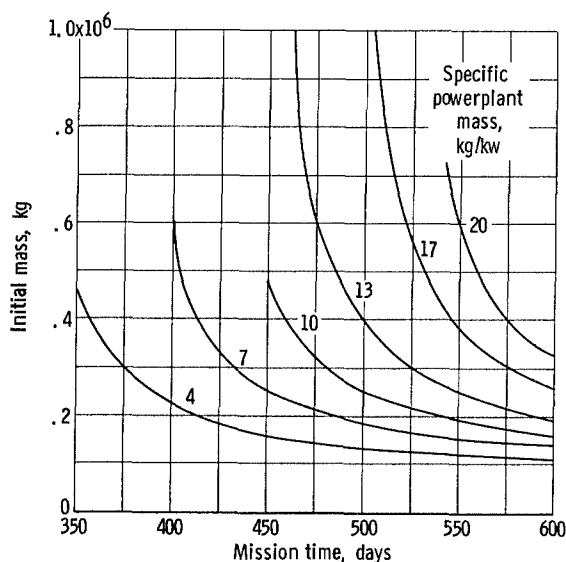
Figure 16. - Effect of specific powerplant mass. Wait time, 40 days; unmanned belt traversal; chemical plus electric braking, to 15 820 meters per second.
