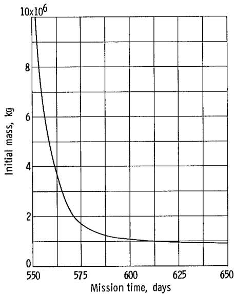
Figure 7. - Initial mass using nominal mission profile. Seven-man Mars mission; wait time, 40 days; specific powerplant mass, 7 kilograms per kilowatt.
