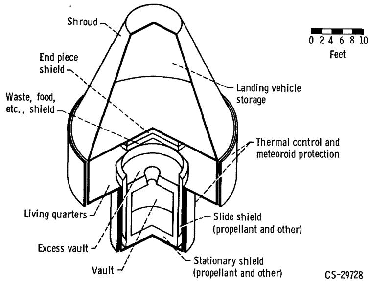
Figure 2. - Typical crew-cabin living-quarters configuration for seven-man Mars mission.
