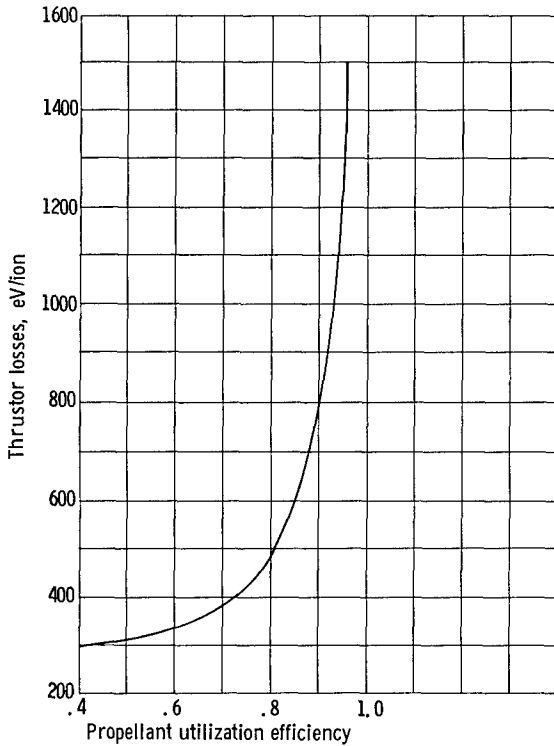
(a) Thruster losses (discharge only).
