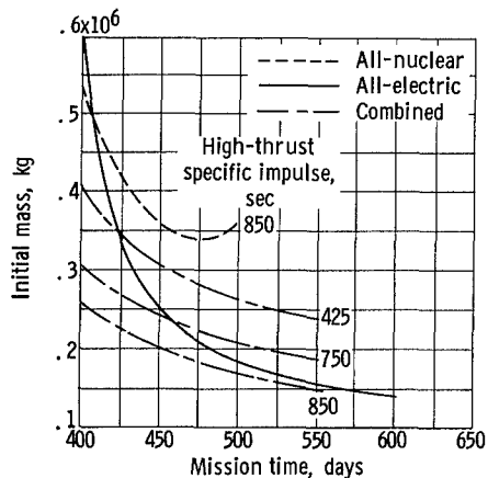
Figure 20. - Comparison of all-nuclear, all-electric, and combined systems. Wait time, 40 days; specific powerplant mass, 7 kilograms per kilowatt; Earth atmospheric entry velocity, 15 820 meters per second.
