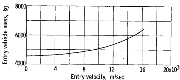
Figure 3. - Estimated Earth atmospheric entry vehicle mass for seven-man crew.
