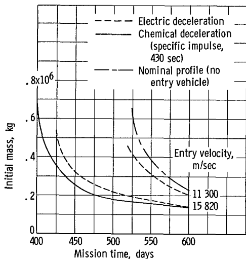
Figure 10. - Effect of atmospheric braking. Seven-man Mars mission; wait time, 40 days; specific powerplant mass, 7 kilograms per kilowatt; unmanned belt traversal.
