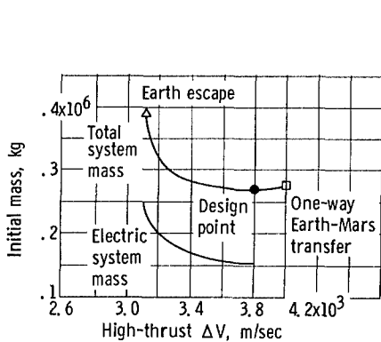
Figure 19. - Effect of high-thrust propulsion on combined system mass. Mission time, 400 days; wait time 40 days; specific power-plant mass, 7 kilograms per kilowatt; Earth atmospheric entry velocity, 15 820 meters per second; high-thrust specific impulse, 850 seconds.
