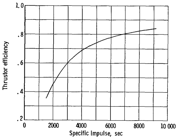
(b) Maximum thruster efficiency.
