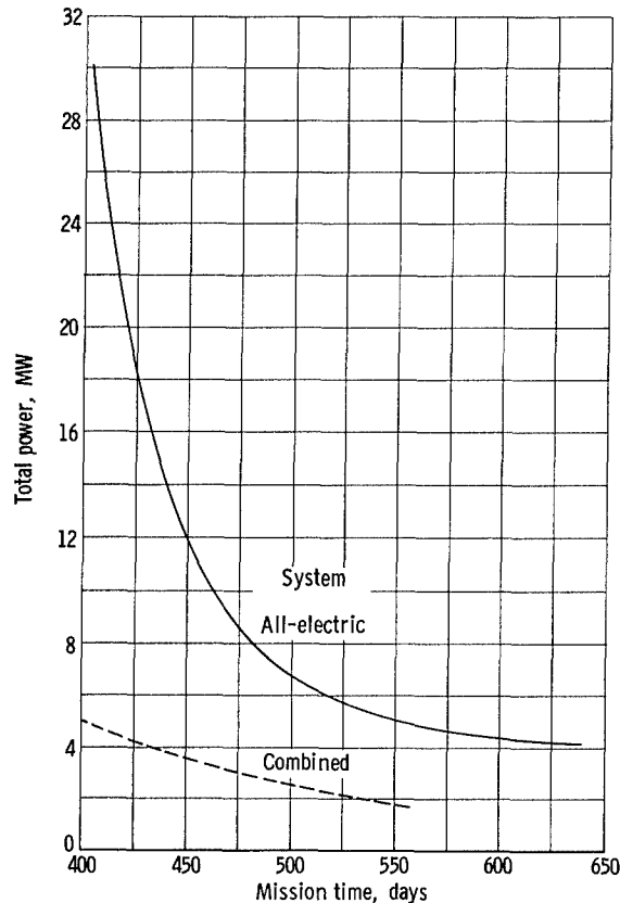
Figure 22. - Comparison of total power required for all-electric and combined systems. Seven-man Mars mission; wait time, 40 days; specific powerplant mass, 7 kilograms per kilowatt; Earth atmospheric entry velocity, 15 820 meters per second; nuclear rocket specific impulse, 850 seconds.
