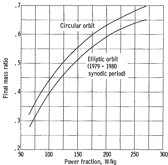
Figure 5. - Noncircular orbit effects on typical round-trip mass ratios. Mission time, 420 days (including four spiral maneuvers); wait time, 30 days (no exploration assumed).
