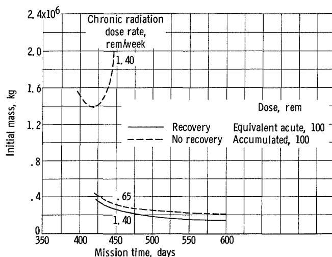
Figure 14. - Effect of dose recovery on initial mass for 100-rem maximum equivalent acute or accumulated dose. Wait time, 40 days; specific powerplant mass, 7 kilograms per kilowatt; Earth atmospheric entry velocity, 15 820 meters per second.
