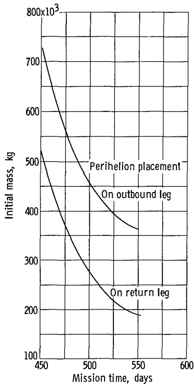
Figure 9. - Comparison of perihelion placement technique. Seven-man Mars mission; wait time 40 days; specific powerplant mass, 4 kilograms per kilowatt.
