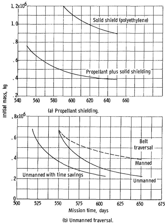
Figure 8. - Comparison of various methods of reducing Van Allen belt radiation. Wait time, 40 days; specific powerplant mass, 7 kilograms per kilowatt.
