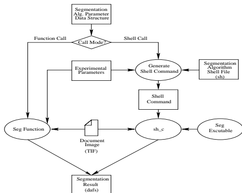
Figure 12: Page segmentation algorithm calling modes: function call and shell call. The left half represents the function calling mode and the right half represents the shell calling mode. The shell calling mode can be used only when the algorithm executable is available; otherwise the function calling mode can be used. Note that the executable is called by the function sh_c .
