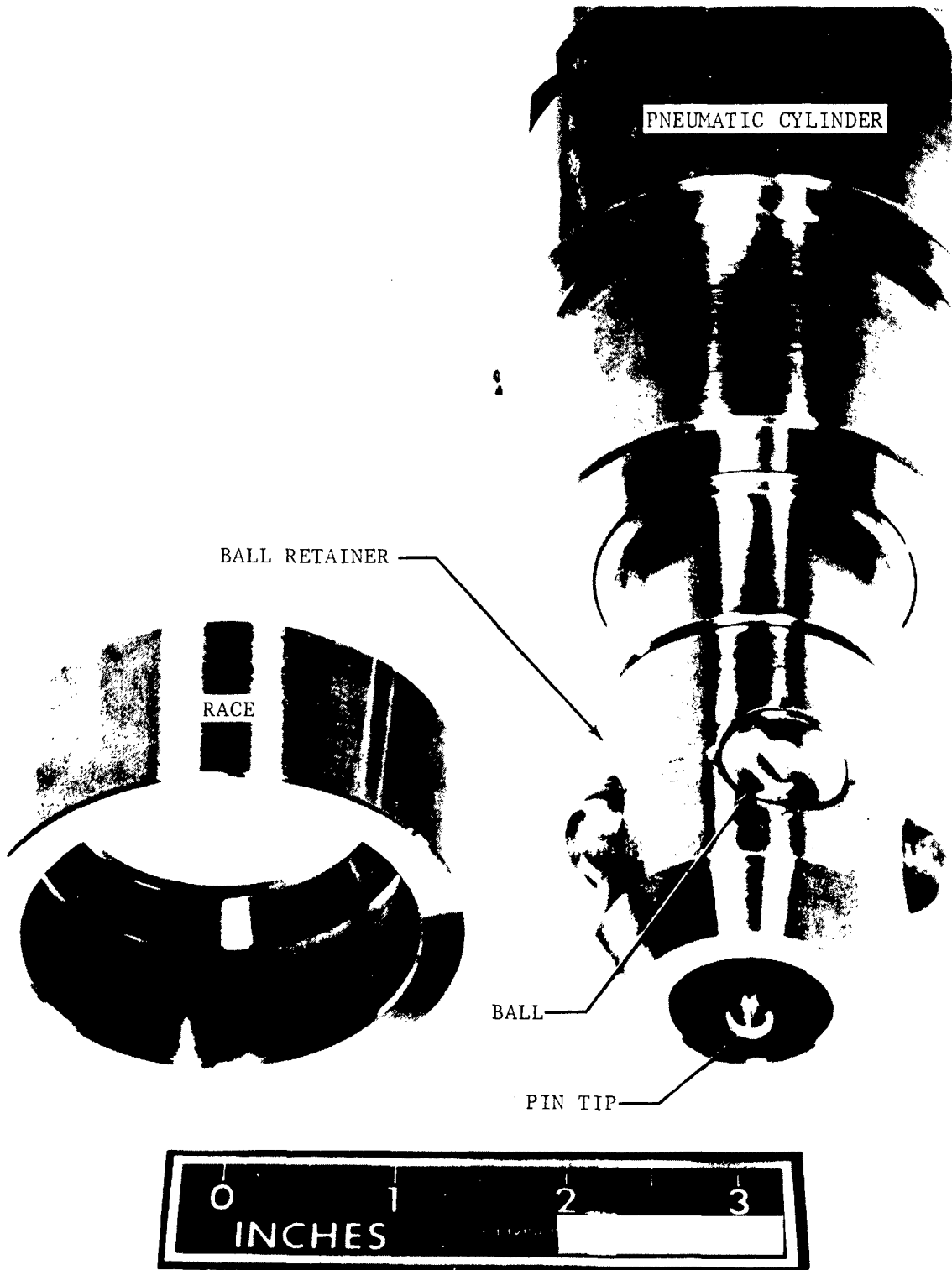
ILLUSTRATION 1. BALL-LOCK (2 INCH)
