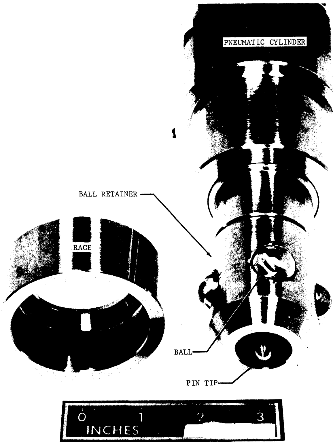
ILLUSTRATION 1. BALL-LOCK (2 INCH)
