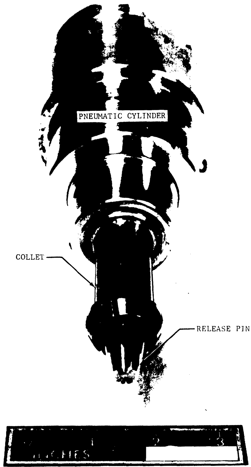
ILLUSTRATION 2. COLLET-LOCK (1 INCH)
