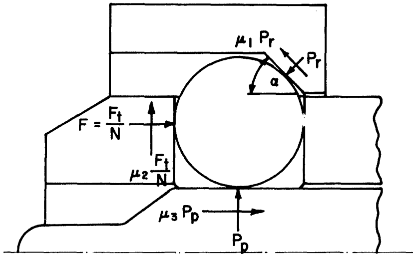
FORCE DIAGRAM
