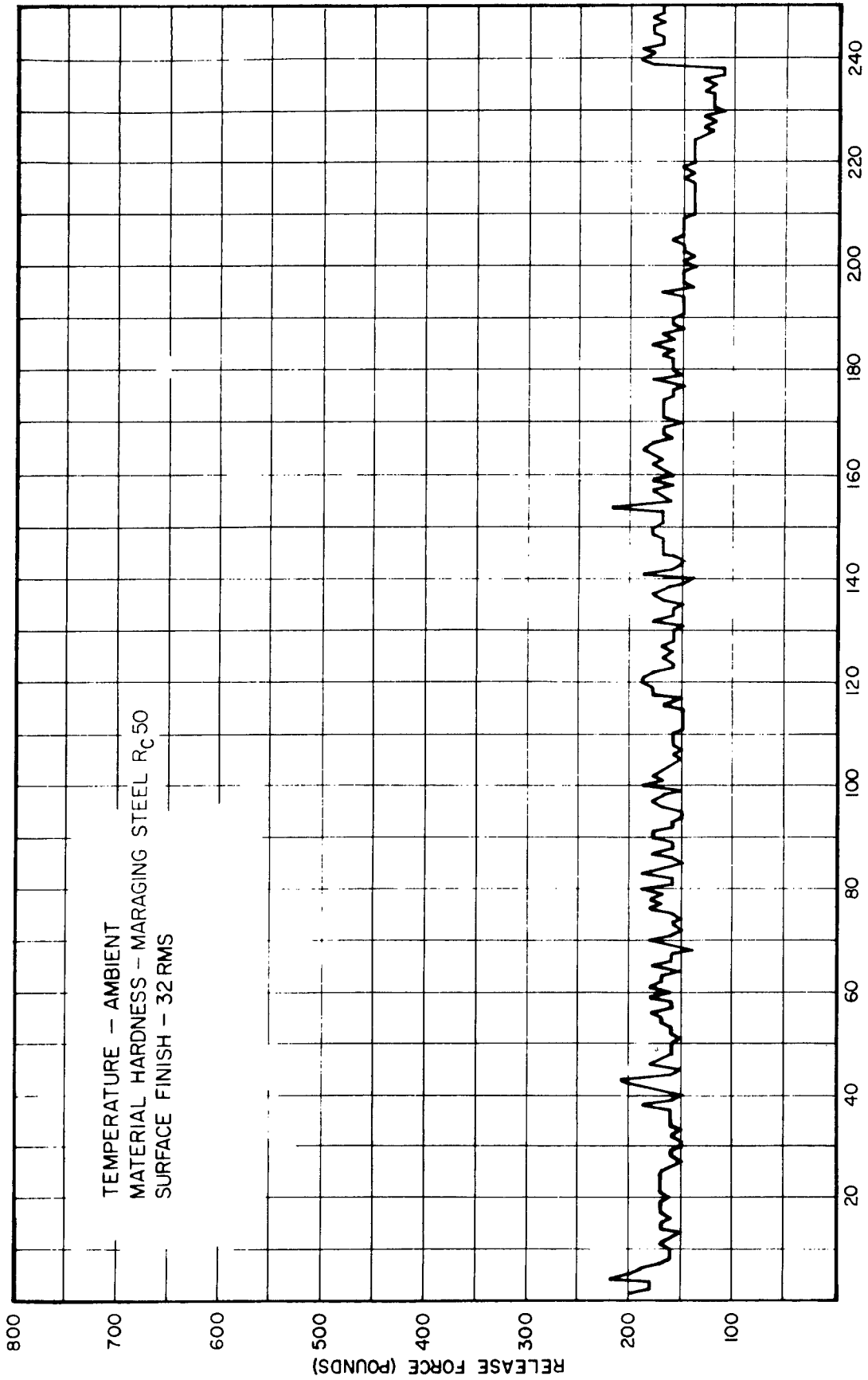
FIGURE 5, BALL-LOCK LIFE CYCLE INVESTIGATION
