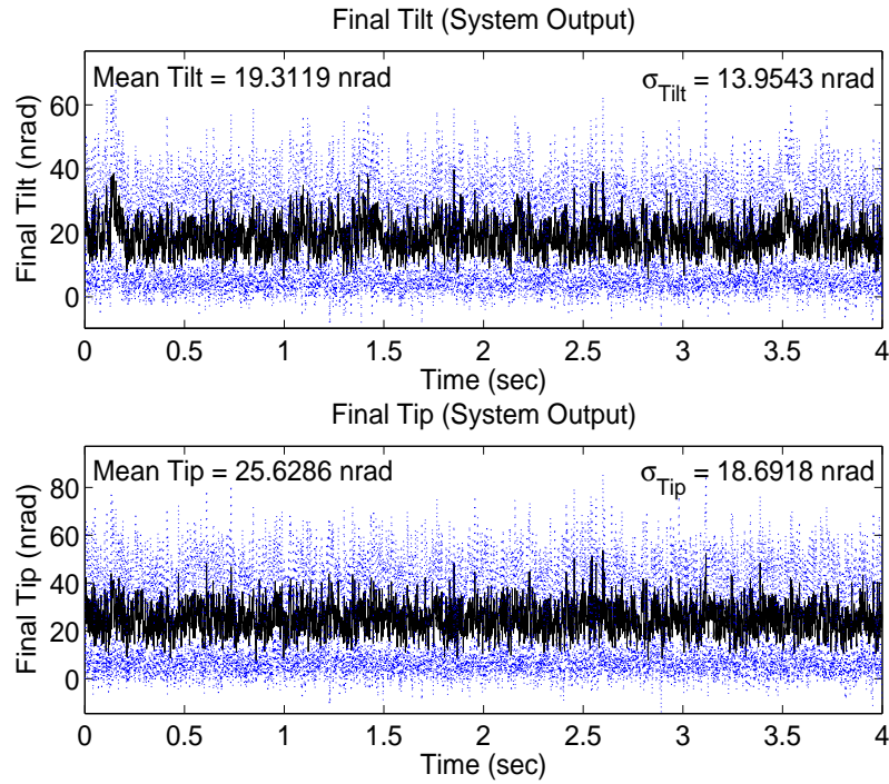
Figure 4.136 Case (23.5a): Delay 5, f_G = 86 Hz, \mathbf{U}_{diag} = [1 \ 1 \ 1E4 \ 1E4]
