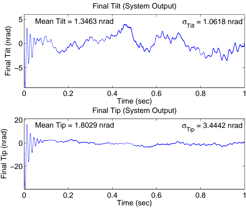
Figure 4.50 Case (7.5b): Delay 5, \mathbf{U}_{diag} = [5E3 \ 5E3 \ 1E4 \ 1E4]
