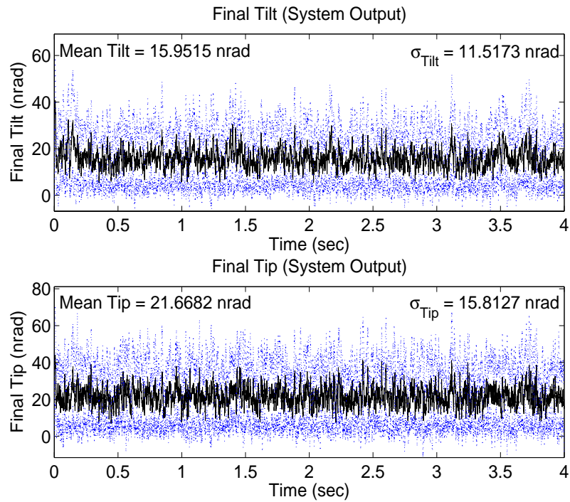
Figure 4.138 Case (23.5b): Delay 5, f_G = 86 \text{ Hz} , \mathbf{U}_{diag} = [5E3 \ 5E3 \ 1E4 \ 1E4]
