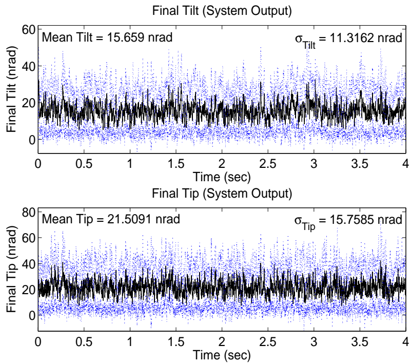
Figure 4.144 Case (24.5b): Delay 5, f_G = 189.2 Hz, \mathbf{U}_{diag} = [5E3 \ 5E3 \ 1E4 \ 1E4]
