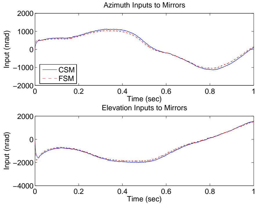
Figure 4.102 Case (16c): \mathbf{U}_{diag} = [1E4 \ 1E4 \ 1E4 \ 1E4]
