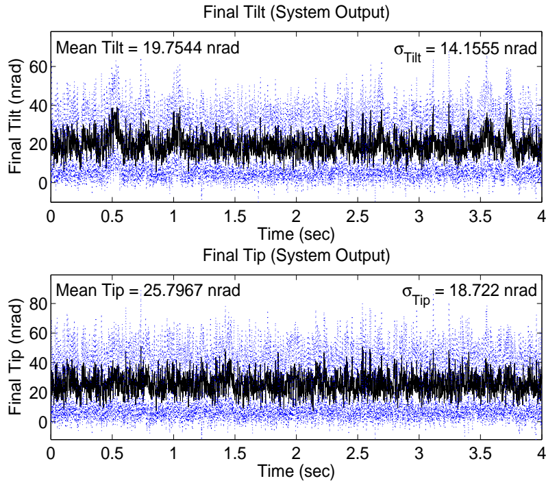
Figure 4.148 Case (25.5a): Delay 5, f_G = 43 \text{ Hz} , \mathbf{U}_{diag} = [1 \ 1 \ 1E4 \ 1E4]
