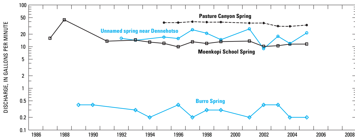
Figure 10. Discharge from selected springs, Black Mesa area, Arizona, 1987–2005. Data from earlier measurements at Moenkopi School Spring, unnamed spring near Dennehotso, and Pasture Canyon Spring are not shown because different measuring locations were used.
