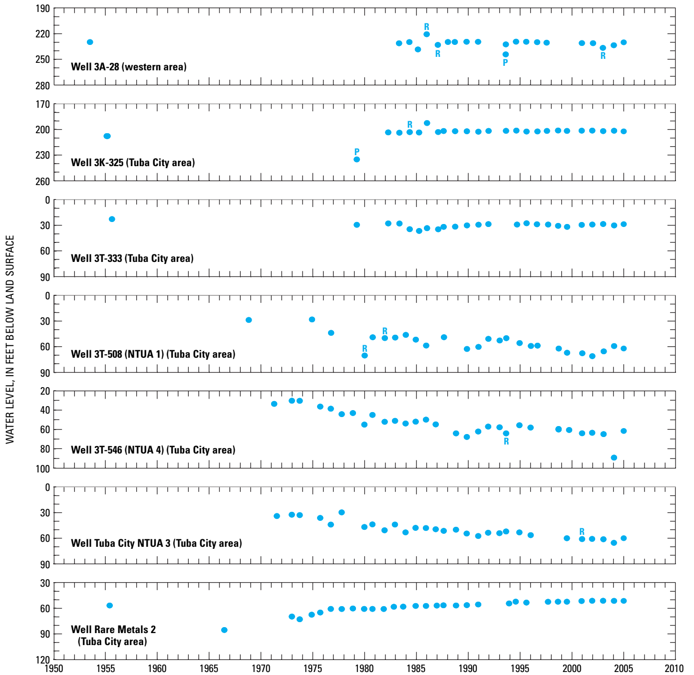
Figure 7. Observed water levels (1950–2005) in annual observation well network, Black Mesa area, Arizona. P, pumping; R, recently pumping.
