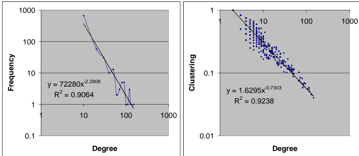
Figure 15: Properties of a scale-free network—degree distribution (left) and clustering coefficient 19 by degree (right)
