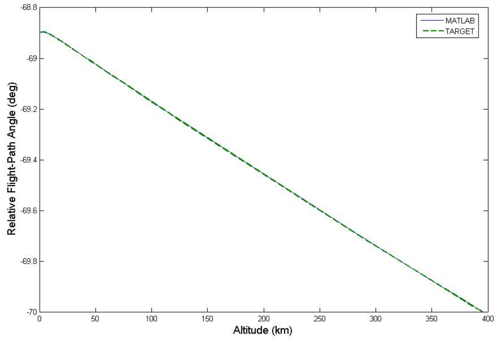
Figure 19. Flight-Path Angle/Altitude Comparison for MATLAB/TARGET Case #1
