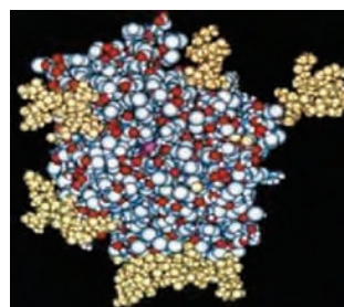
Molecular model of human plasma-derived butyryl
