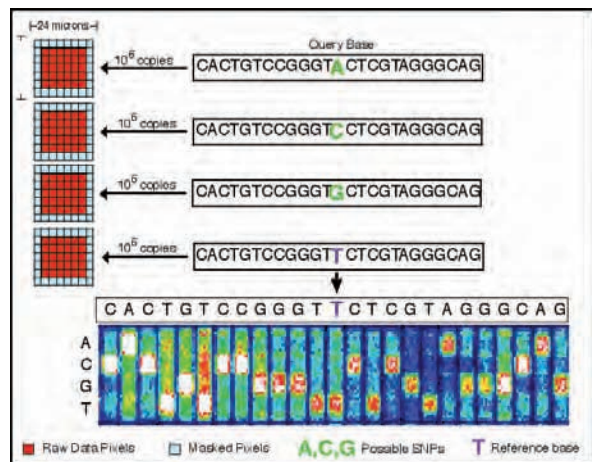
Affymetrix resequencing
