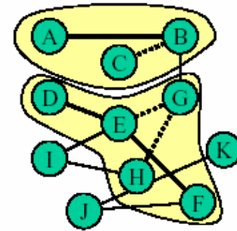
Graph Clustering
