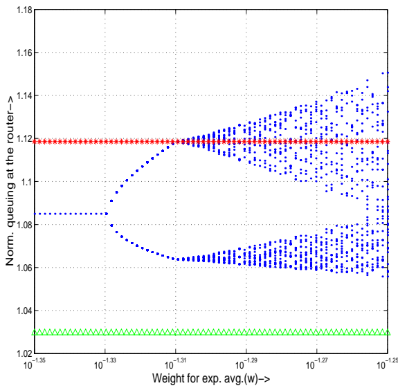
Fig. 5. Bifurcation diagram of average queue length w.r.t. w , p_{max} = 0.1
