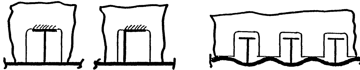
TYPE A - WELD ON TOP - DIFFICULT TO FIT DUE TO PLATE DISTORTION FROM STIFFENER WELDING
