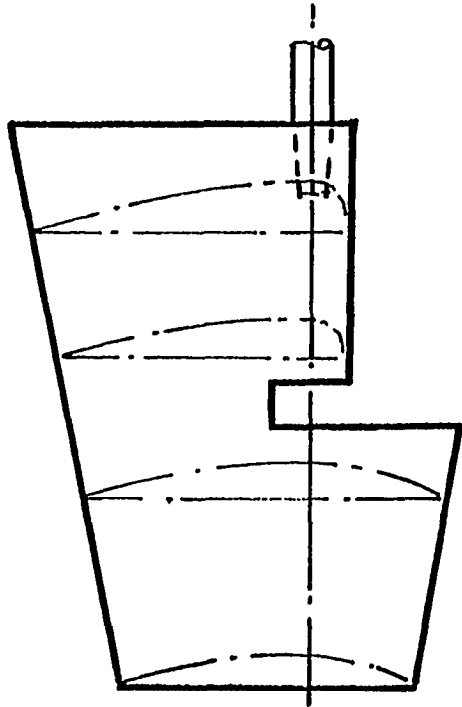
TRADITIONAL, RUDDER ON HORN
