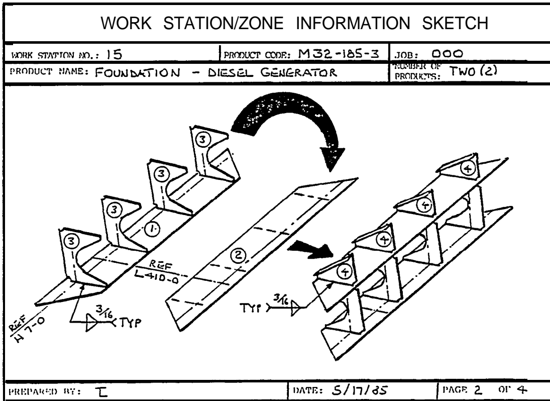
FIGURE 2.29 Hull fitting work station information.
