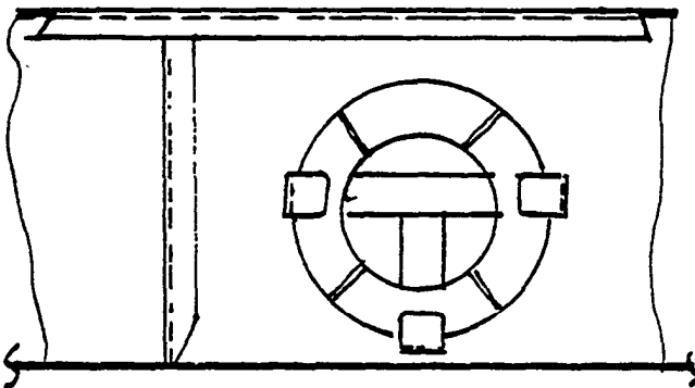
STANDARD LIFEBOUY STOWAGE ON BULWARK
