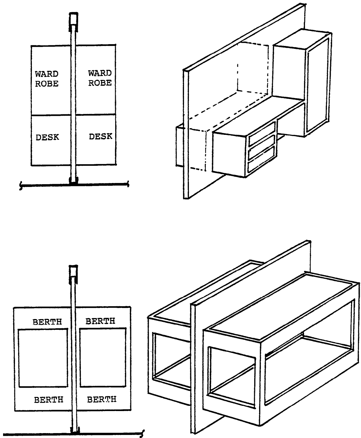
FIGURE 1.98 Common outfitted joiner bulkheads.
