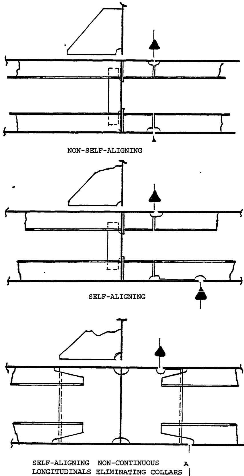
FIGURE 1.45 Longitudinal joining details.
