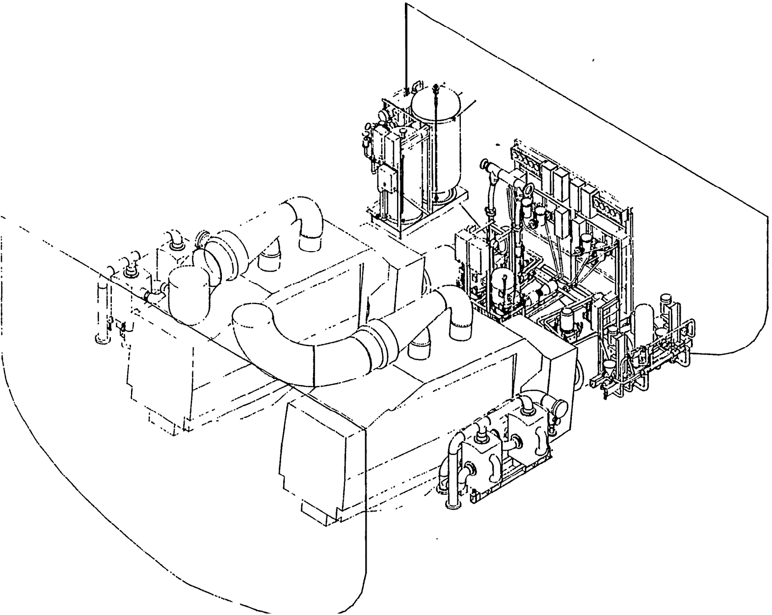
FIGURE 2.21 CAD-prepared isometric zone design arrangement.
