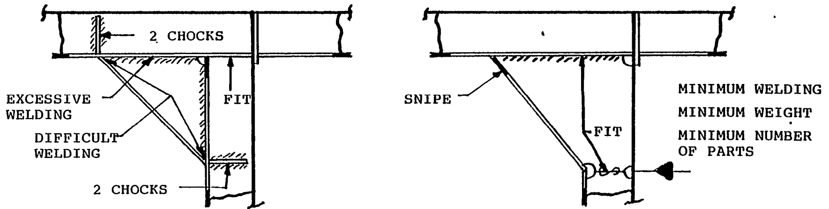
[B] - LONGITUDINAL/STIFFENER DETAIL
