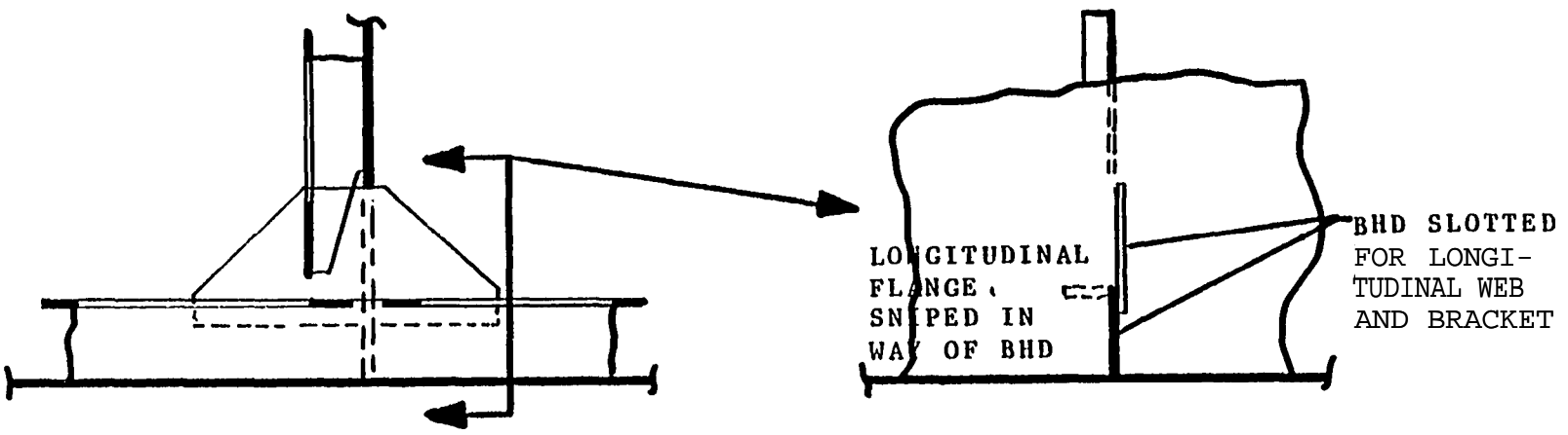
ALTERNATIVE WHEN LONGITUDINALS ARE TO BE CONTINUOUS
