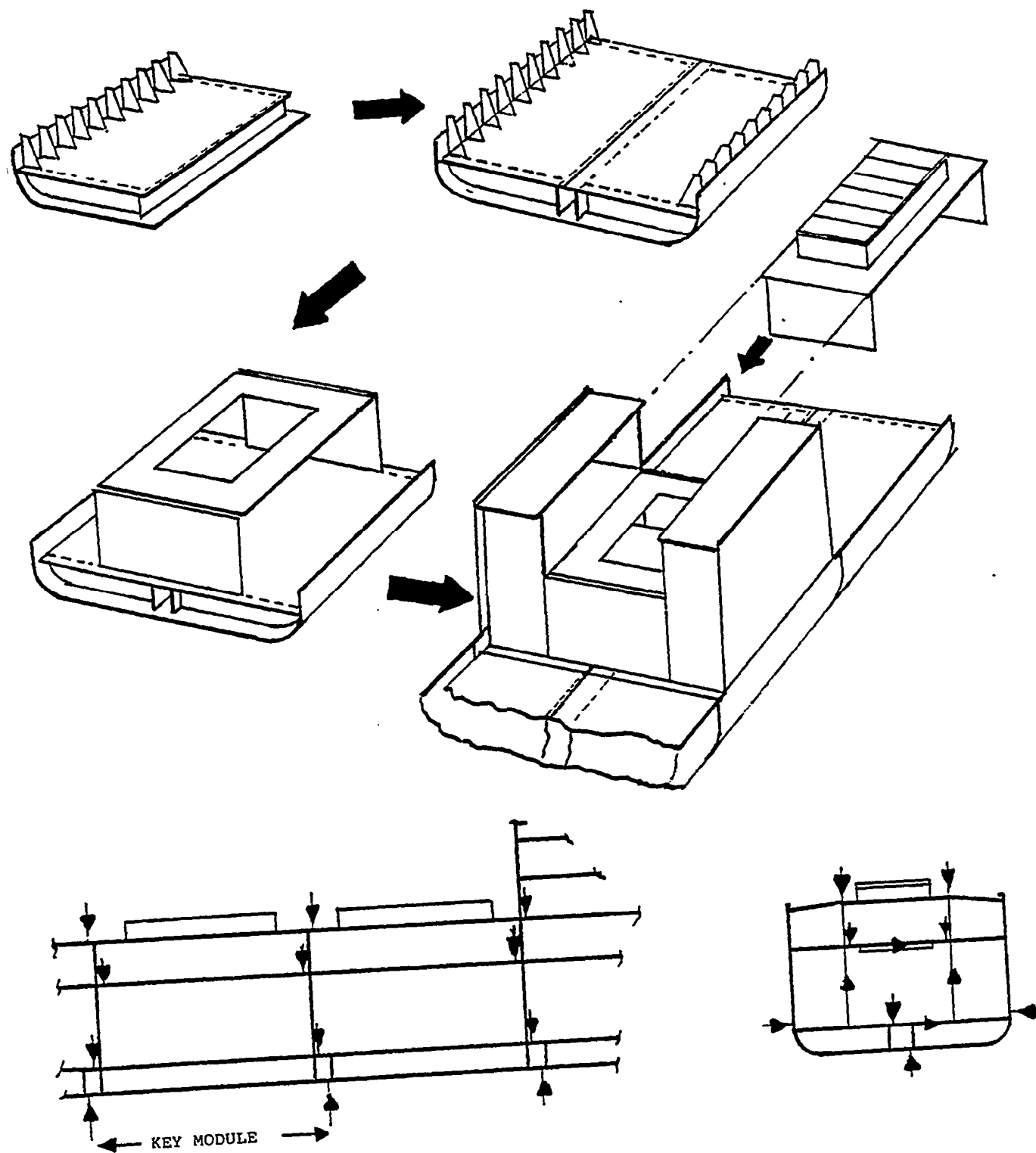
FIGURE 1.52 Cargo ship modules.
