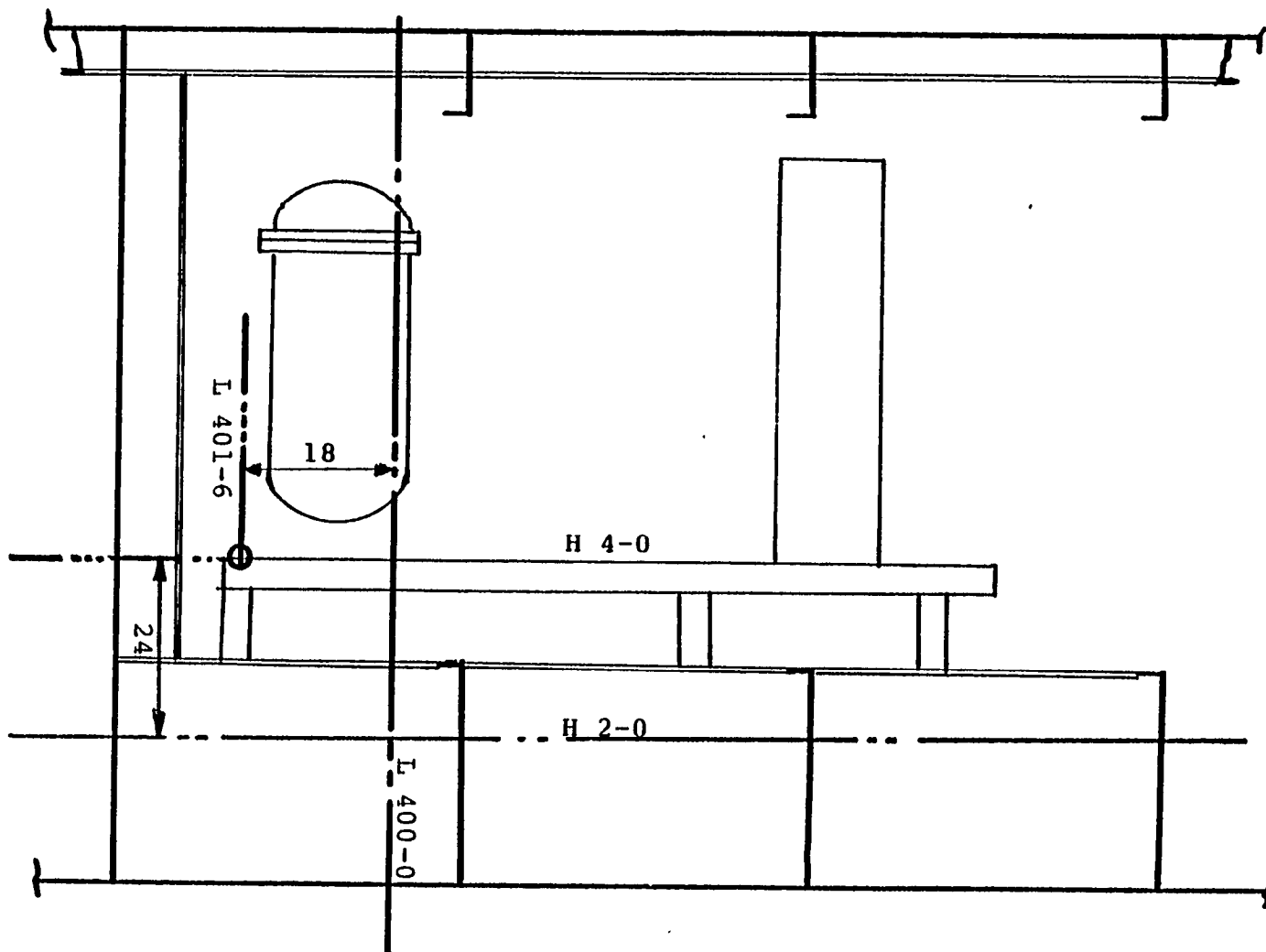
FIGURE 1.32(b) Relation of secondary reference system to primary reference system.
