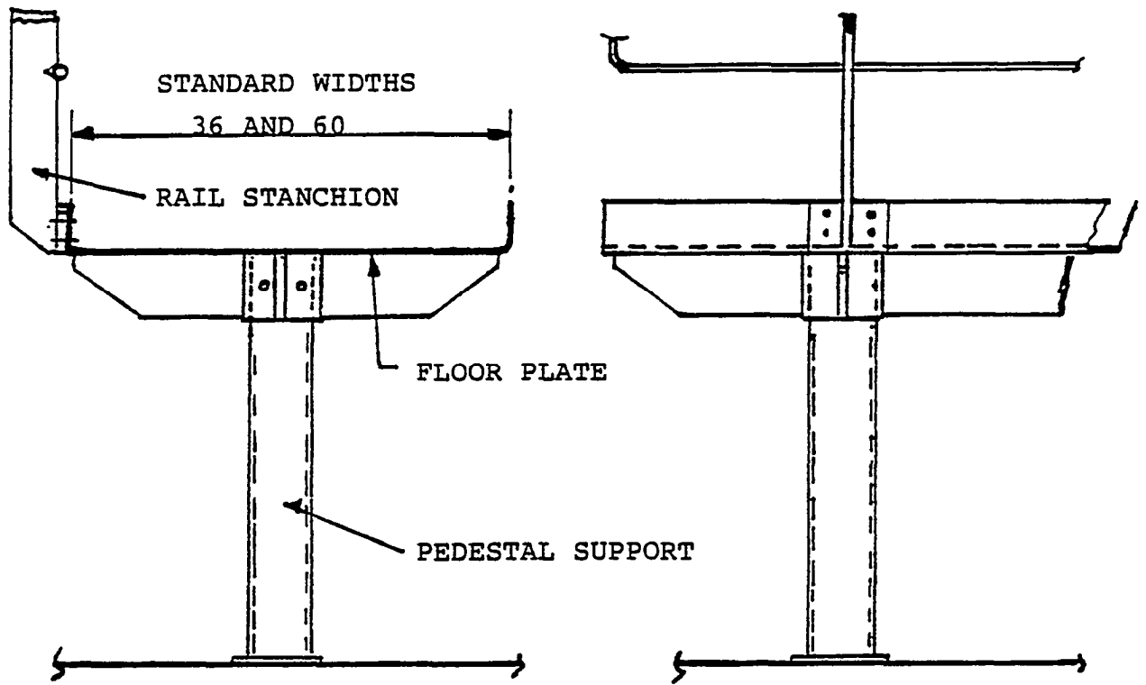
[A] BASIC COMPONENTS OF STANDARD FLOOR PLATE
