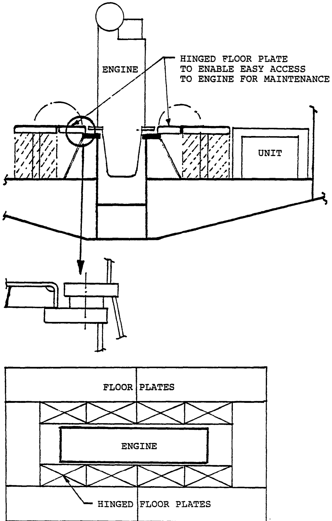
FIGURE 1.102 Hinged floor plates adjacent to engine.
