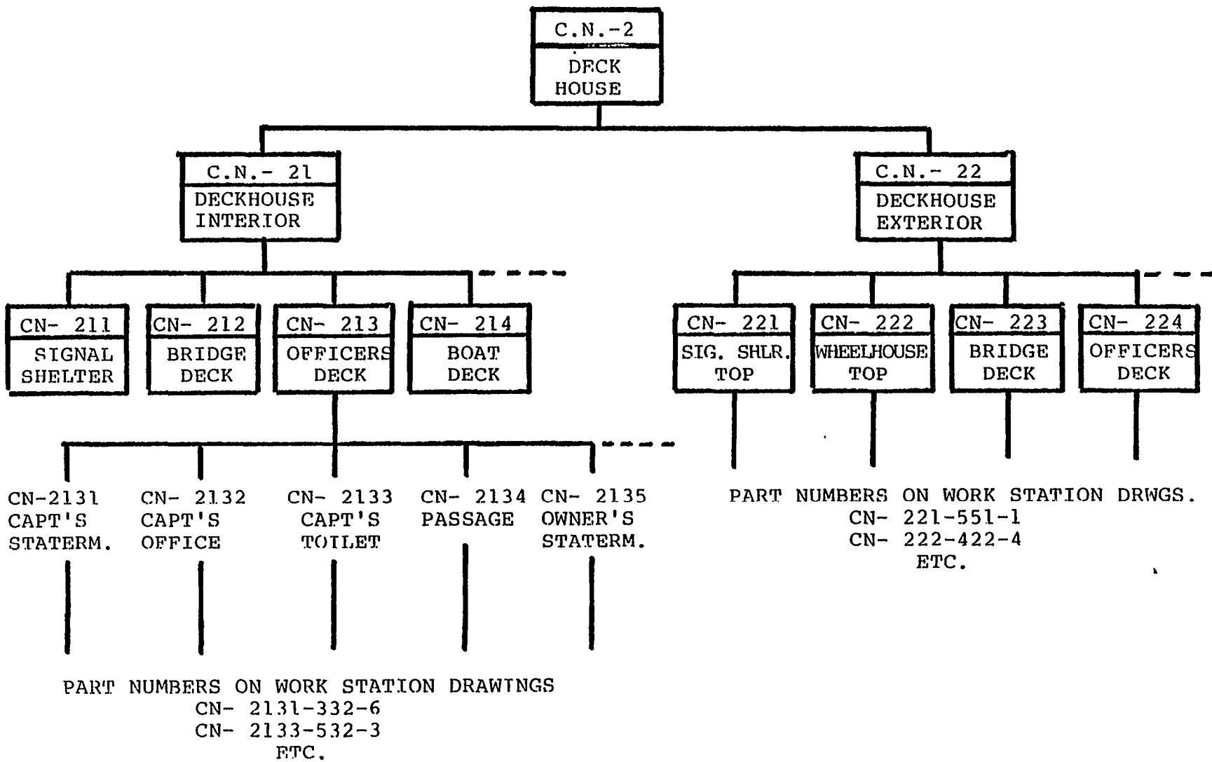
FIGURE 2.18 (Continued)-Deckhouse zone breakdown.
