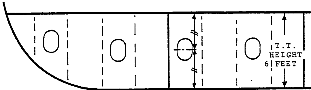
CENTERED ACCESS HOLES - DIFFICULT ACCESS
