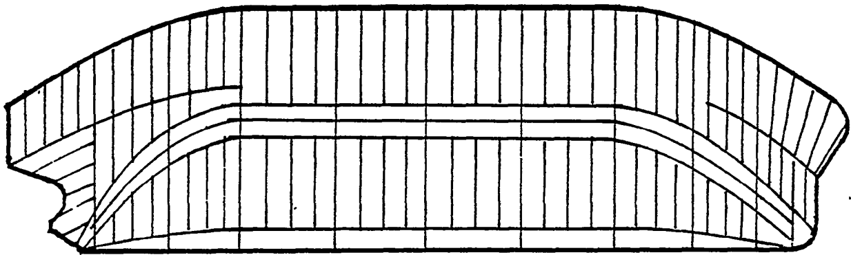
VERTICALLY STRAKED SHELL
