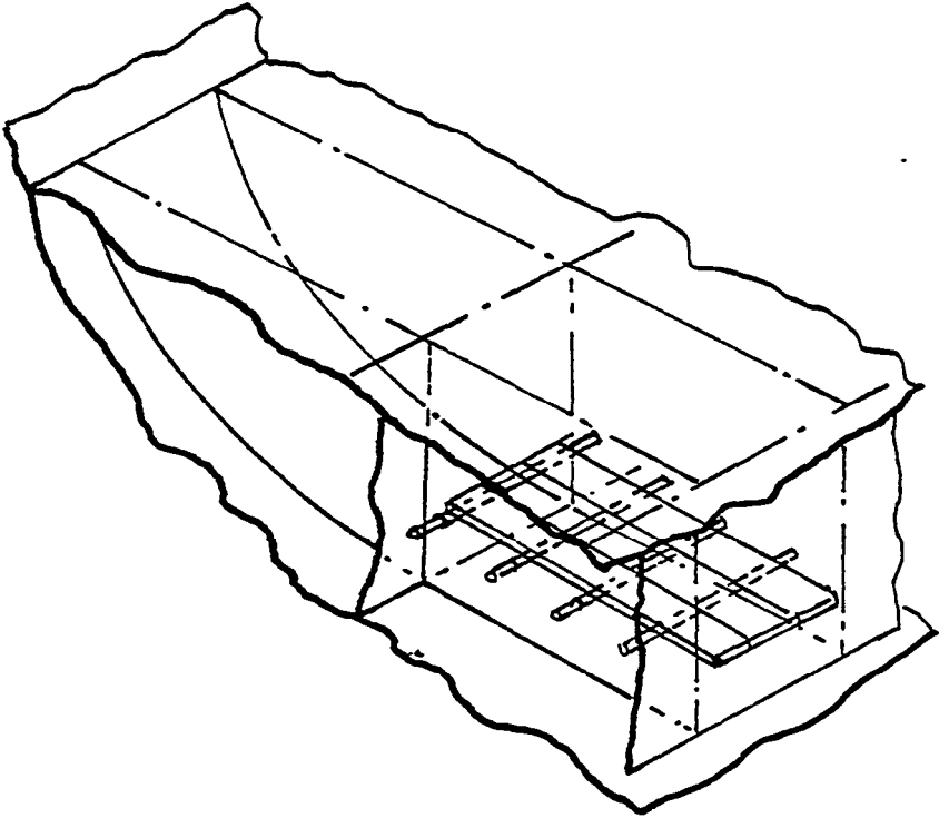
FIGURE 1.69(a) Built-in staging aids in D.B.
