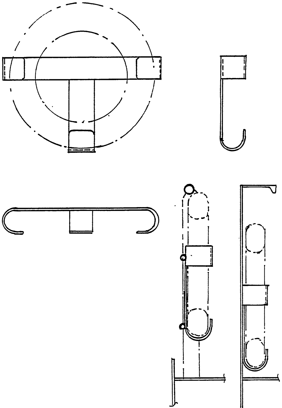
FIGURE 1.83(b) Details for standard lifebuoy stowage.
