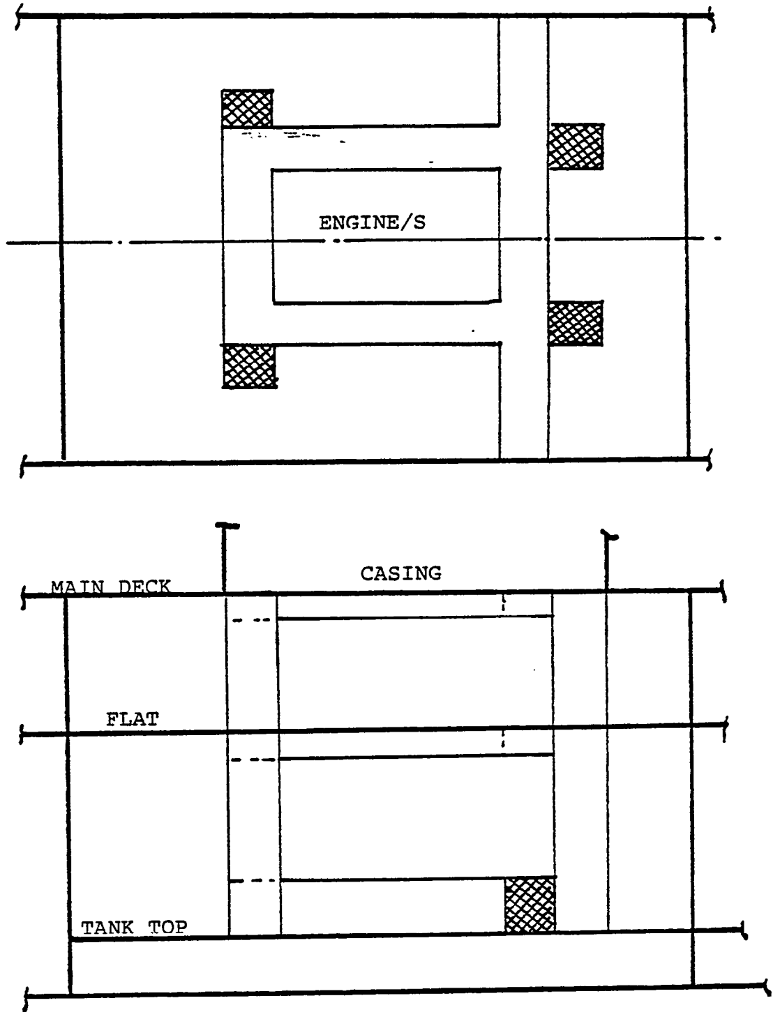
FIGURE 1.110 Standard machinery space system corridors.
