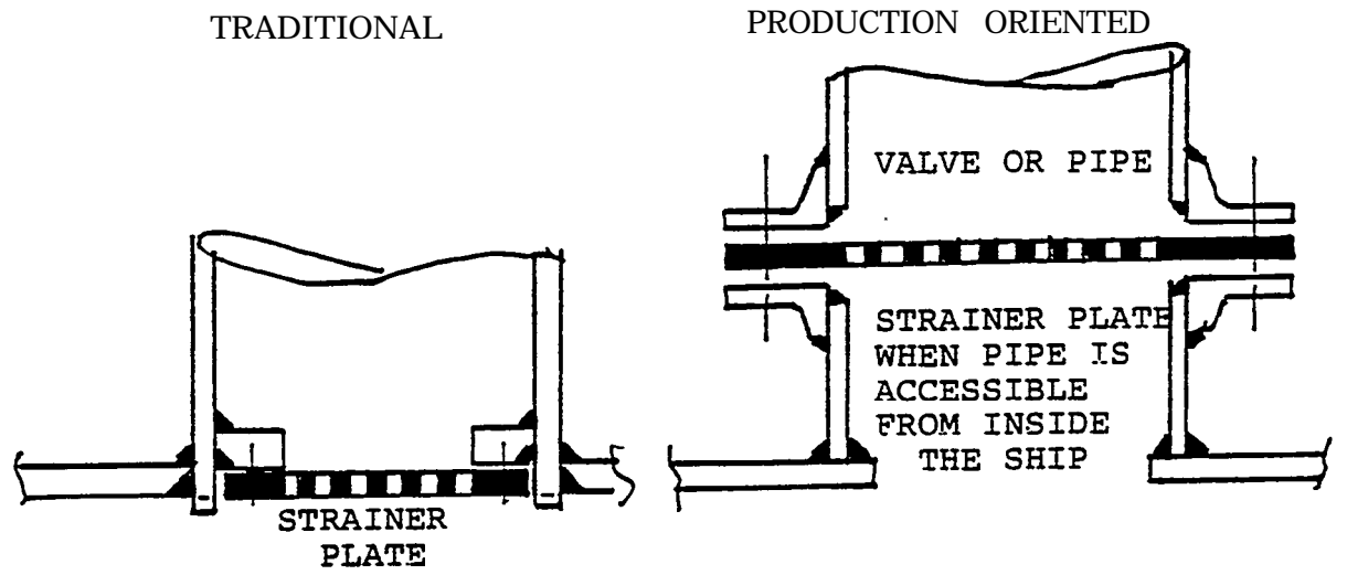
[A] PIPE/SHELL CONNECTION
