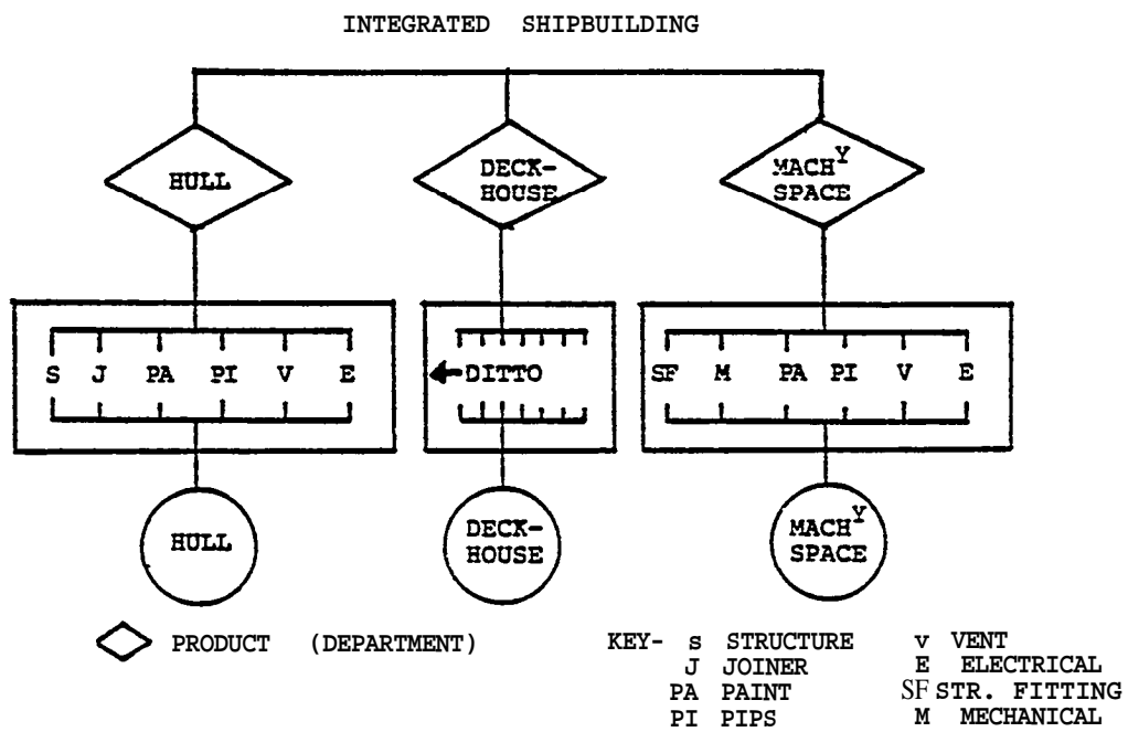
FIGURE 3.11 Suggested zone construction organization.
