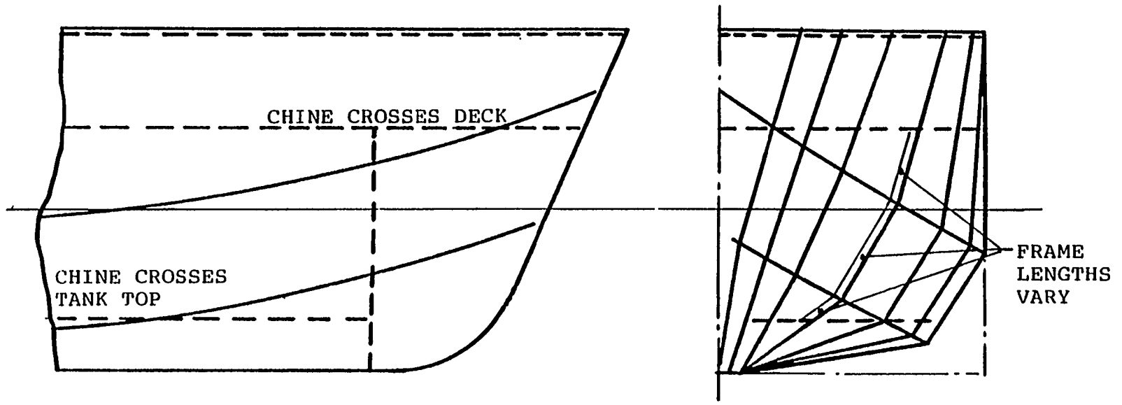
[A] TRADITIONAL CHINE FORM
