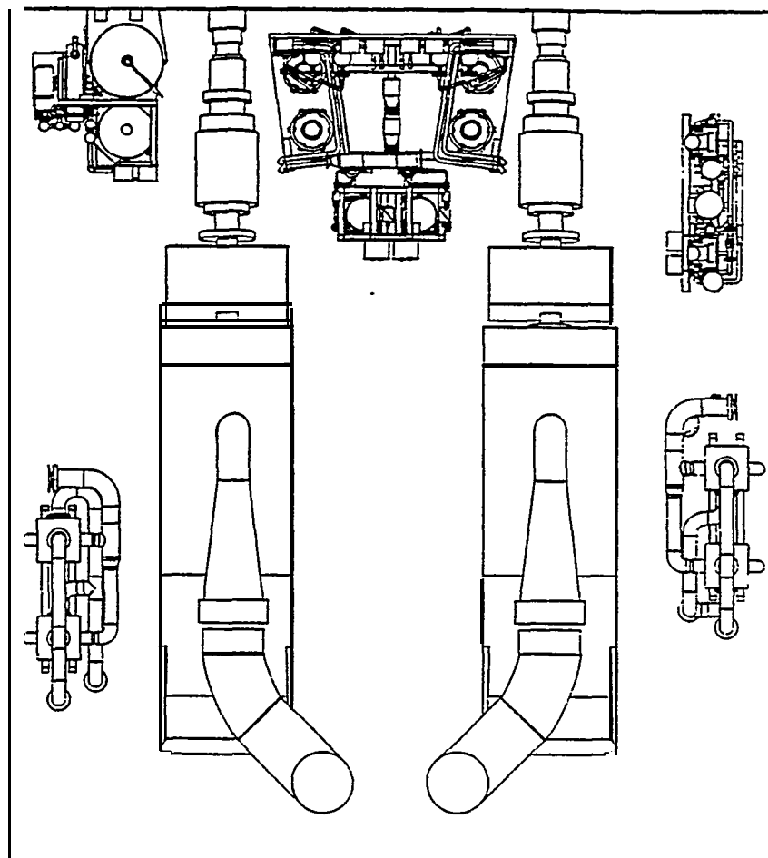
FIGURE 2.20 Manually prepared zone design arrangement.
