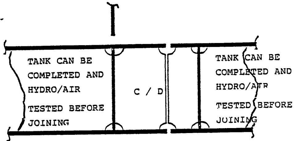
LOW WORK CONTENT NON-SELF-ALIGNING DESIGN
