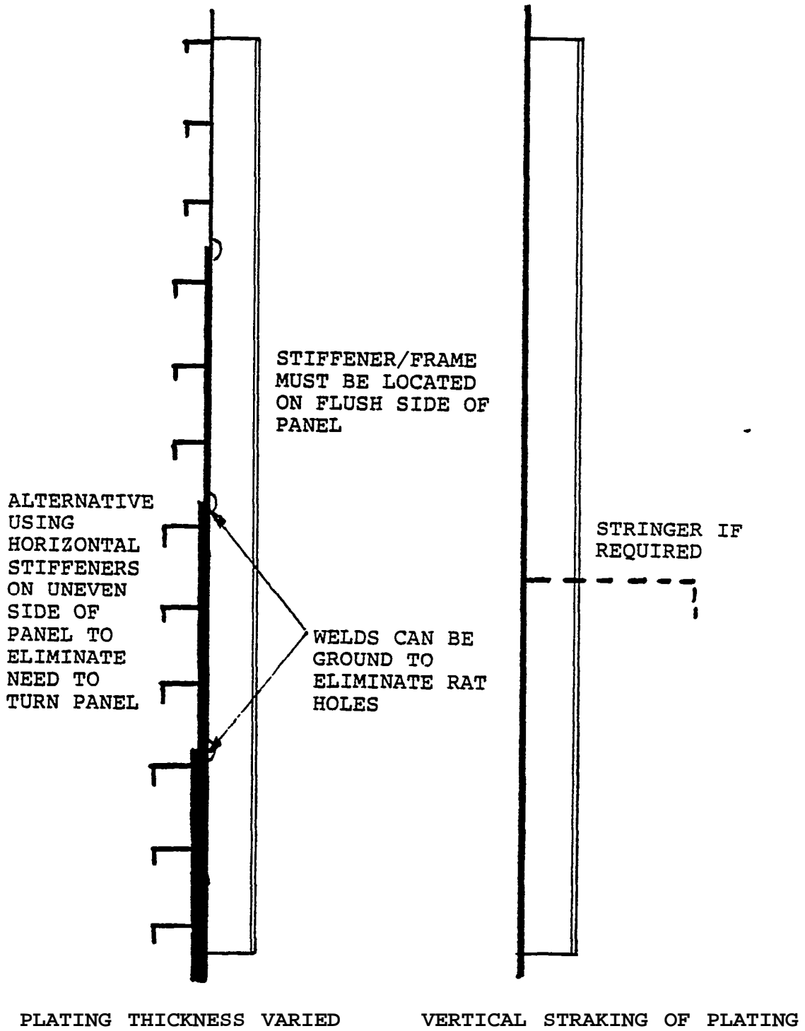
FIGURE 1.50 Plate straking/stiffener arrangements for productivity.
