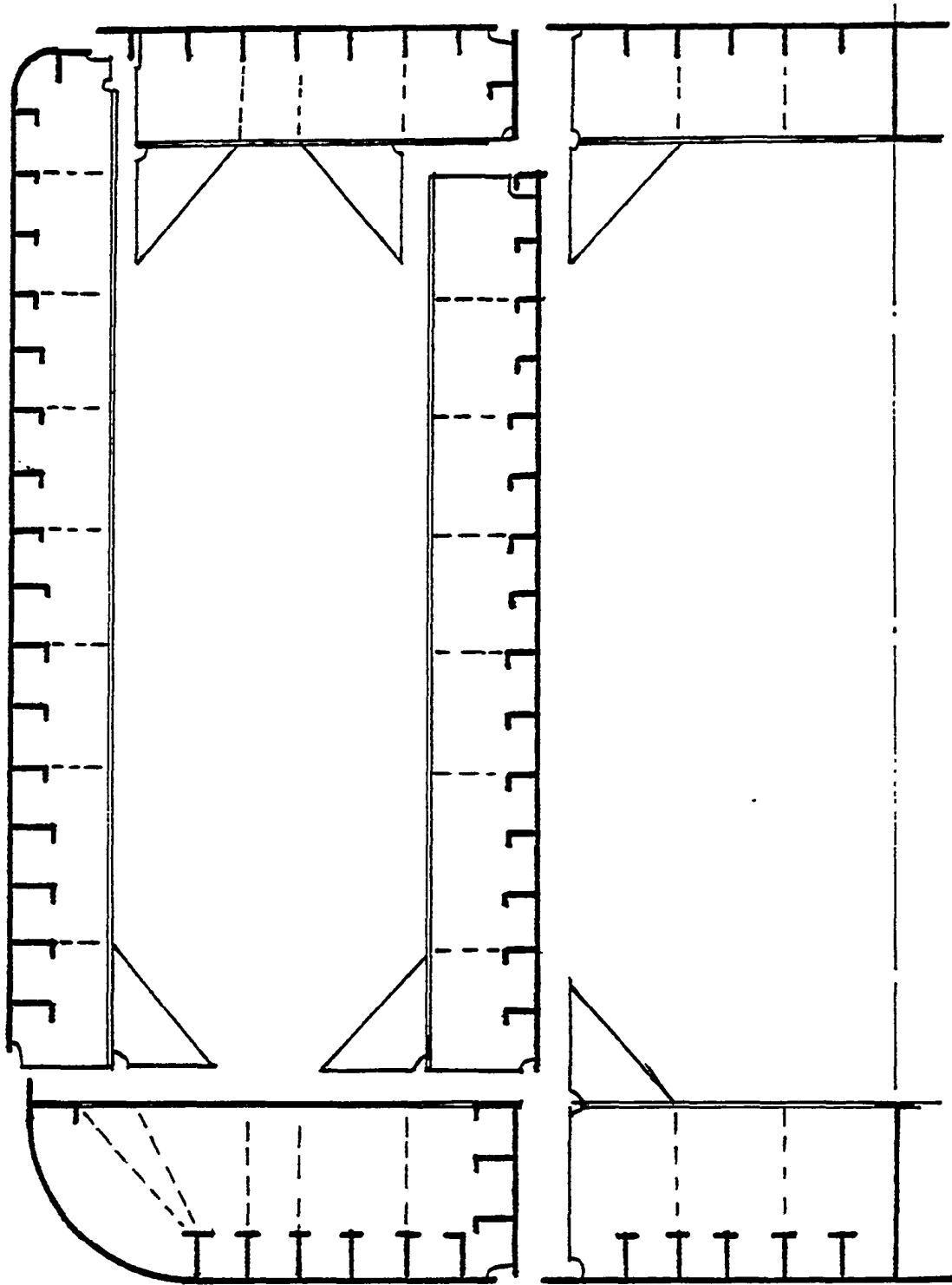
FIGURE 1.55(b) Tanker modules for "layer" method.
