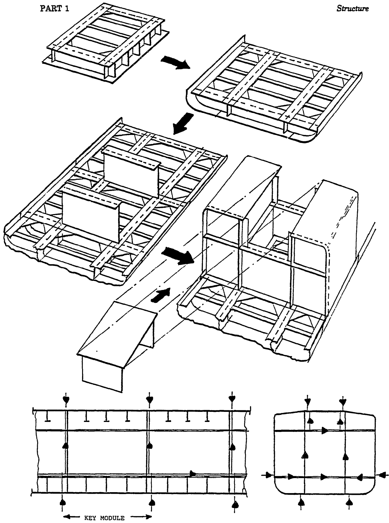
FIGURE 1.53 Tanker "layer" system modules.
