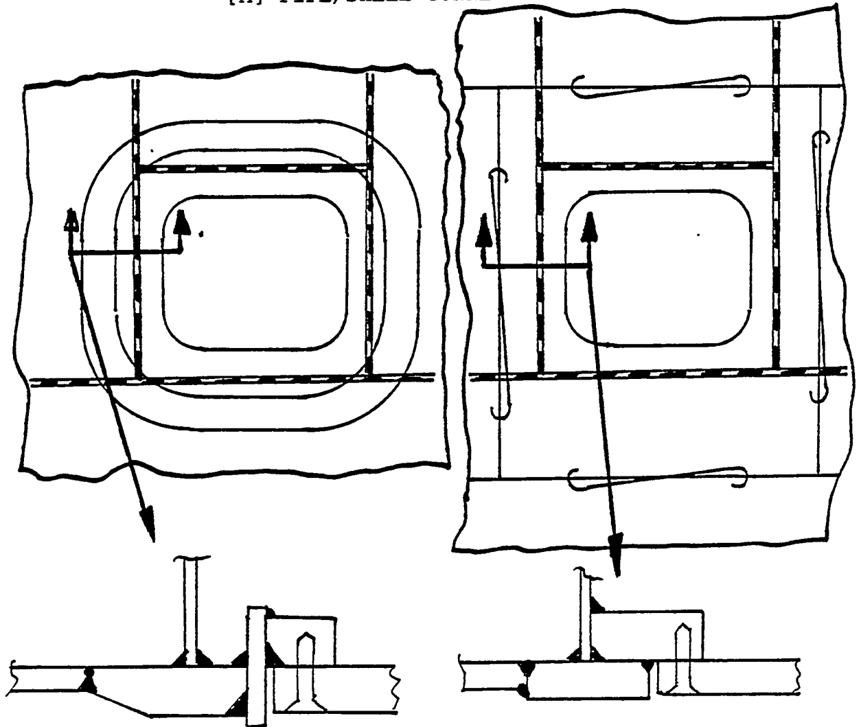
[A] PIPE/SHELL CONNECTION
