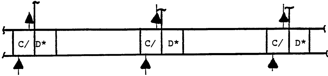
ELEVATION OF DOUBLE BOTTOM
