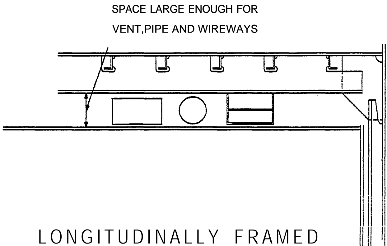
FIGURE 1.12 Required space above ceiling for services.
