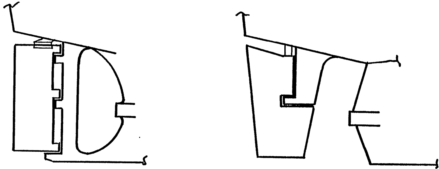
CLOSED APERTURE WITH STERN POST
