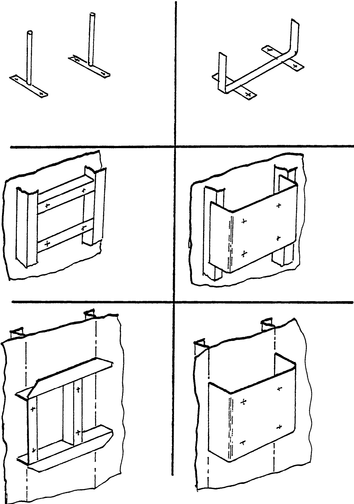
FIGURE 1.124 Electrical foundation design for production.
