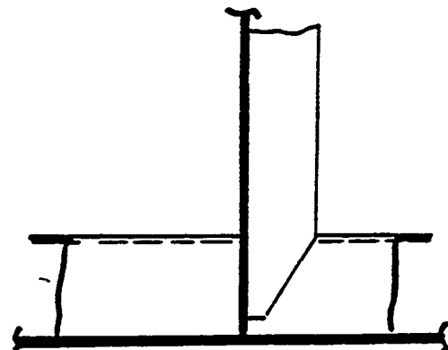
[C] ANGLE OPEN CUT-OUT WITH UNATTACHED STIFFENER
