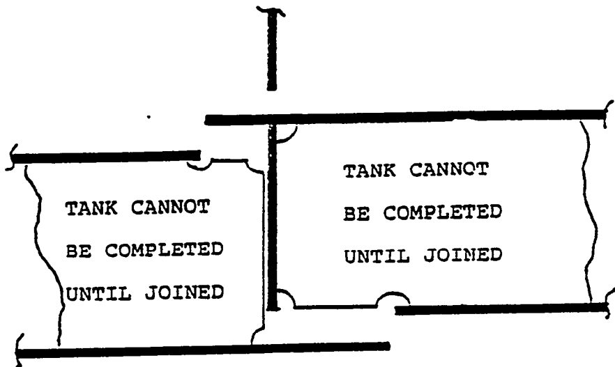
TRADITIONAL DESIGN - HIGH WORK CONTENT
