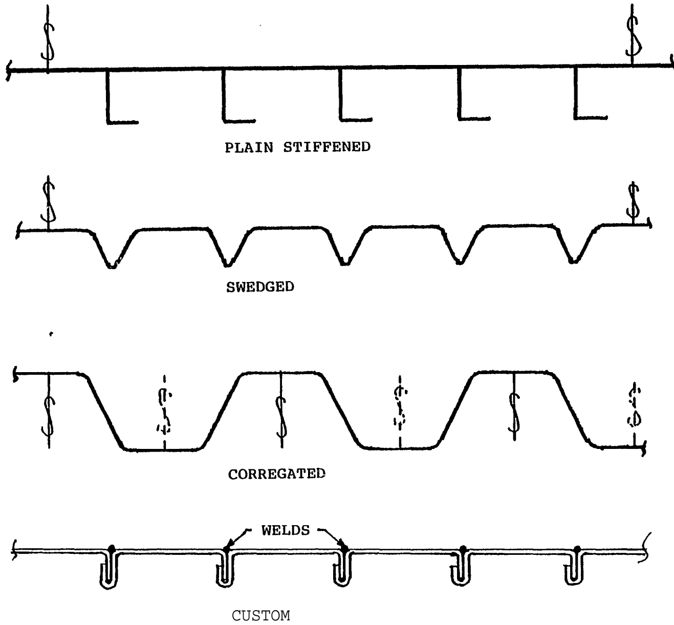
FIGURE 1.74 Alternative panel stiffening systems.
