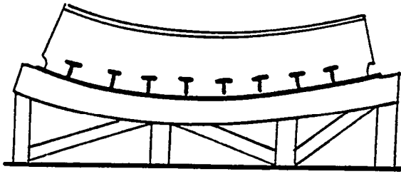
PLATE JIG
