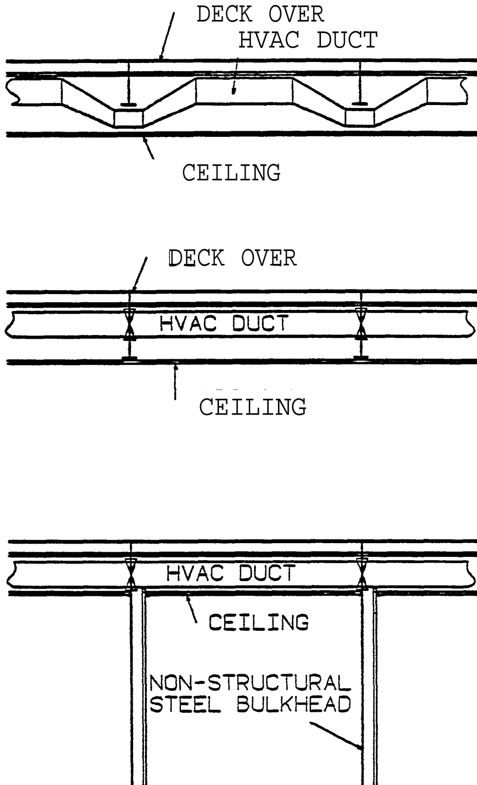
FIGURE 1.13 Alternative overhead deck space use.
