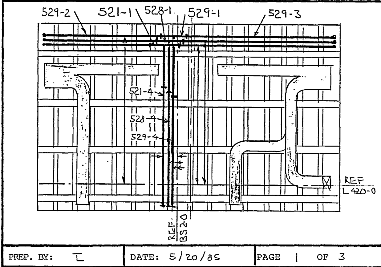
FIGURE 2.39 "On-block" advanced outfitting installation work station information for pipe.
