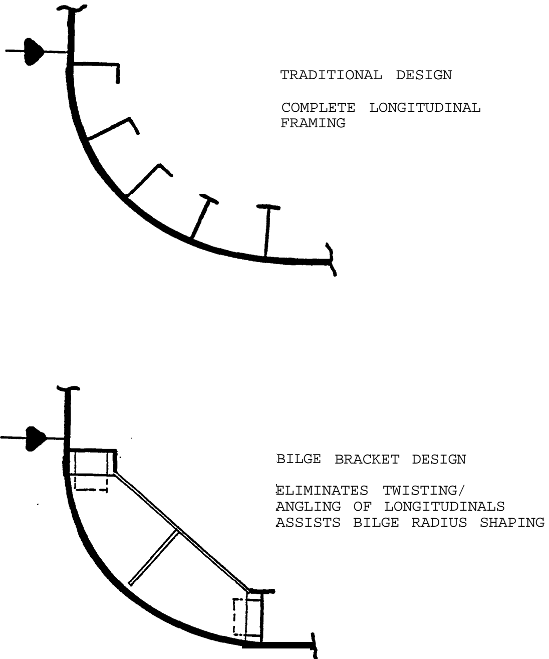
FIGURE 1.72 Bilge framing alternatives.
