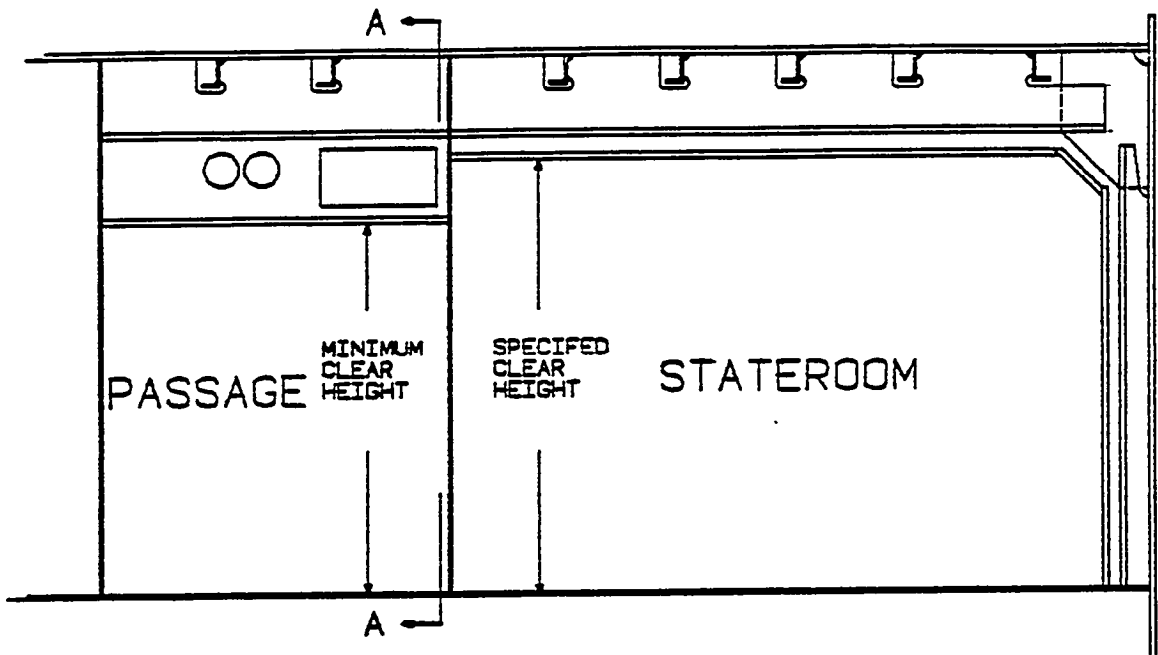
TRANSVERSE SECTION THROUGH ACCOMMODATION
