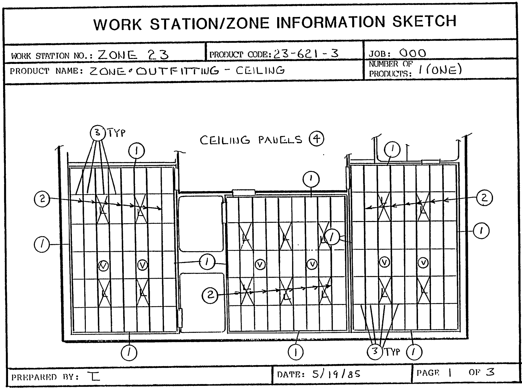
FIGURE 2.52 Deckhouse zone information for joiner ceiling installation.
