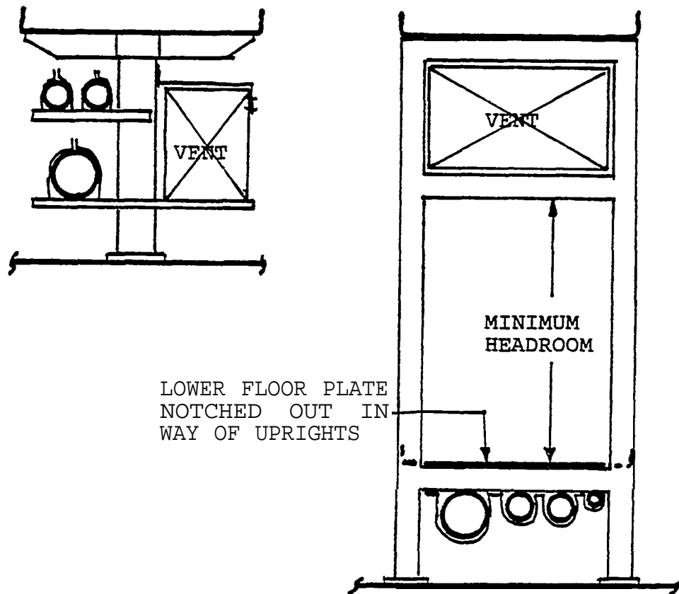
[B] COMBINED FLOOR PLATE/GRATING/SYSTEMS SUPPORT
