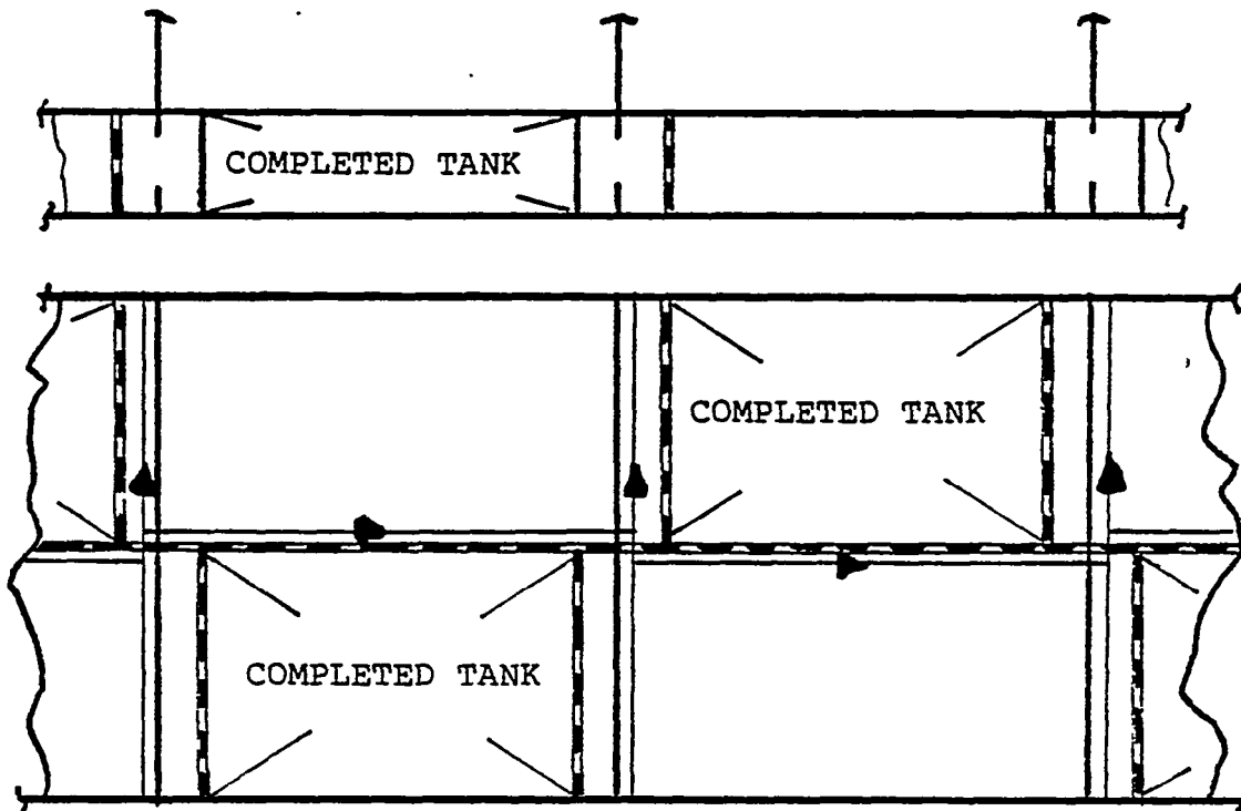
FIGURE 1.48 Alternative arrangement of module joints to facilitate tank completion including alternate tank testing.
