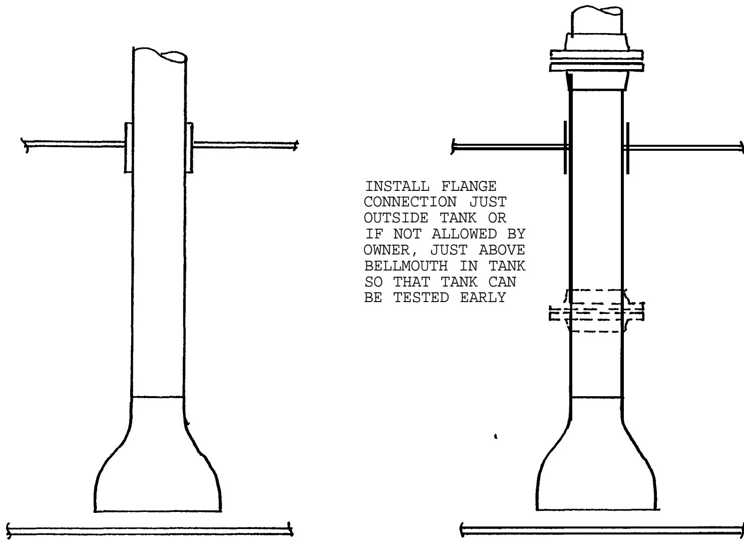
FIGURE 1.114 Piping passing through tank tops.
