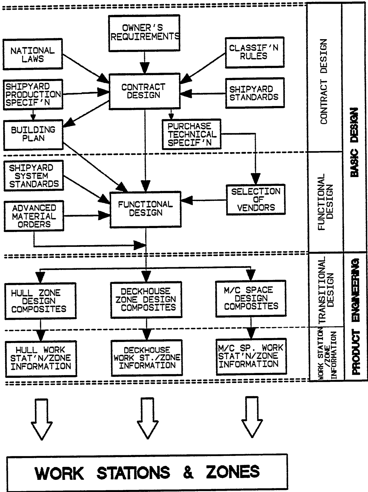
FIGURE 2.3 Flow of design and engineering information.
