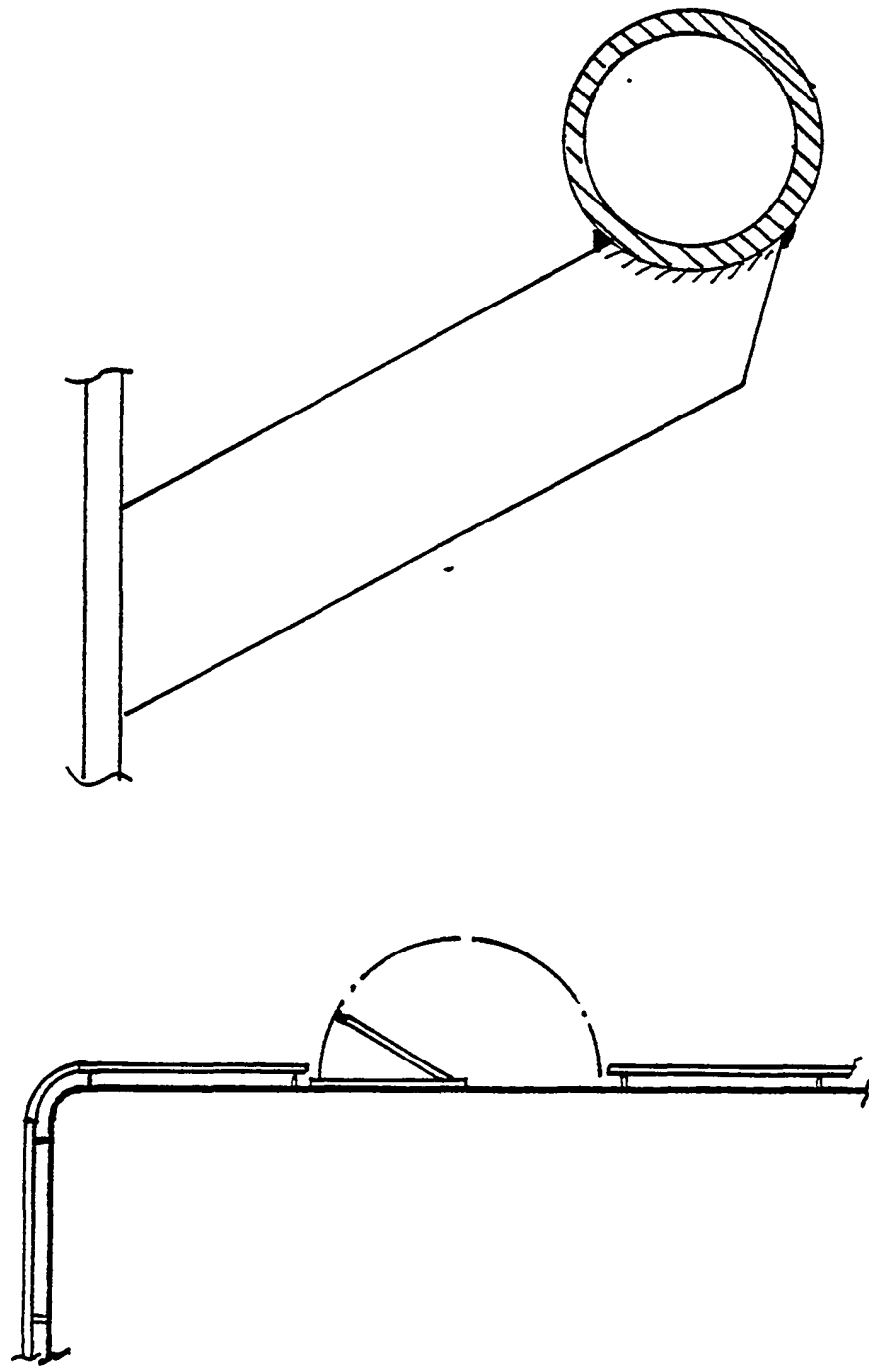
FIGURE 1.84 Standard handrail detail.
