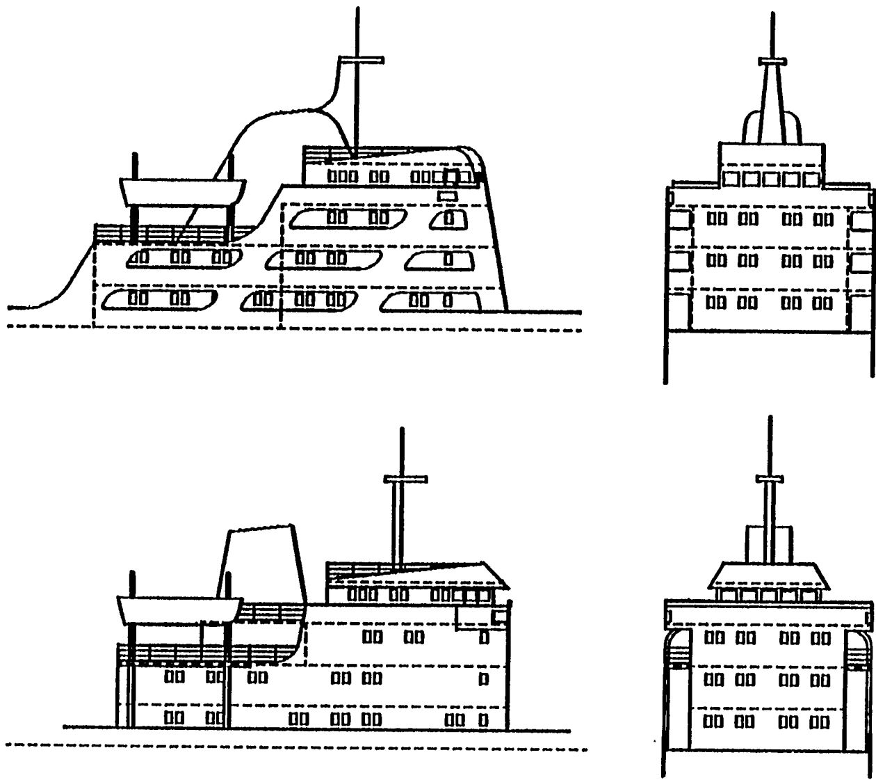
FIGURE 1.16 Aesthetic and cost-effective deckhouses.
