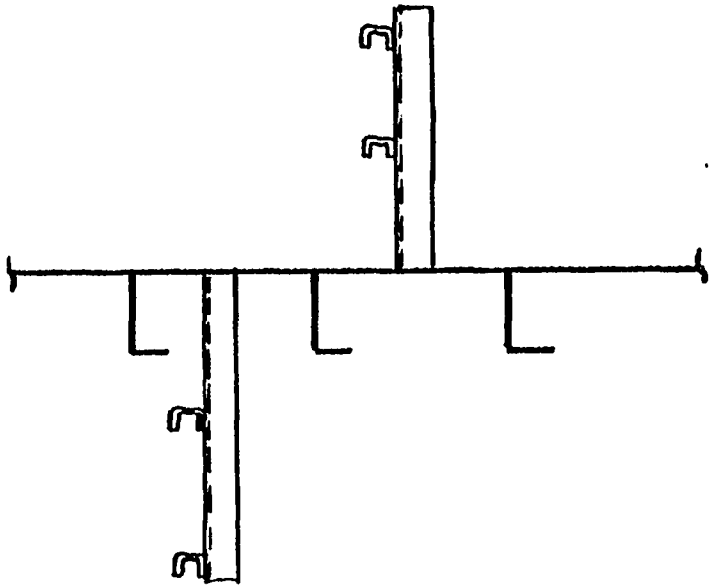
TYPICAL BAD PRACTICE - NOT PERMITTED ON SHELL OR MAIN DECK PLATING
