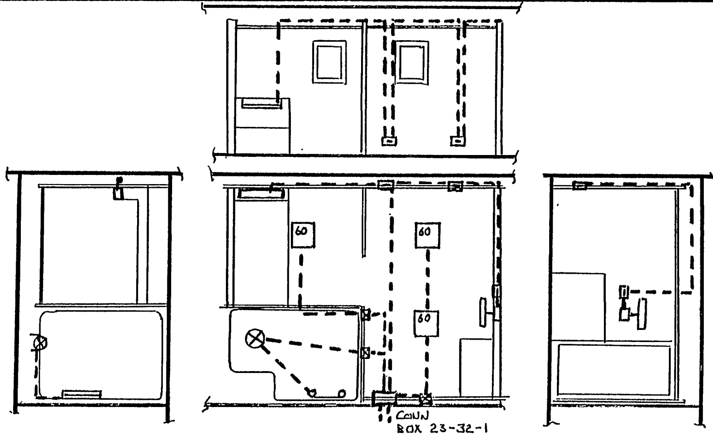
FIGURE 2.44 Zone information for electrical cable connecting.
