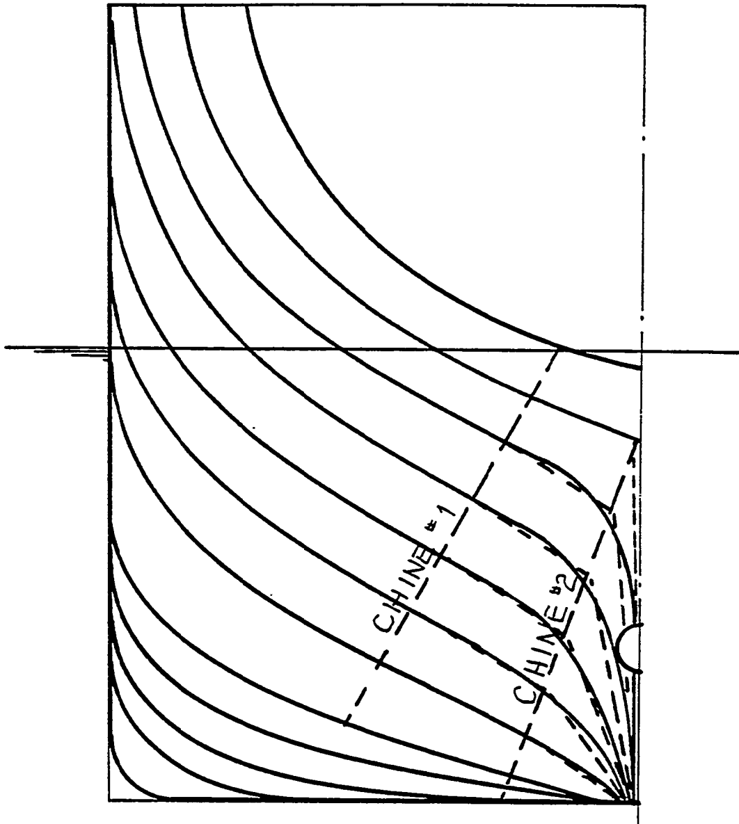
FIGURE 1.26 Use of chines to simplify stern construction.
