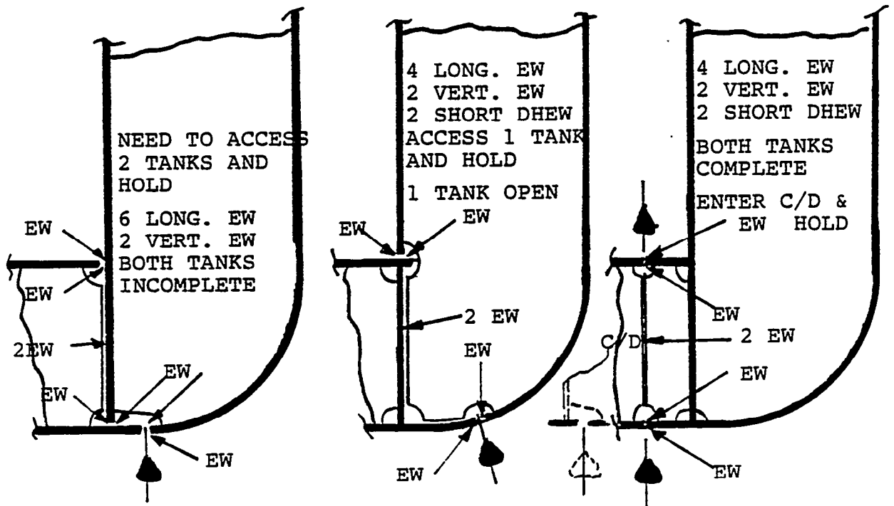
Figure 1.49 Module joining structural detail.
