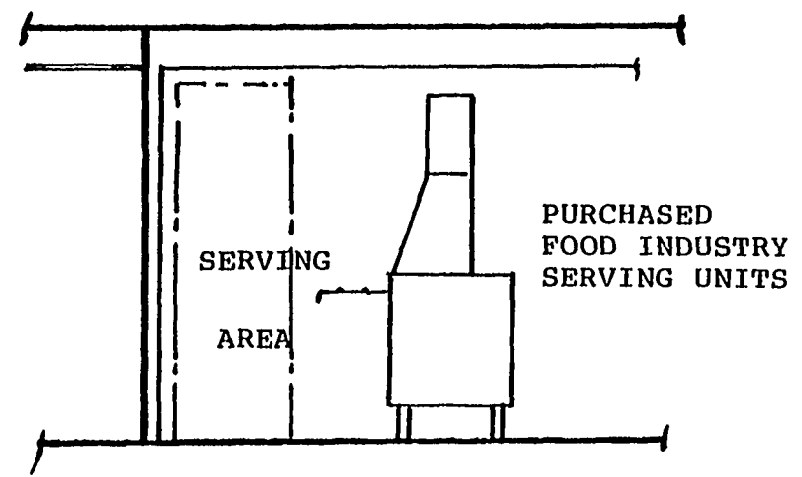
FIGURE 1.99 Galley arrangement for productivity.
