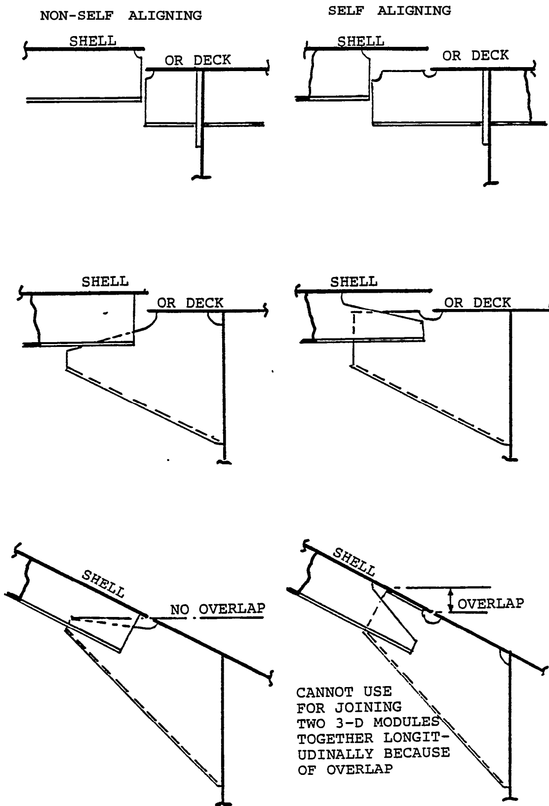
FIGURE 1.44 Module joining structural details.
