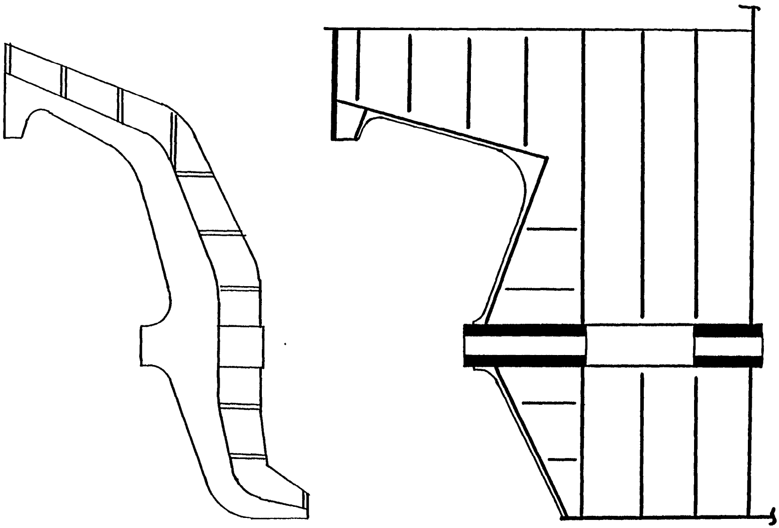
CAST STERN FRAME COMPOUND CURVES NECESSITATED CASTING
