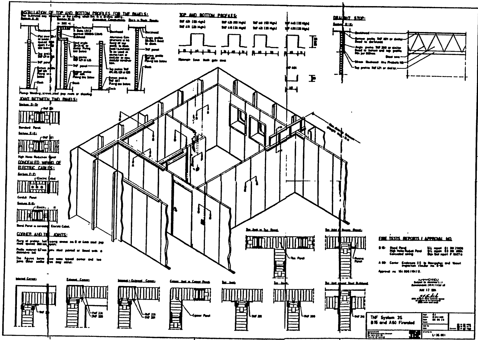
FIGURE 1.95 TNF joiner bulkhead and lining system.
