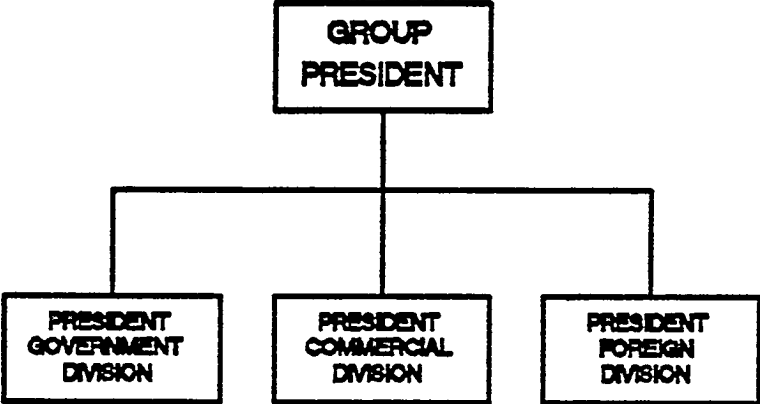
FIGURE 3.5 Customer organization.
