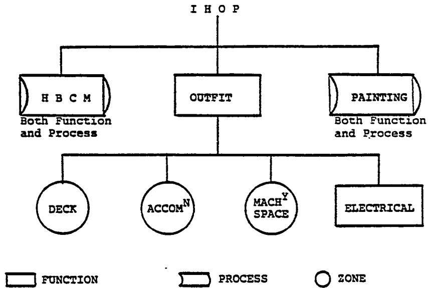
FIGURE 3.10 IHOP organization.
