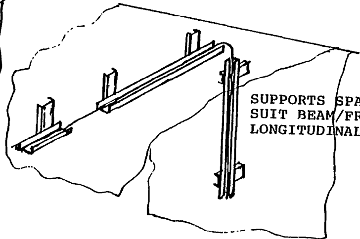
FIGURE 1.122 Small cable support design for production.
