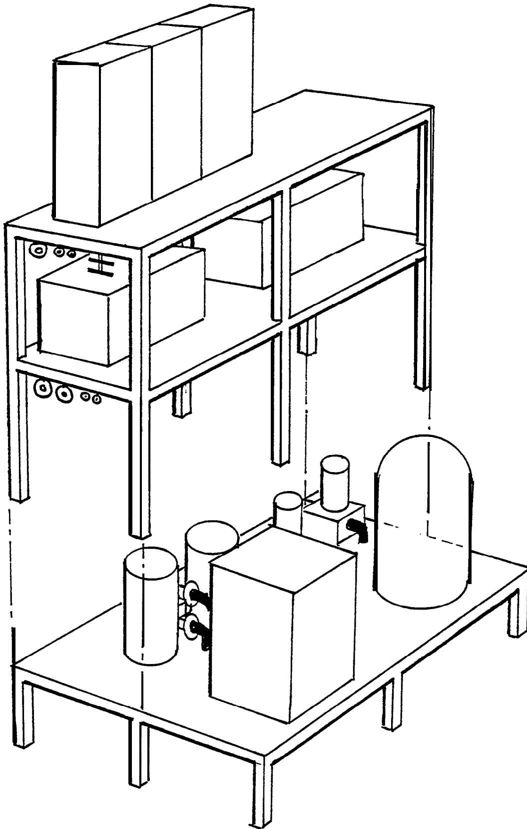
FIGURE 1.138 Wartsila "macromodule" advanced outfitting.
