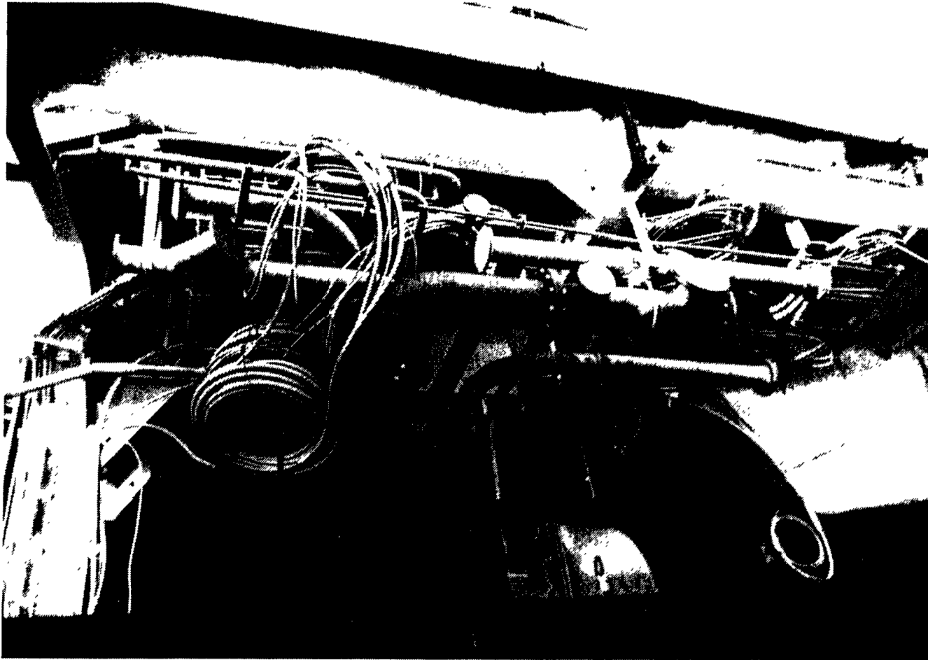
FIGURE 1.130 "On-block" advanced outfitting.
