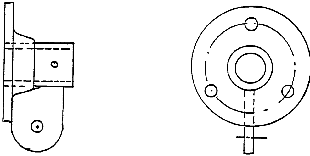
TOP FITTING
