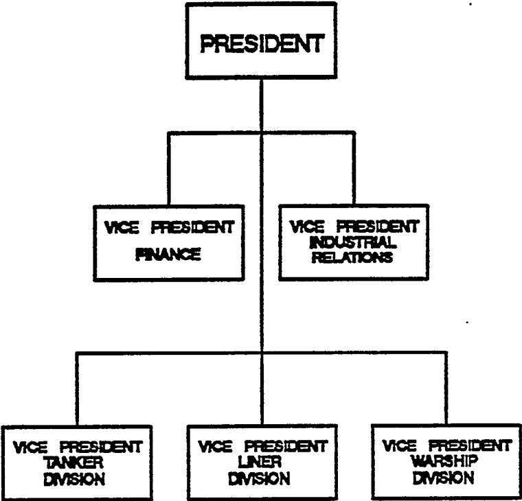
FIGURE 3.3 Product organization.
