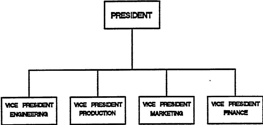
FIGURE 3.2 Functional organization.
