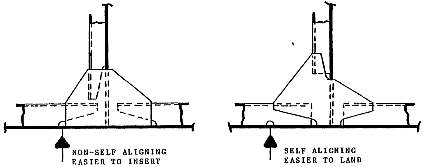
ALTERNATIVE WHEN LONGITUDINALS CAN BE CUT AT TRANSVERSE BULKHEADS
