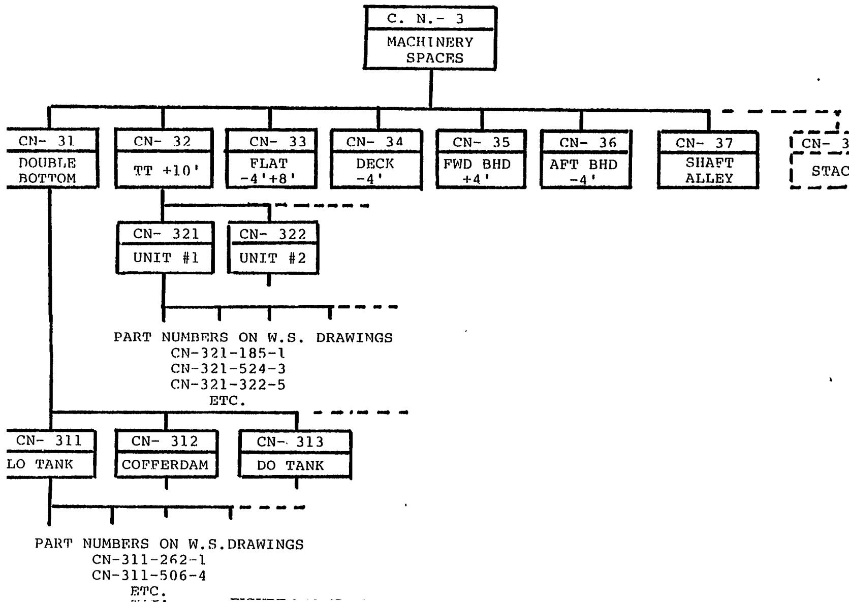
FIGURE 2.18 (Continued)-Machinery spaces zone breakdown.
