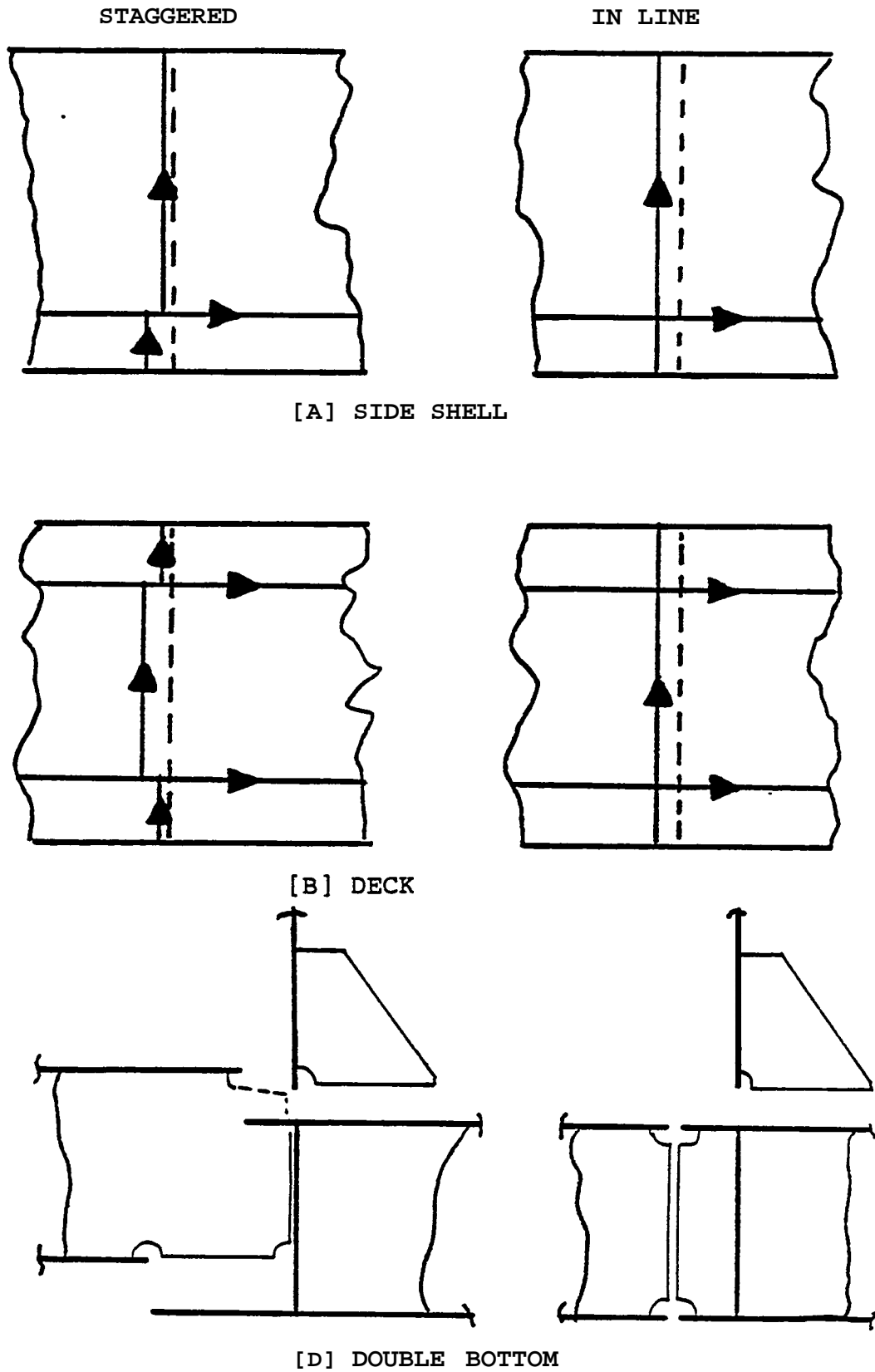
FIGURE 1.43 Module connection definition.
