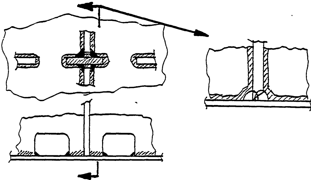
FIGURE 1.62 Oil/water stop design for productivity.
