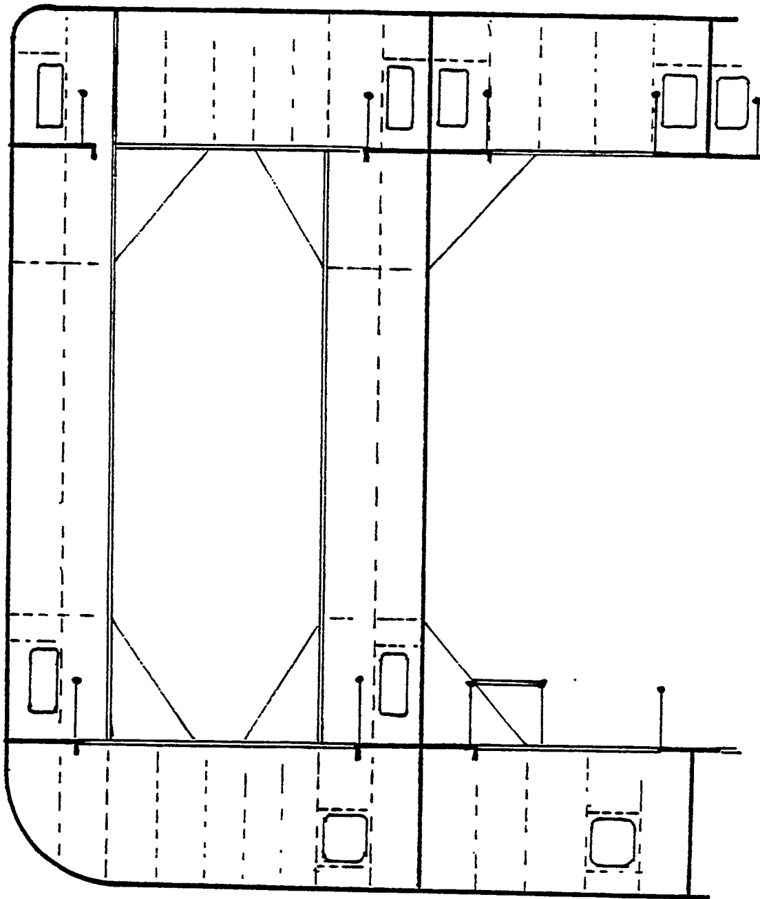
FIGURE 1.70 Tanker with "built-in" access galleries.
