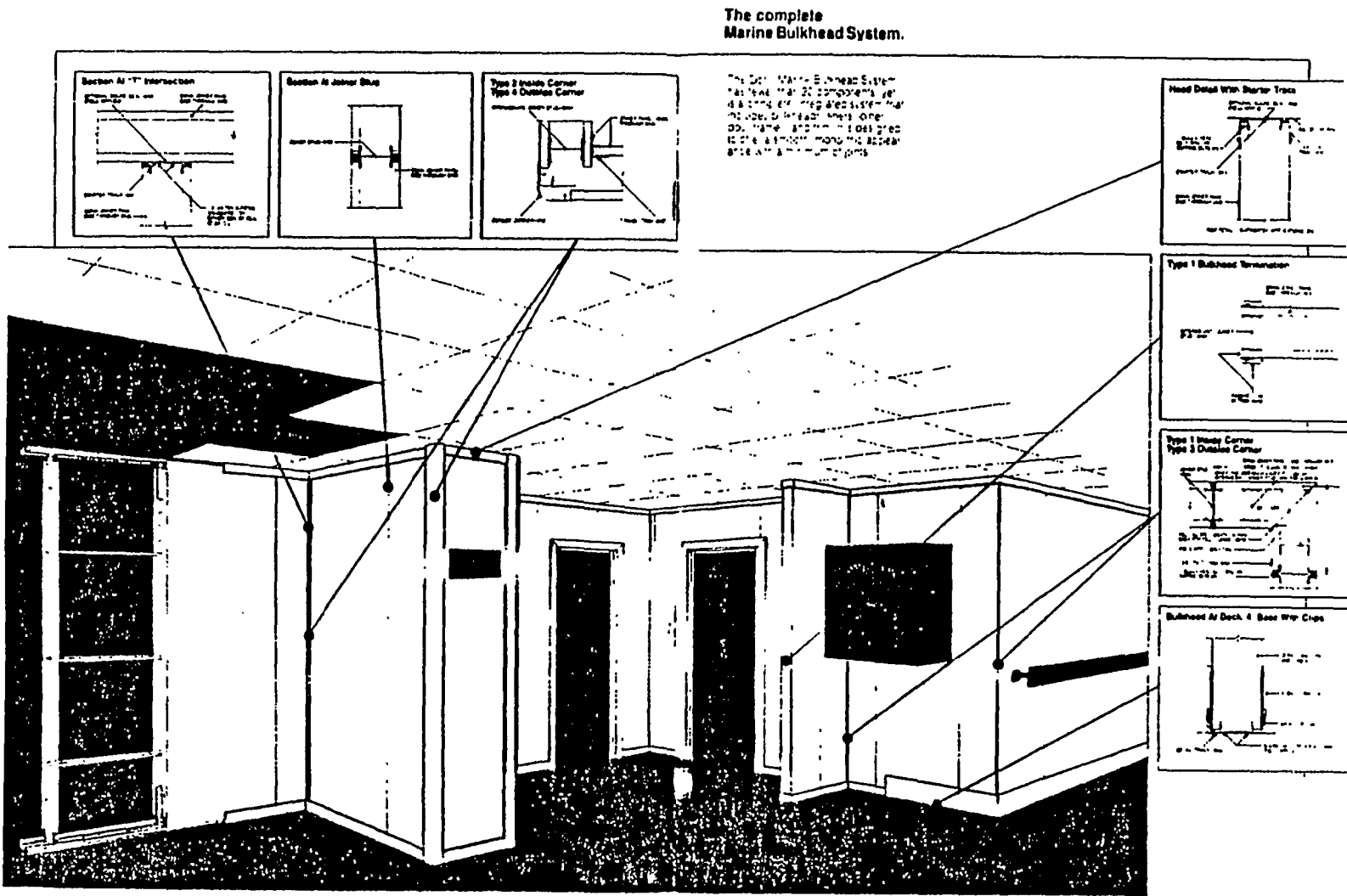
FIGURE 1.92 The Donn joiner bulkhead and lining system.
