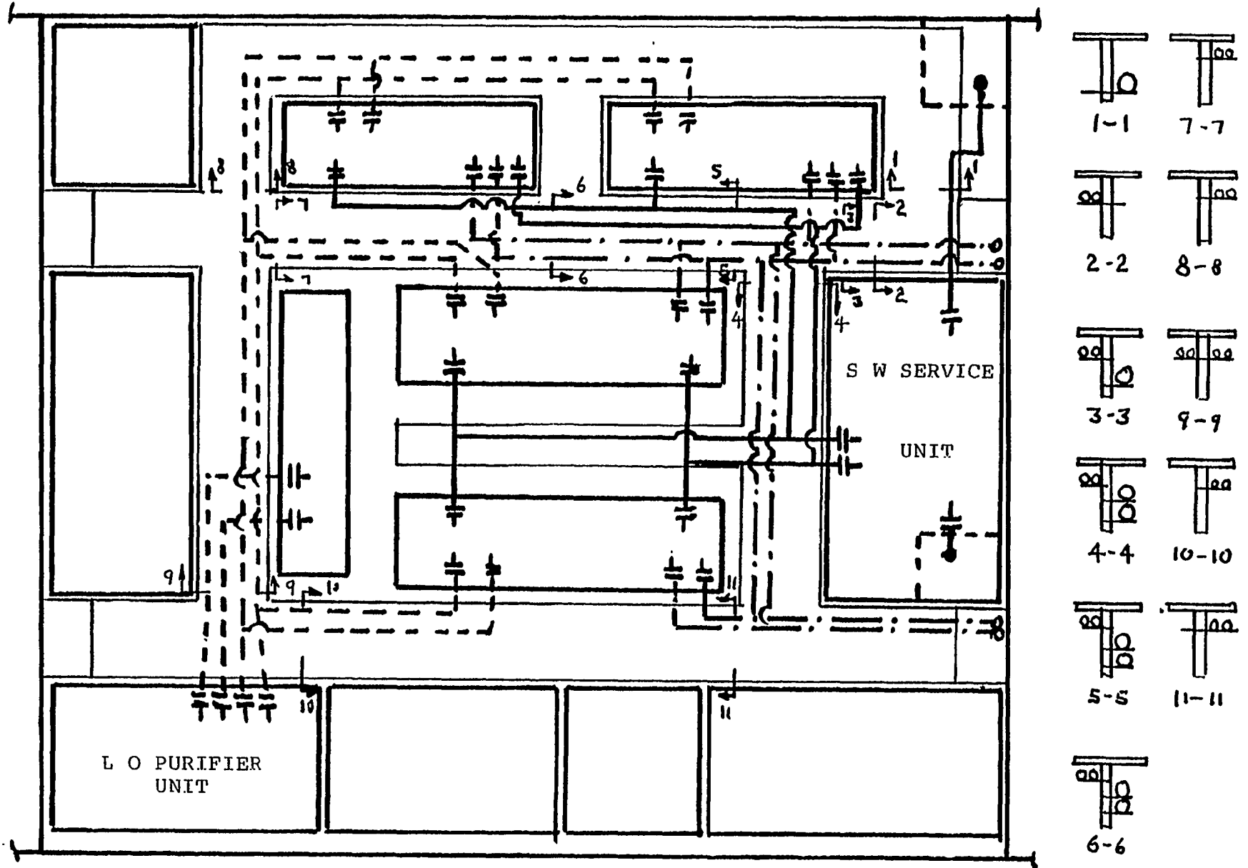
FIGURE 2.13 Distributive system routing diagrammatic.
