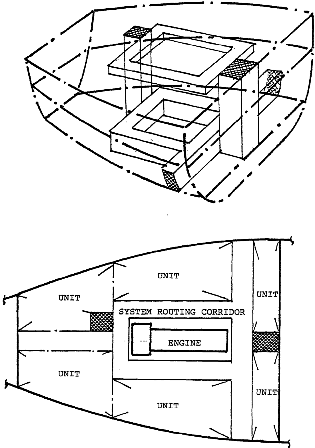
FIGURE 1.109 Distributive system corridors.
