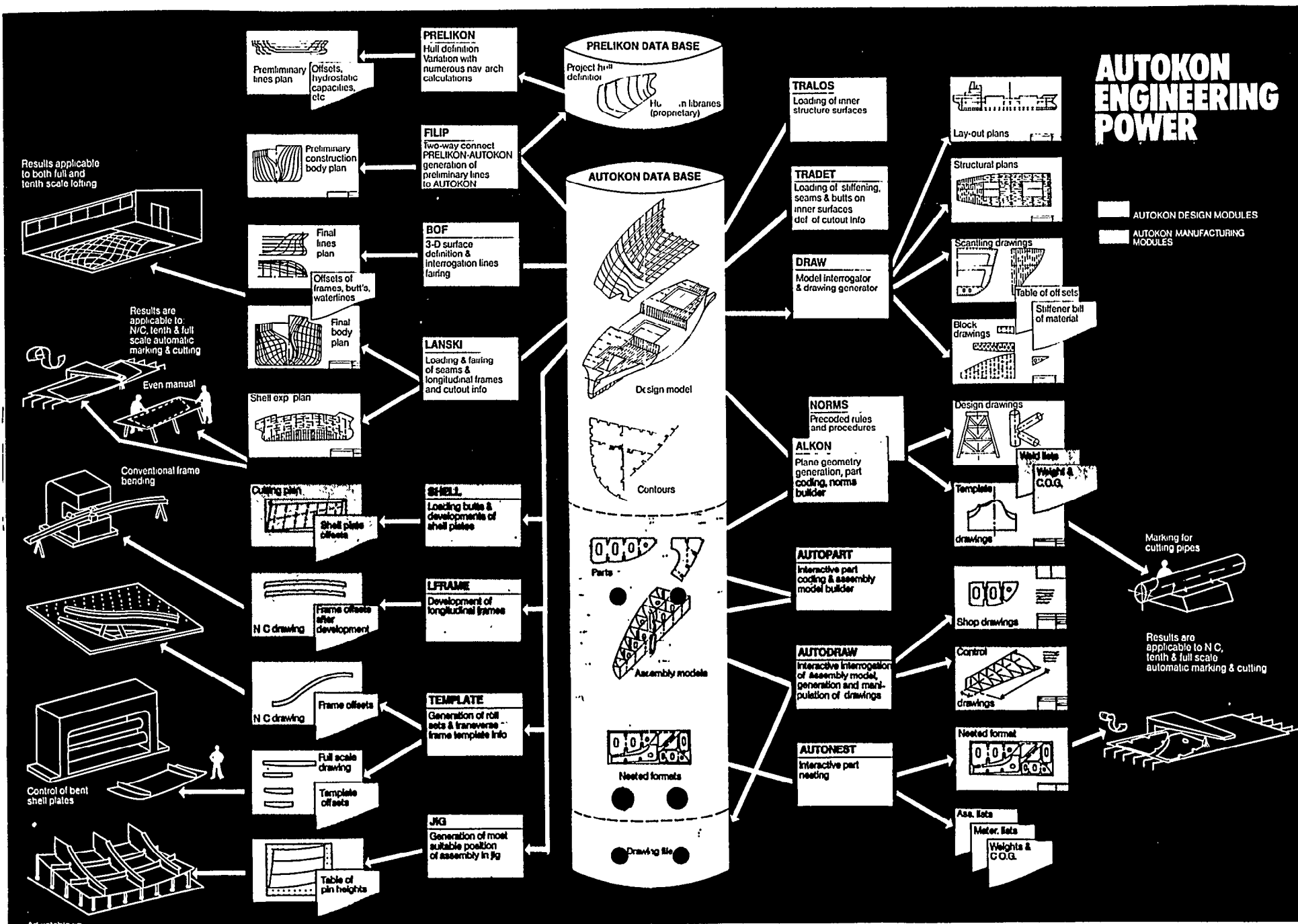
FIGURE 2.68 AUTOKON 79 system.
