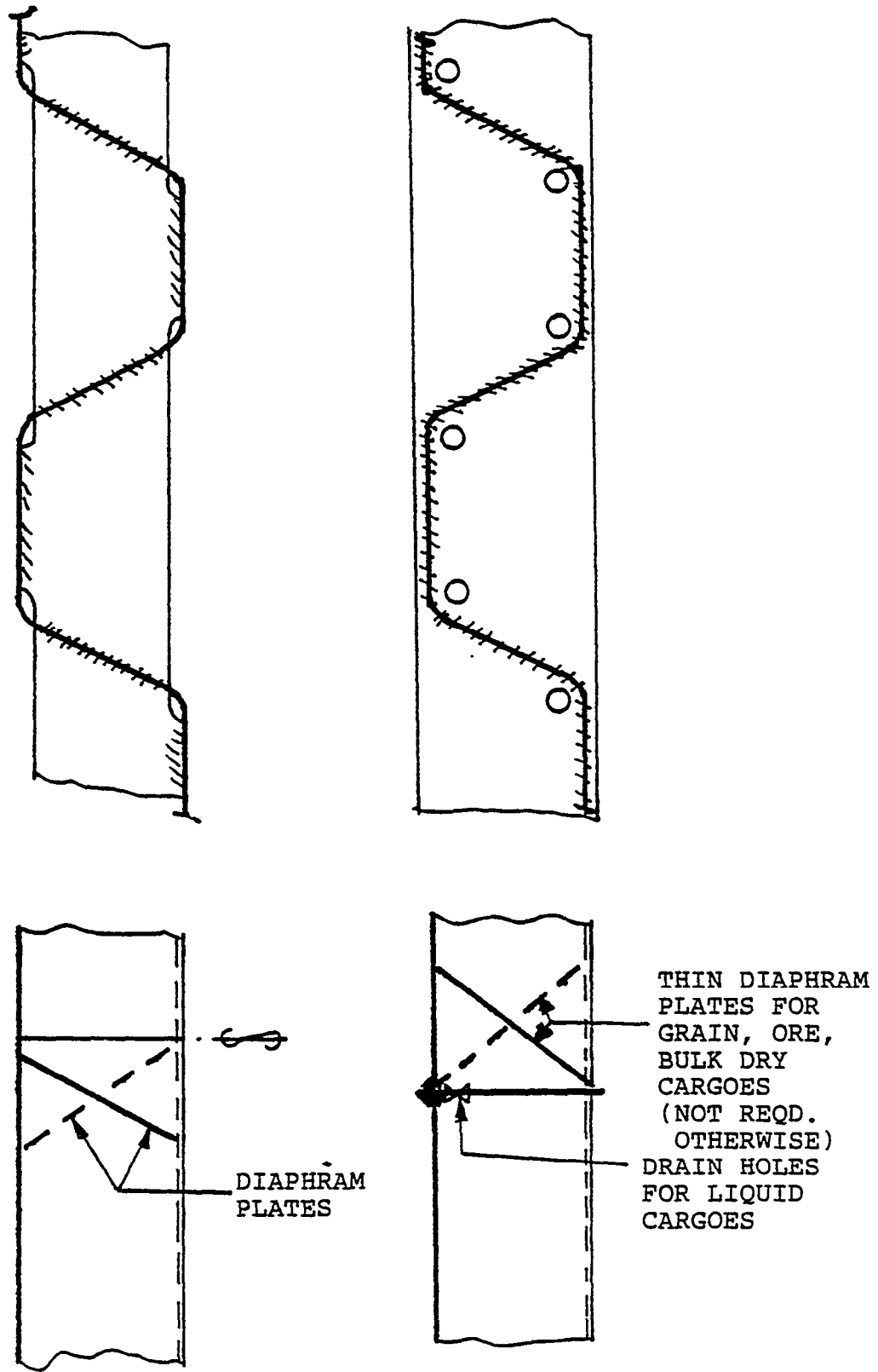
FIGURE 1.75 Corrugated panel details.
