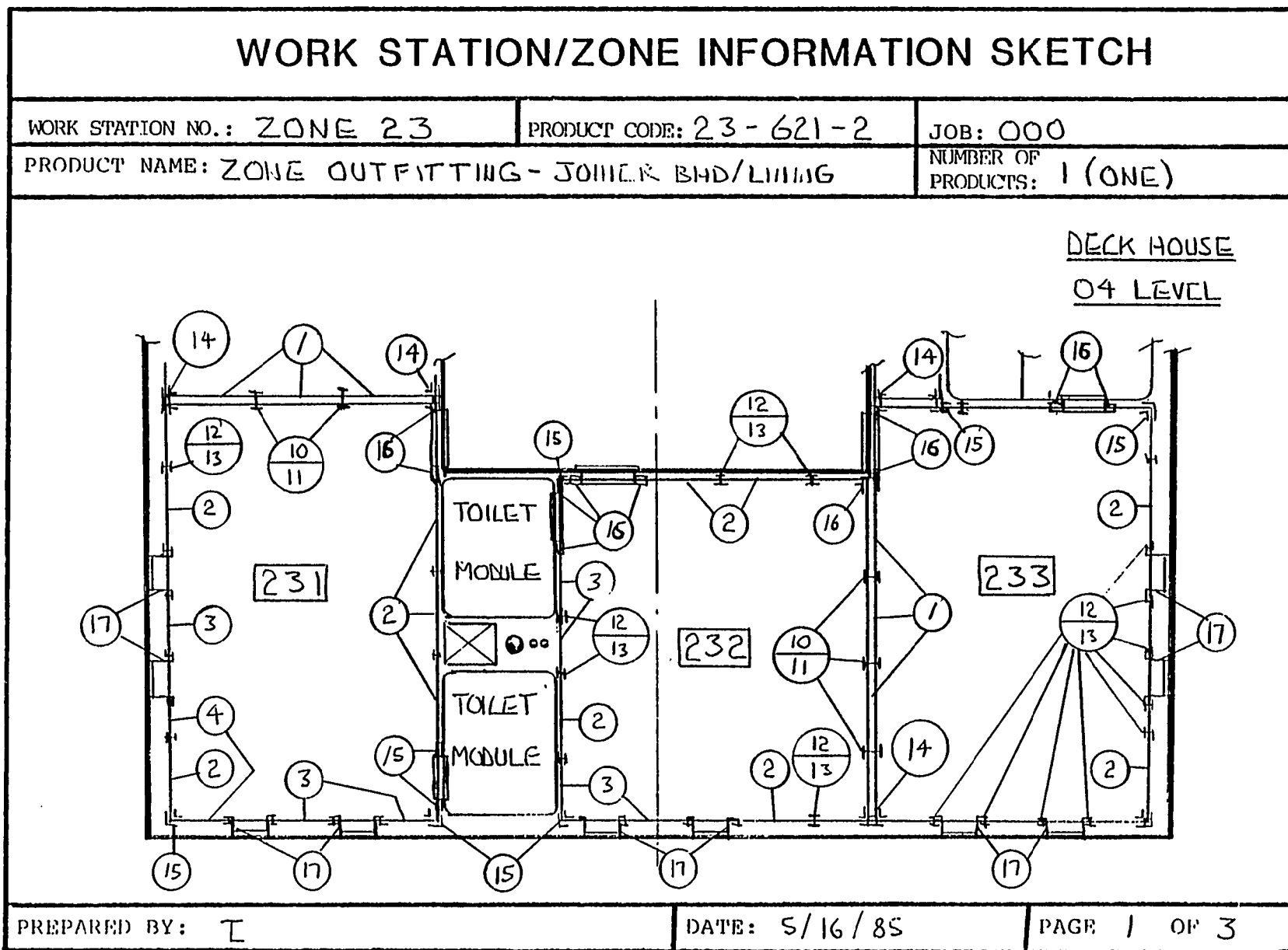
FIGURE 2.51 Deckhouse zone information for joiner lining and bulkheads.
