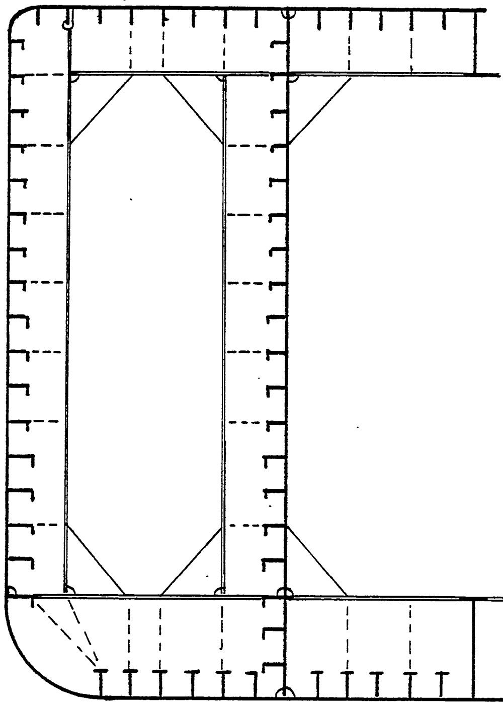
FIGURE 1.55(a) Tanker structural detail for "layer" construction method.
