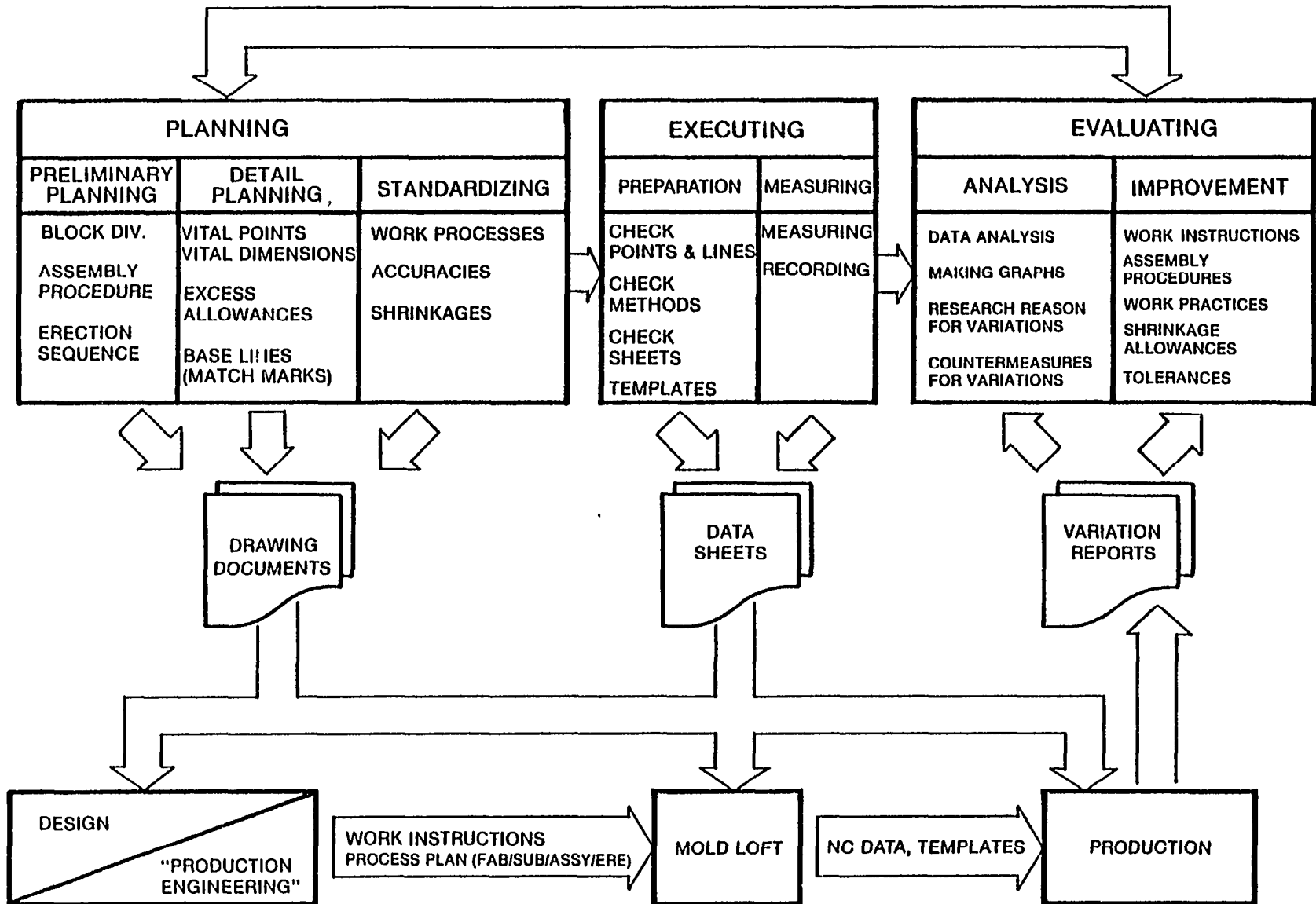
FIGURE 2.10 Phases of accuracy control.
