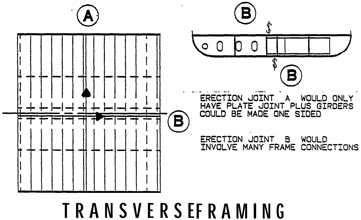
FIGURE 1.51 Producibility considerations for module breaks.
