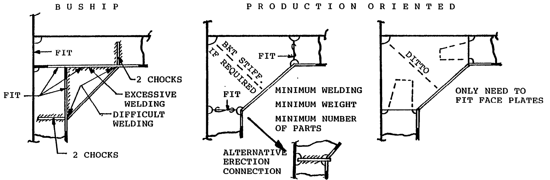
[A] - BEAM/FRAME DETAIL
