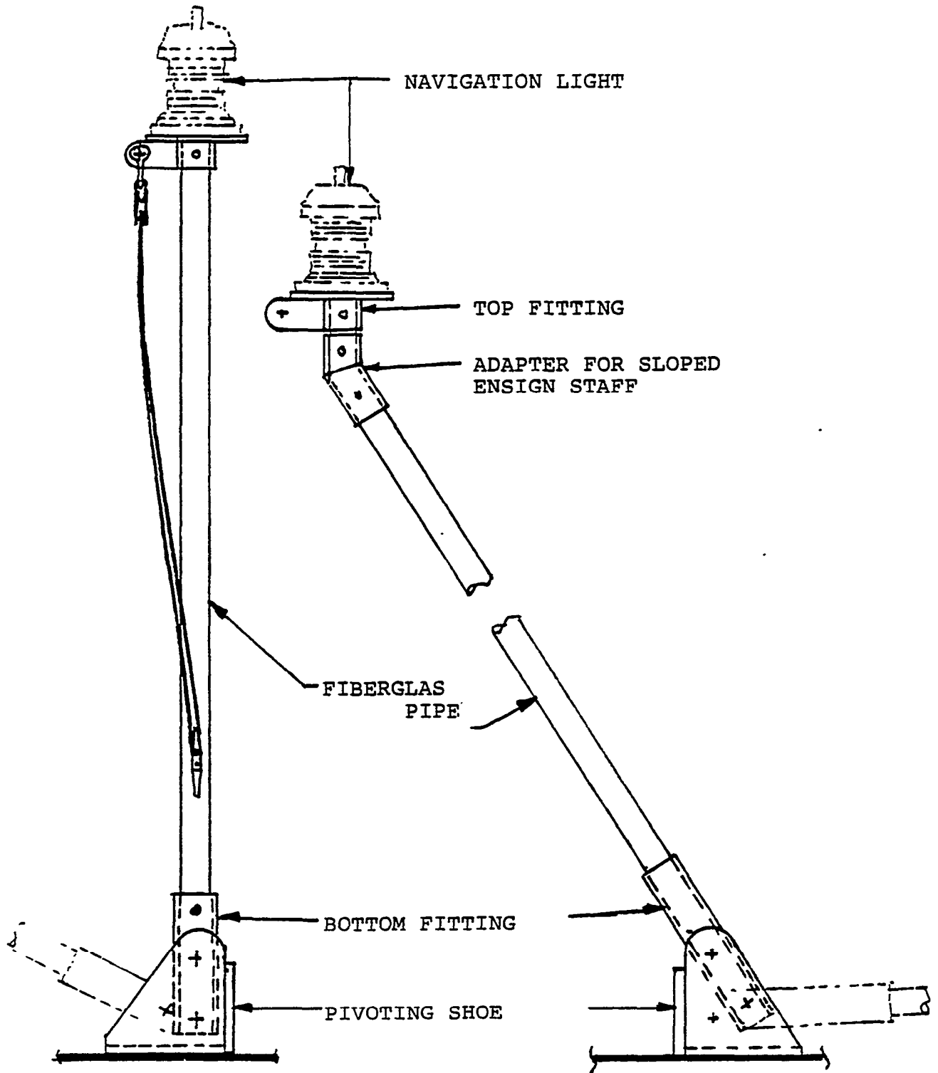
FIGURE 1.85(a) Standard jack and ensign staffs.
