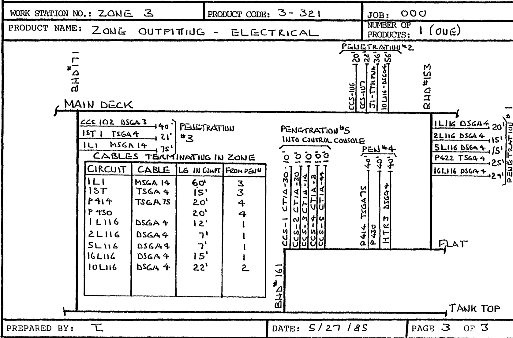
FIGURE 2.46 Zone information, cable penetrations, starts, ends, and lengths.
