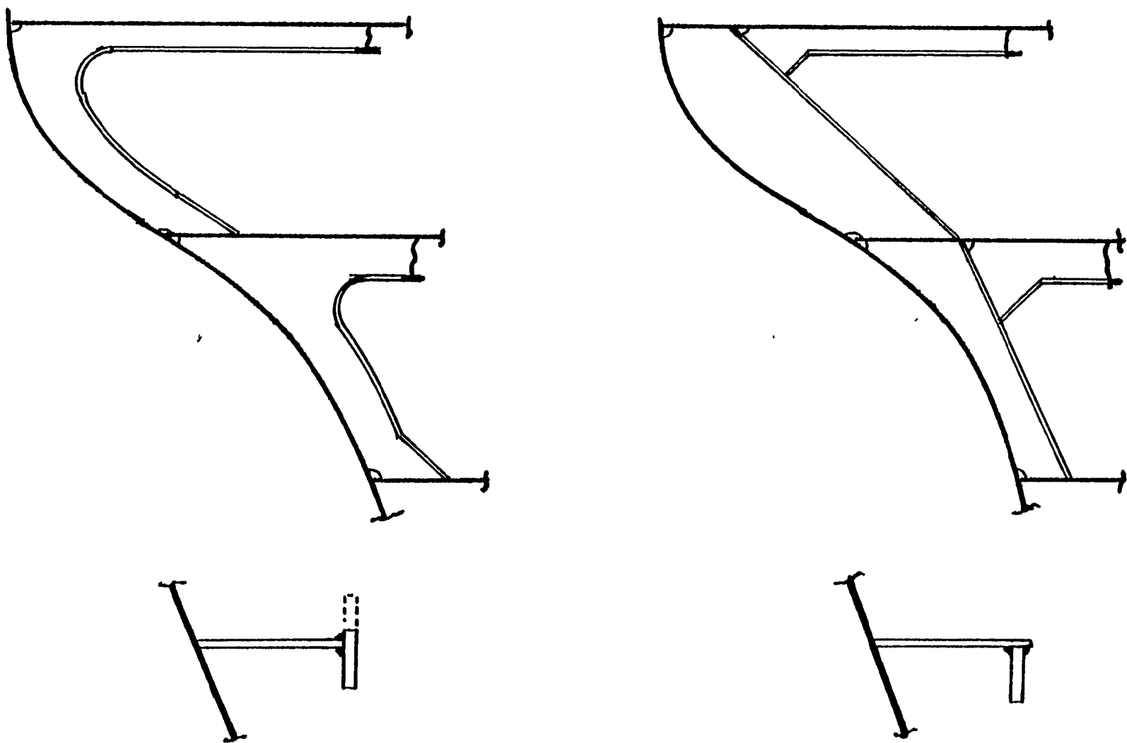
FIGURE 1.67 Web frame design for productivity.
