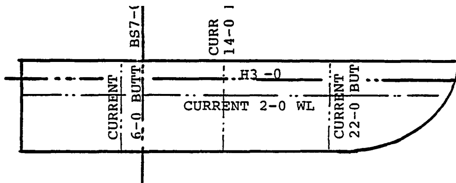
FLOOR ASSEMBLY SHOWING CURRENT AND SUGGESTED MARKING (TWO LESS LINES)
