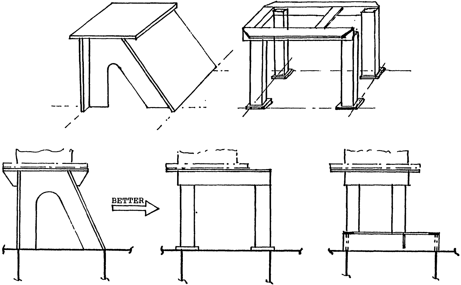
FIGURE 1.80 Foundation design for productivity.
