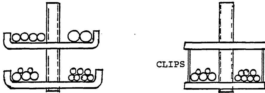
FIGURE 1.120 Cable-retaining methods.
