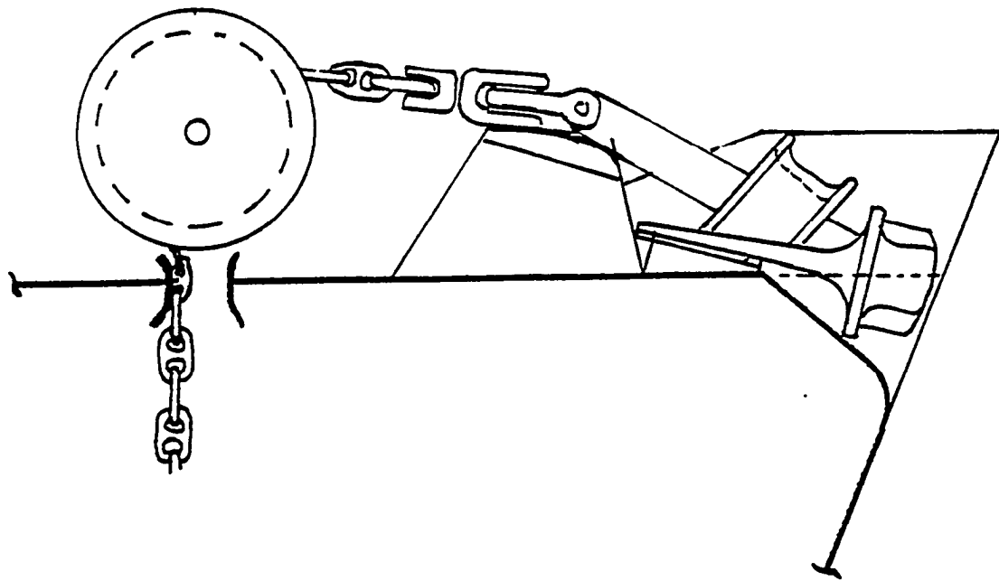
[A] KOCKUM'S DECK ANCHOR STOWAGE ARRANGEMENT
