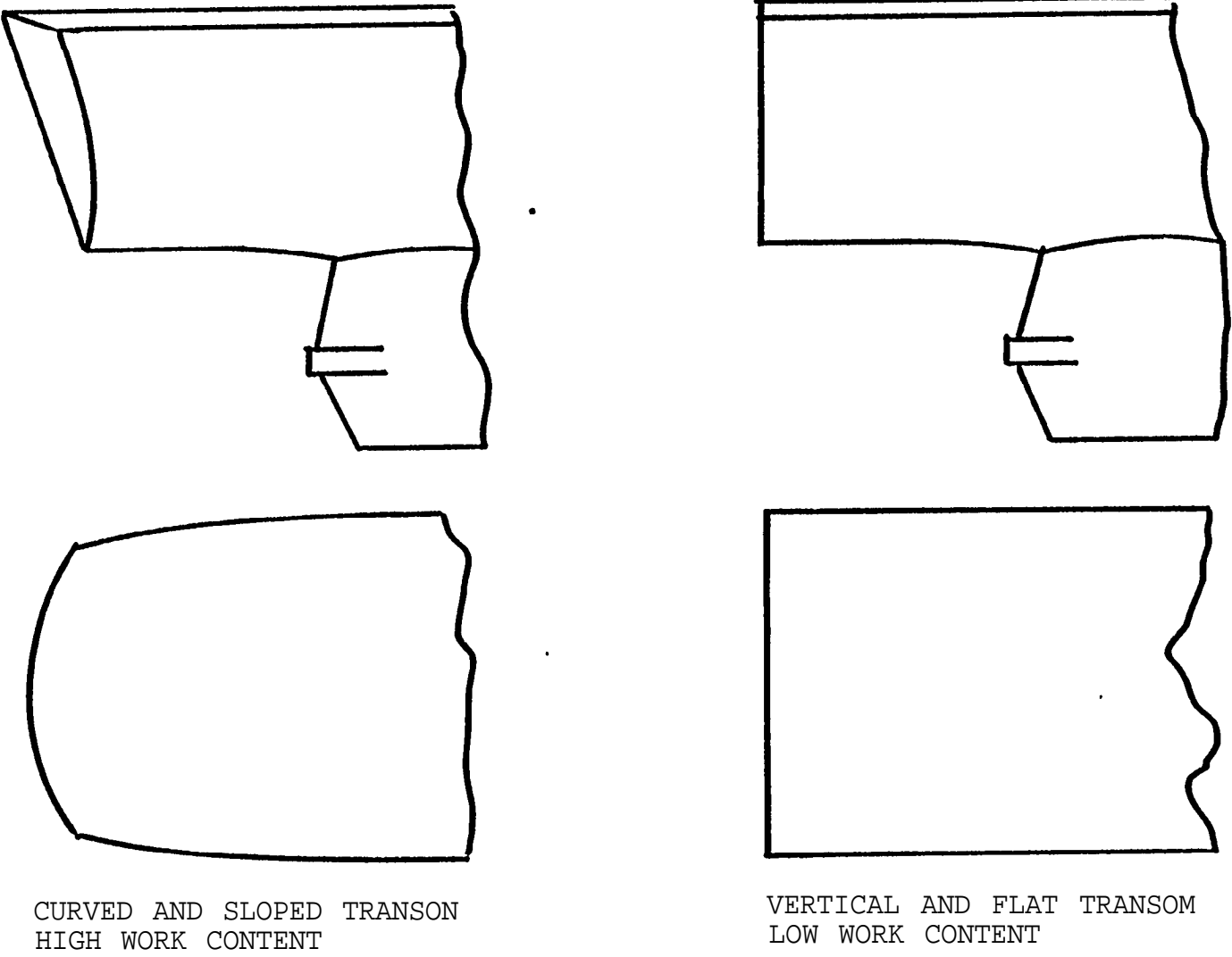
FIGURE 1.22 Transom stern design for production.
