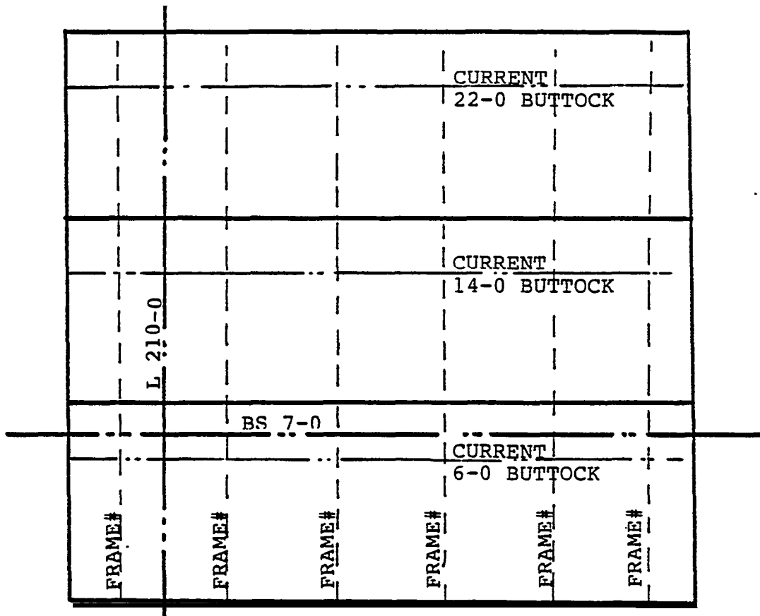
SHELL ASSEMBLY SHOWING CURRENT AND SUGGESTED MARKING (ONE LESS LINE BUT REFERENCE LINE L210 IS VISIBLE AFTER ASSEMBLY WHEREAS FRAME LINE DISAPPEARS UNDER FLOOR)
