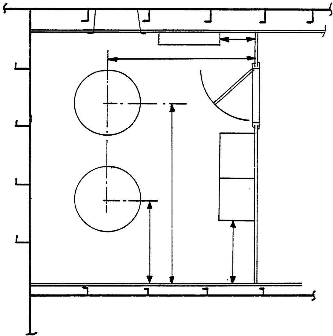
FIGURE 1.33 Tertiary reference system.
