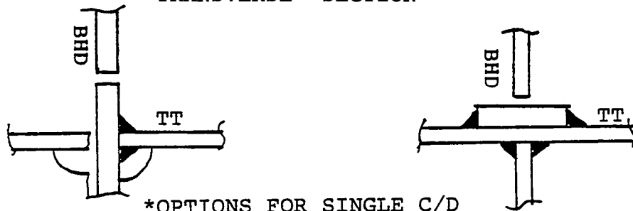
FIGURE 1.46 Use of cofferdams as a module joining aid.
