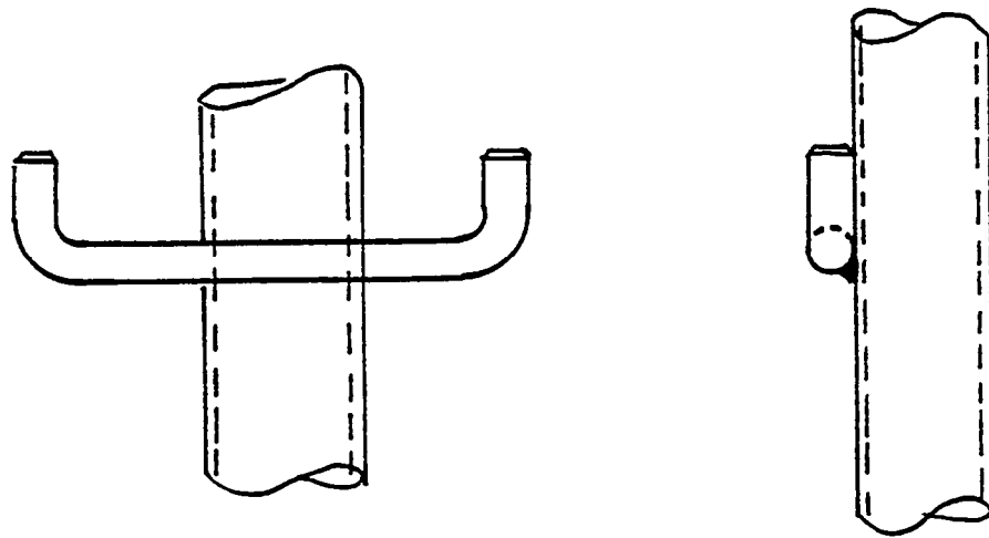
LADDER RUNG FOR WELDING TO MASTS, STAFFS, ETC.
