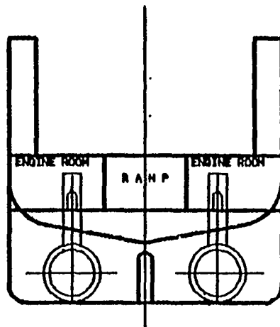
FIGURE 1.7. Split-engine room with azimuthing propulsors.
