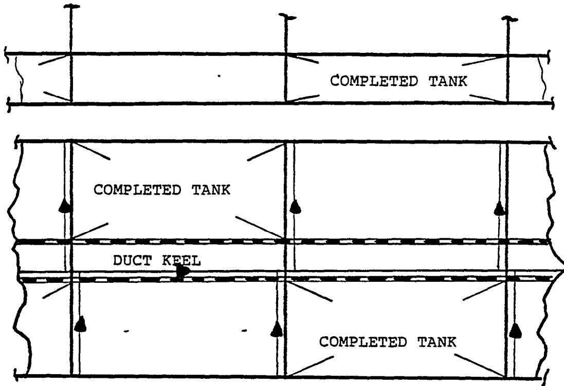
FIGURE 1.47 Arrangement of module joints to facilitate tank completion including alternate tank testing.
