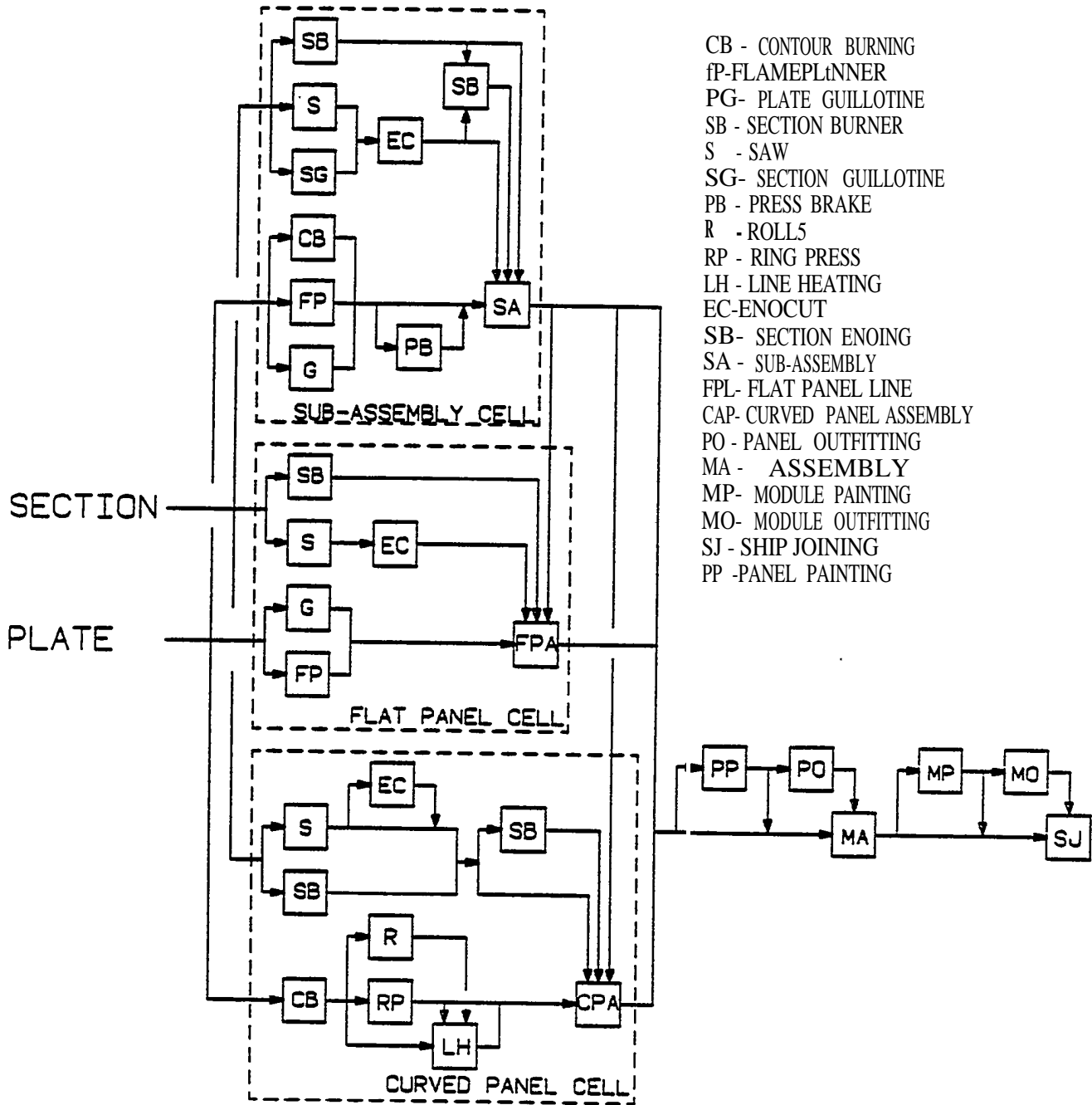
FIGURE 1.34(b) Shipyard group layout.
