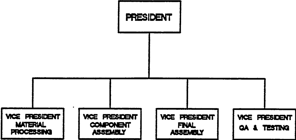
FIGURE 3.4 Process organization.
