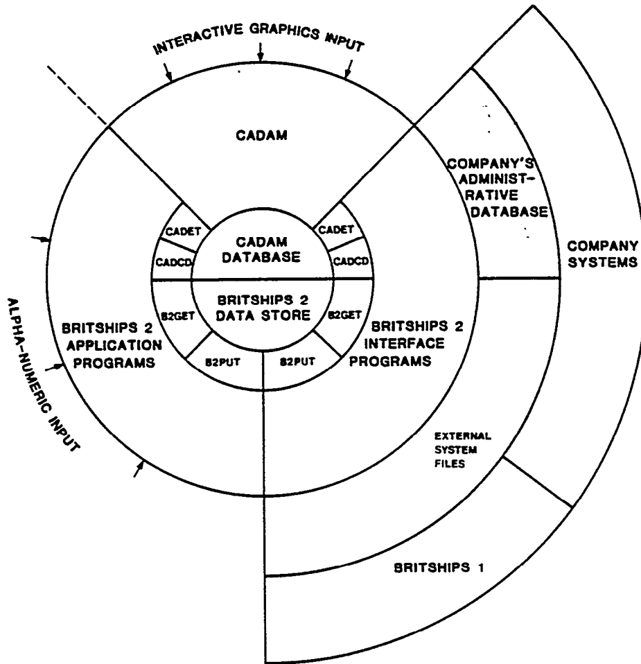
FIGURE 2.67 BRITSHIP 2/CADAM interface.
