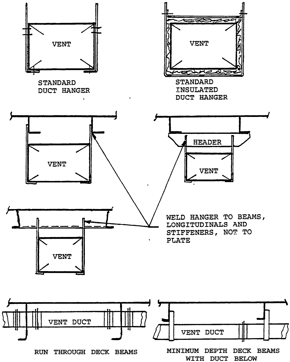
FIGURE 1.118 Standard duct support.
