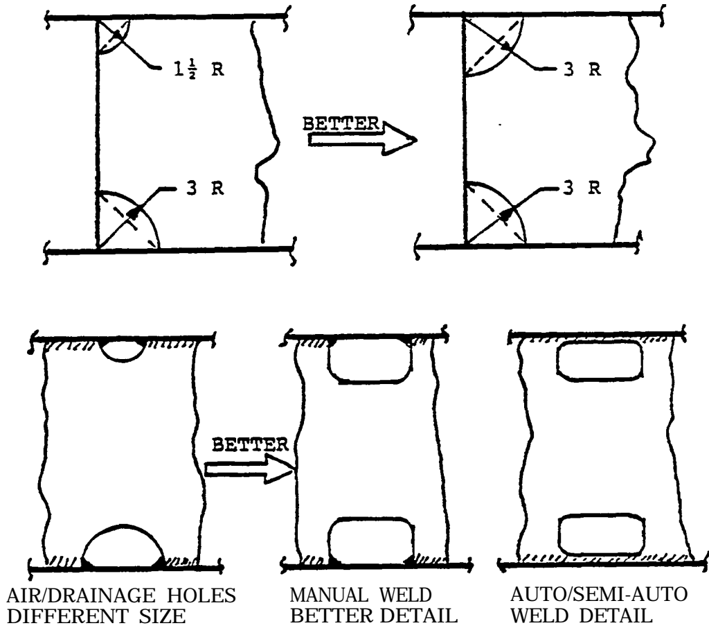
FIGURE X.61 Cut-out alternatives for productivity.
