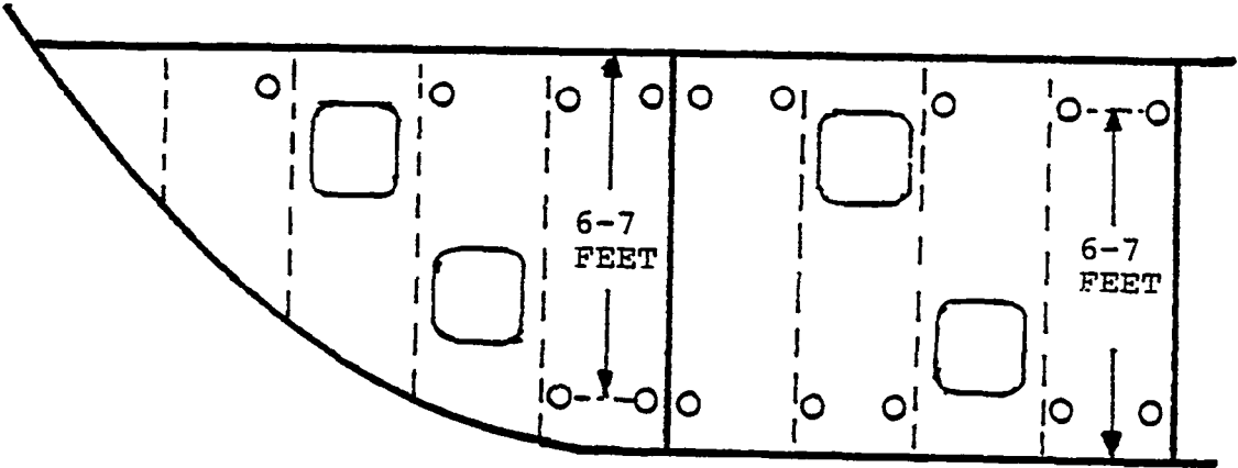
STAGING PIPE HOLES IN DOUBLE BOTTOM FLOORS
