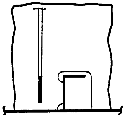
[C] ANGLE OPEN CUT-OUT WITH UNATTACHED STIFFENER
