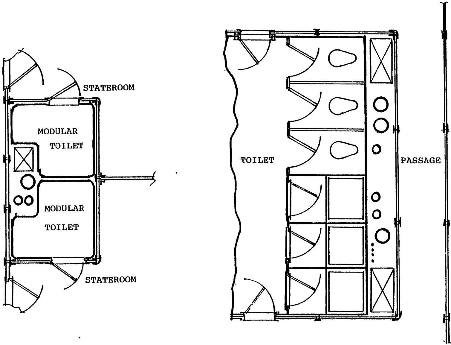
FIGURE 1.100 "Designed-in" service space accessible by removing joiner lining.
