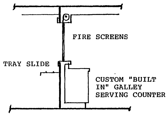
FIGURE 1.99 Galley arrangement for productivity.
