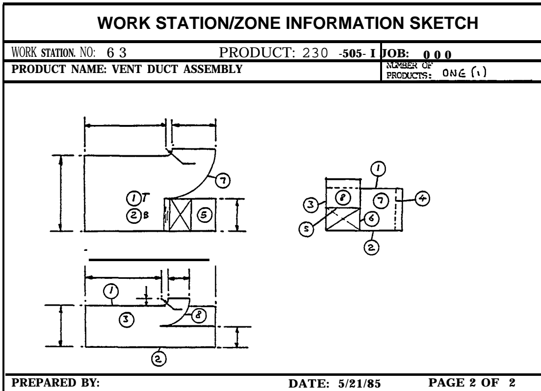
FIGURE 2.30 Hull ventilation duct assembly work Station information.
