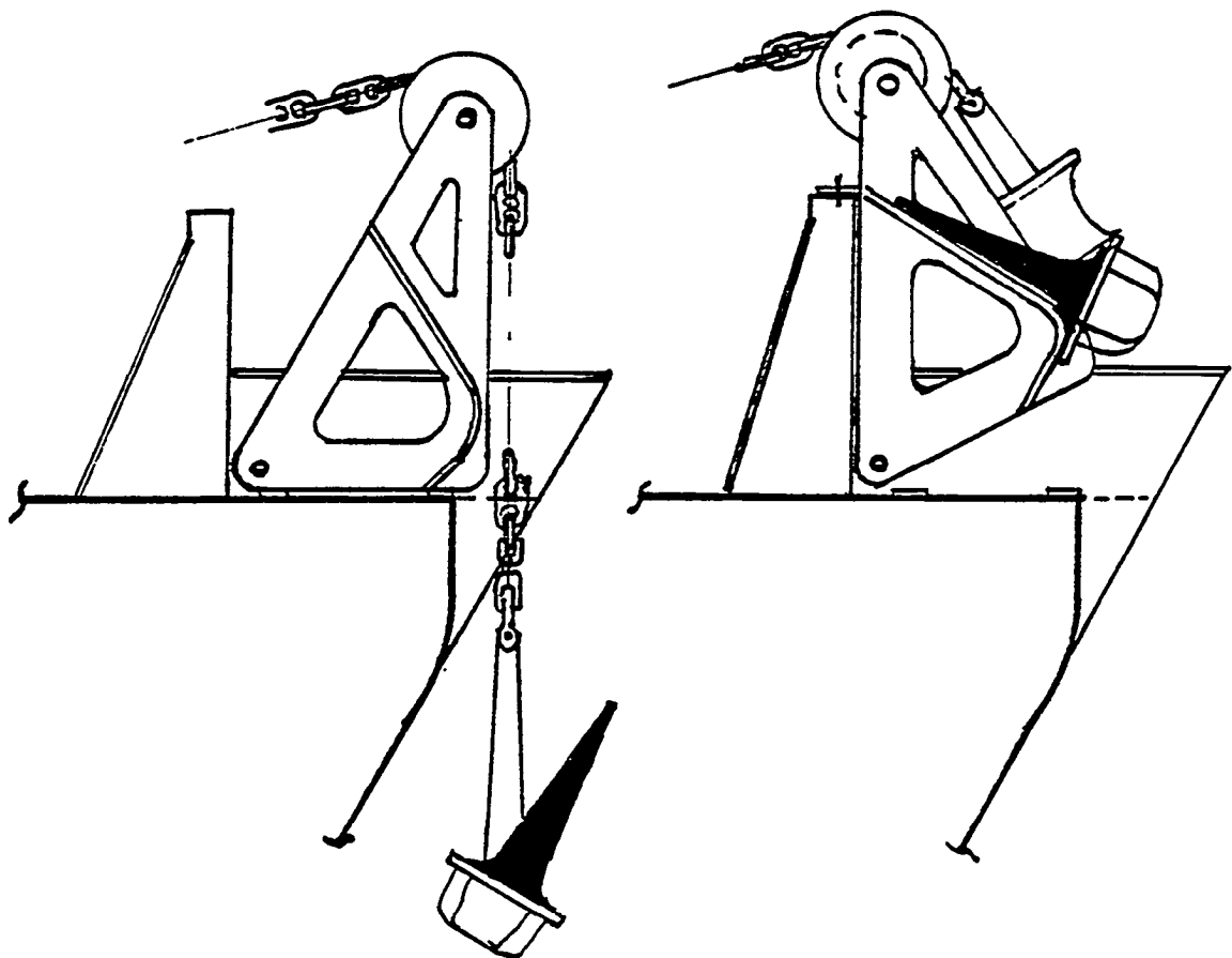
[B] LAMB'S PIVOTING ANCHOR GALLOWS ARRANGEMENT
