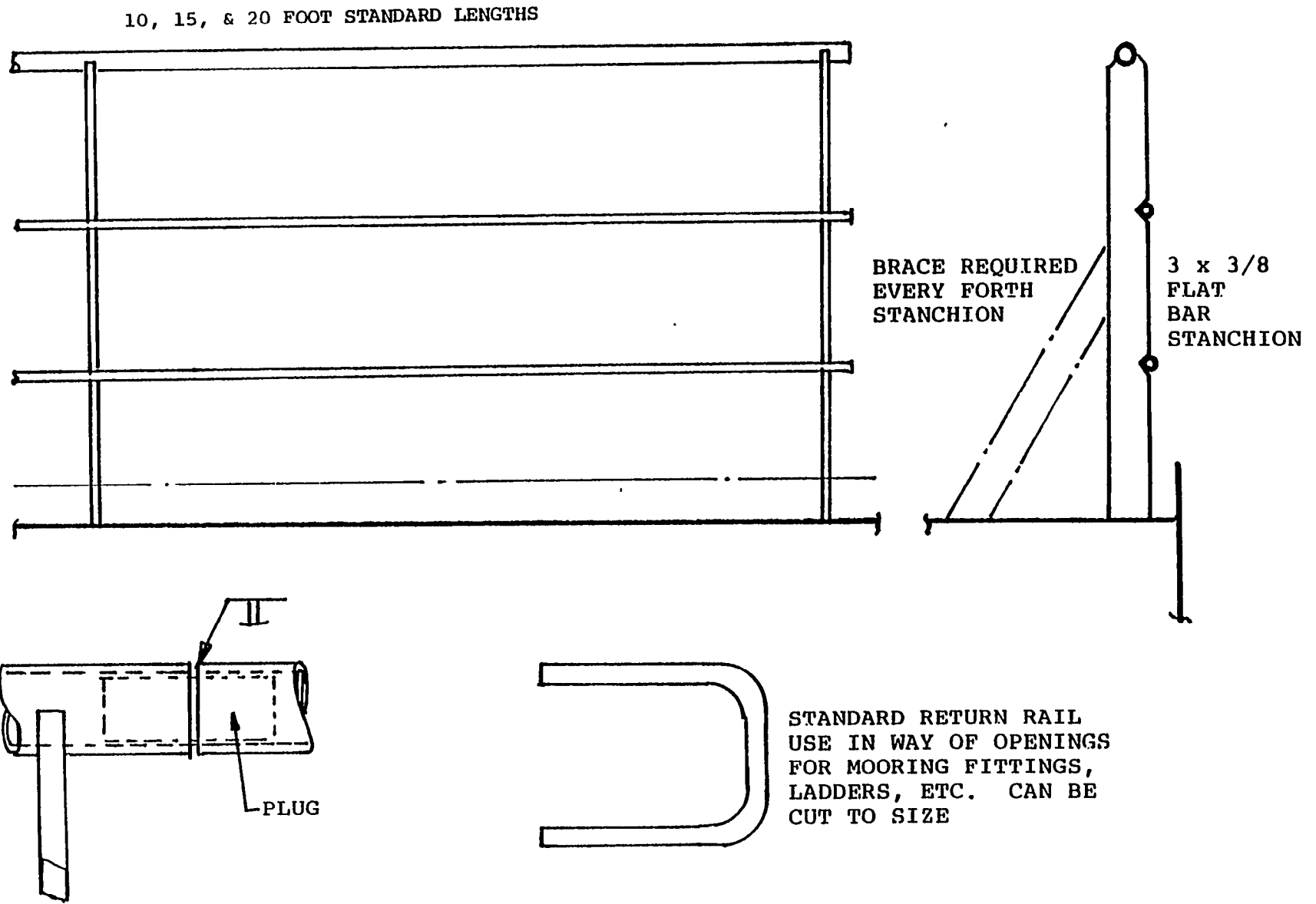
FIGURE 1.82 Standard exterior handrails.
