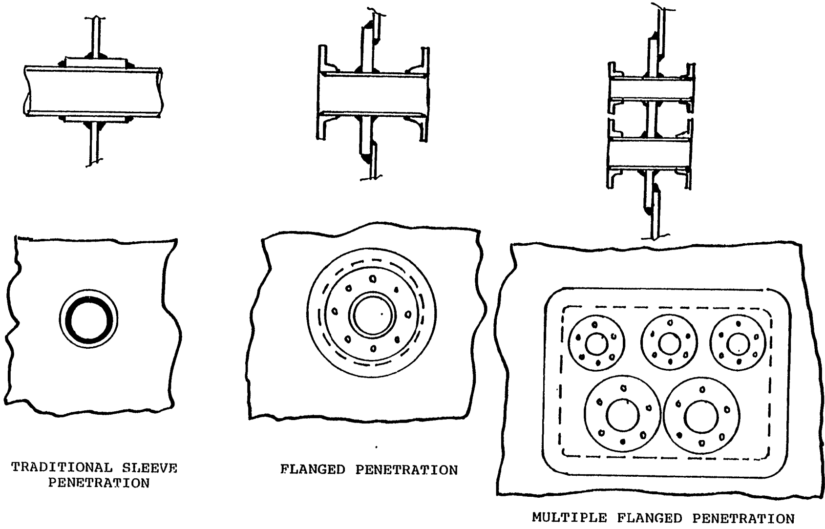
FIGURE 1.112 Piping penetration design for productivity.
