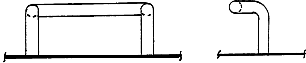
LADDER RUNG FOR WELDING TO STRUCTURE
