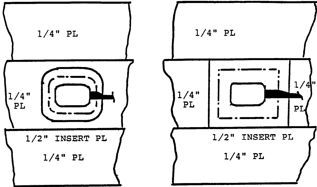
[A] TRADITIONAL INSERT PLATE
