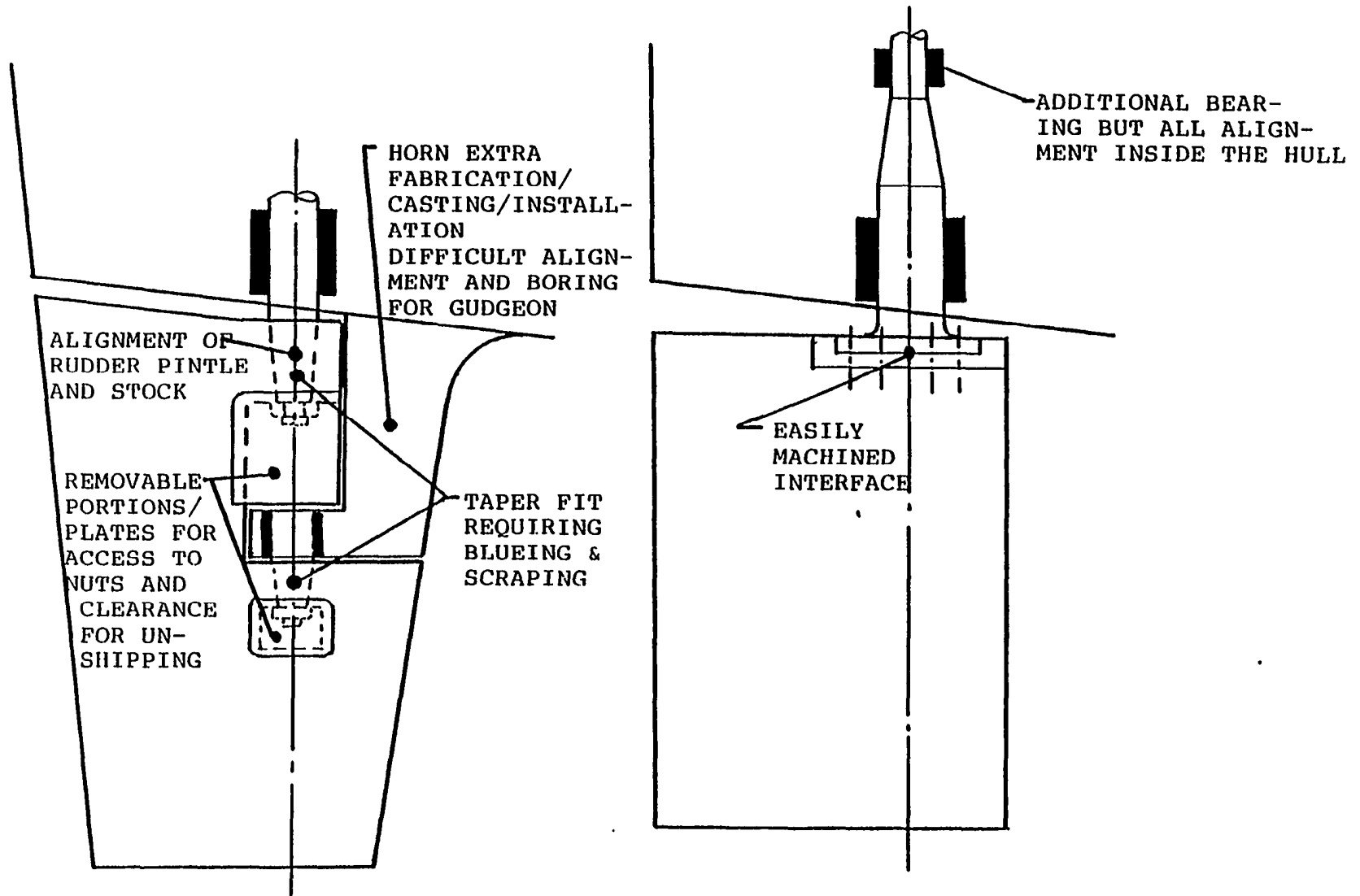
FIGURE 1.21 Rudder-type selection for producibility.
