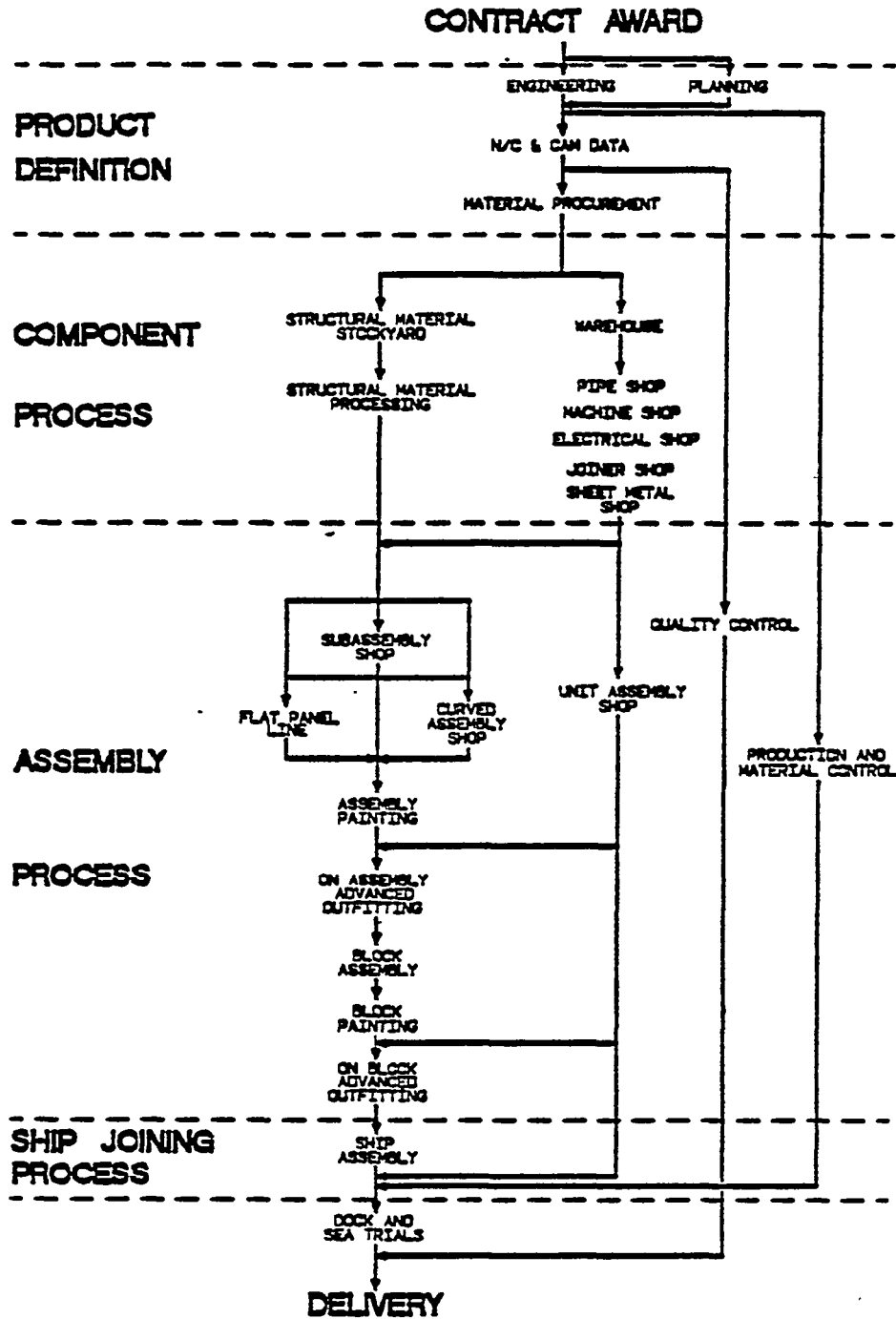
FIGURE 1.2 The shipbuilding process.
