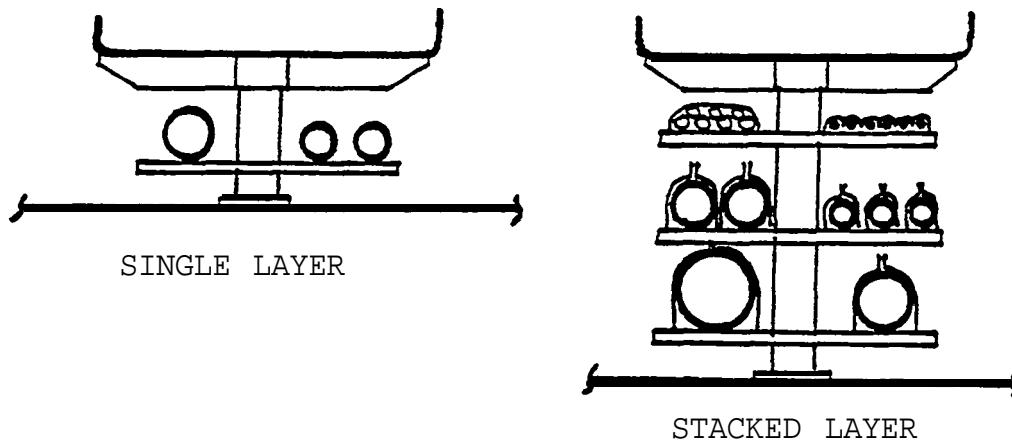
[A] COMBINED FLOOR PLATE/SYSTEMS SUPPORT
