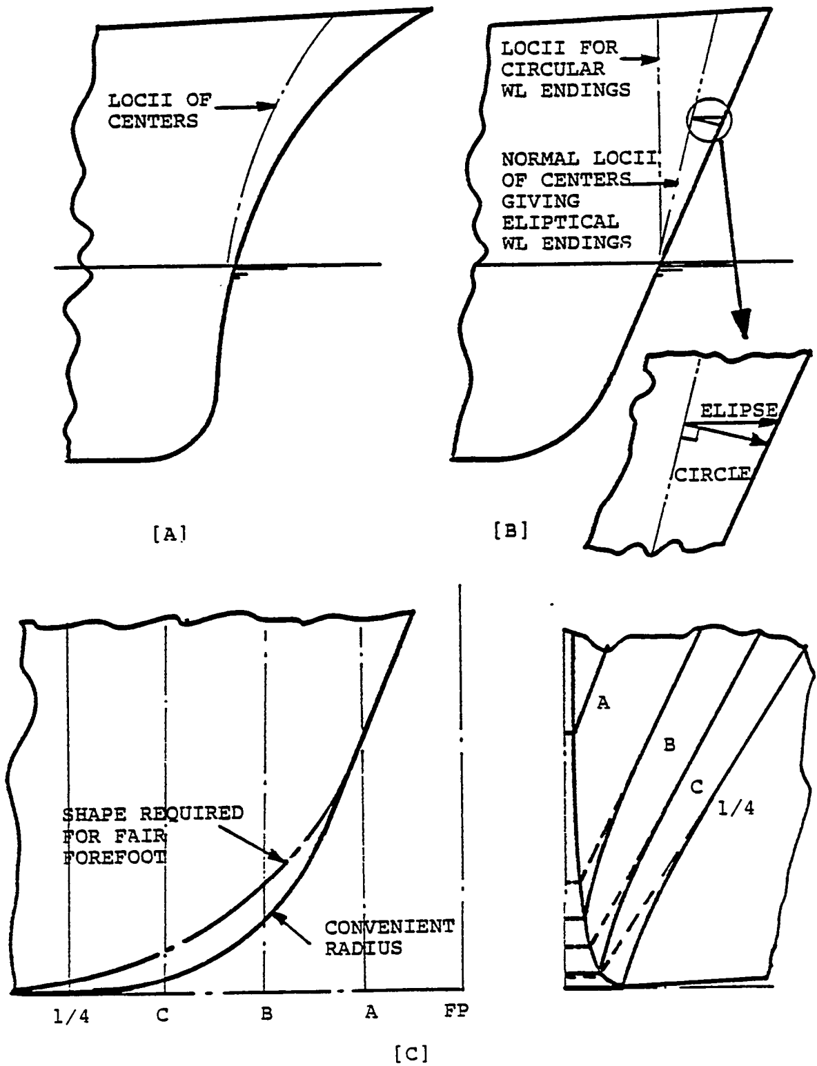
FIGURE 1.18 Stem productivity considerations.
