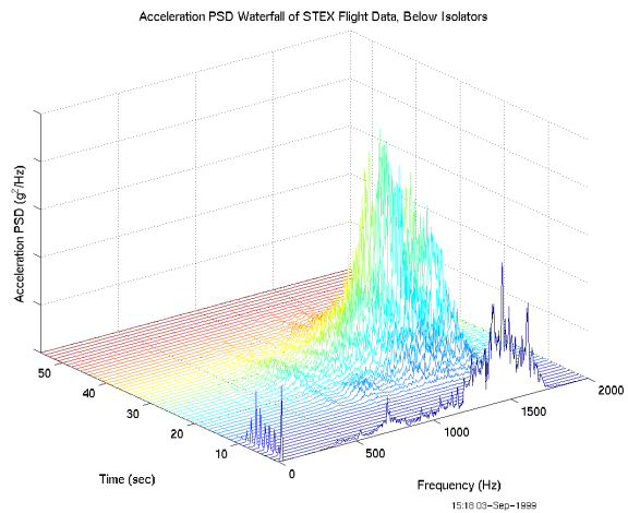
Figure 11 Waterfall PSD of STEX data - below isolators
