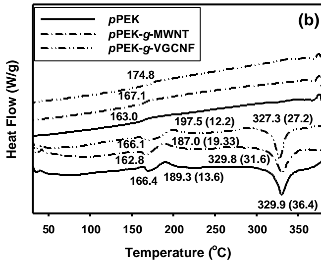
Figure 4. DSC thermograms of PEK (solid), PEK-g-MWNT (dash-dot-dash) and PEK-g-VGCNF (dash-dot-dot-dash) samples run with heating and cooling rates of 10 °C/min: (a) m PEK; (b) p PEK.
