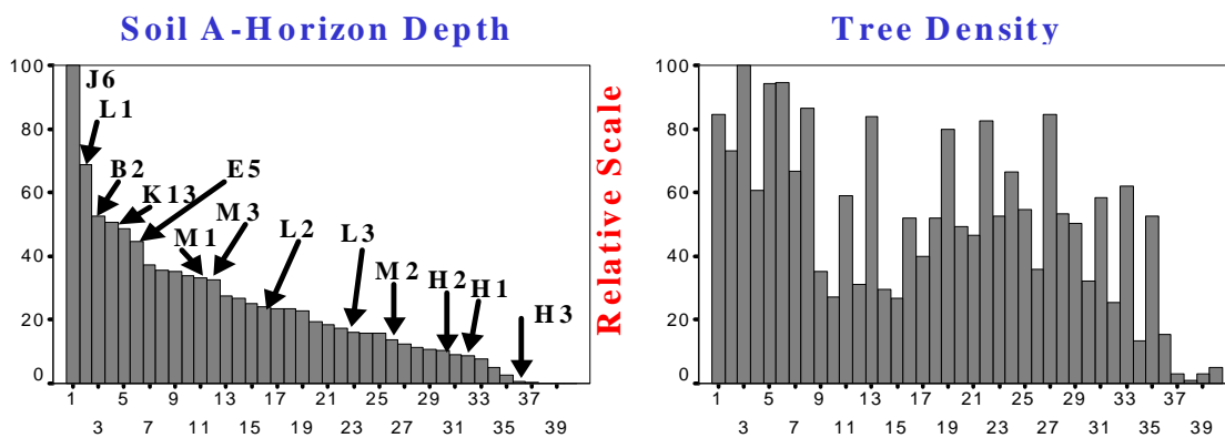
Figure 9-2. Tree density at the 40 sites (right), ranked by soil A-horizon depth. Note that the ordinate is a relative scale where 100 is the maximum possible value.
