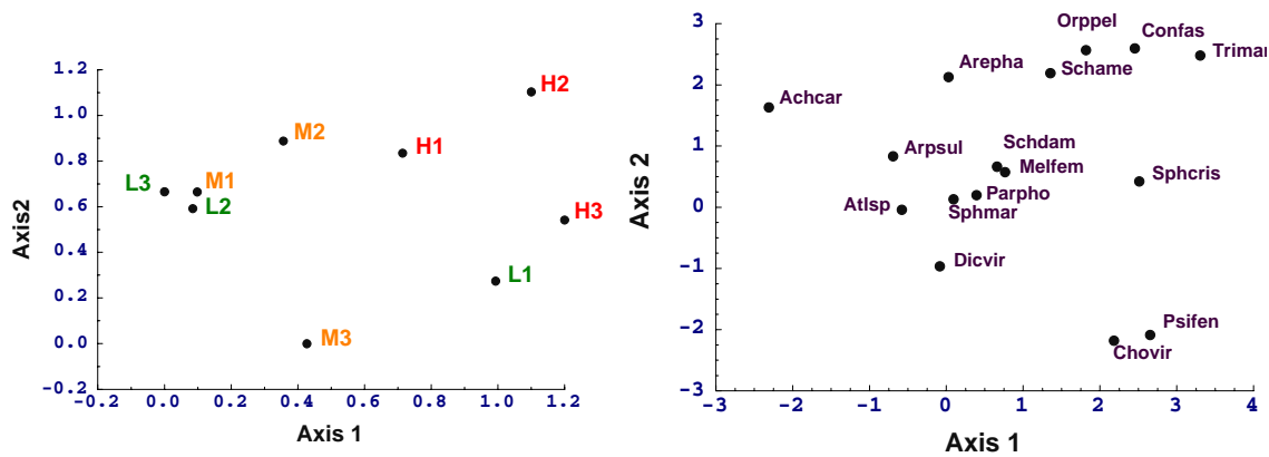
Figure 5-18. Detrended correspondence analysis of grasshopper and katydid Fort Benning communities. Low disturbance sites are in dark green, Medium sites in orange, and High disturbance sites in red.
