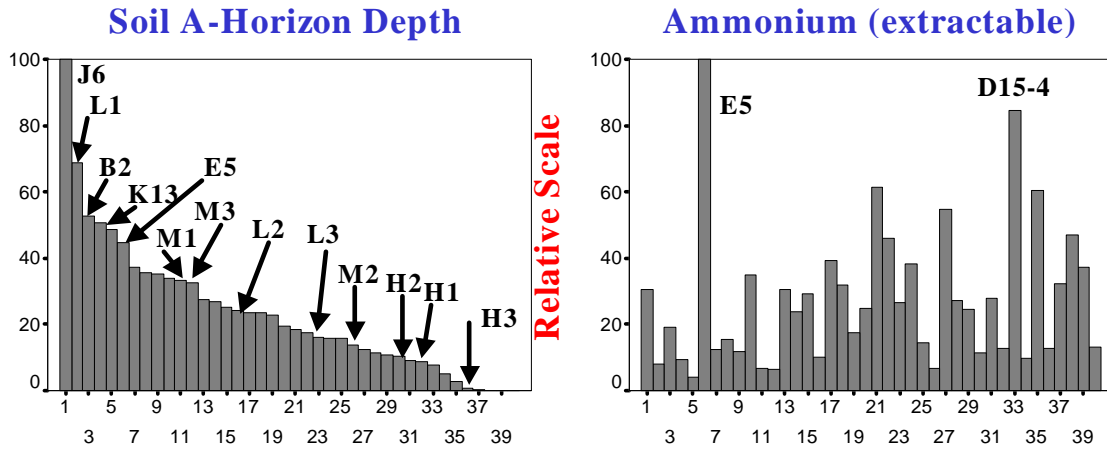
Figure 9-4. Soil ammonium ( \text{NH}_4^+ ) at the 40 sites, ranked by soil A-horizon depth. Note that the ordinate is a relative scale where 100 is the maximum possible value.
