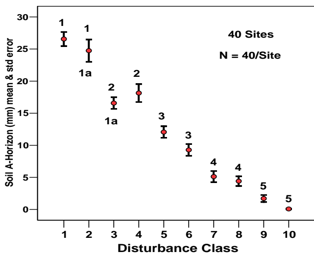
Figure 9-1. Soil A-horizon depth (mean and standard error) at the 40 sites based on disturbance class. Numbers represent statistically similar disturbance classes.
