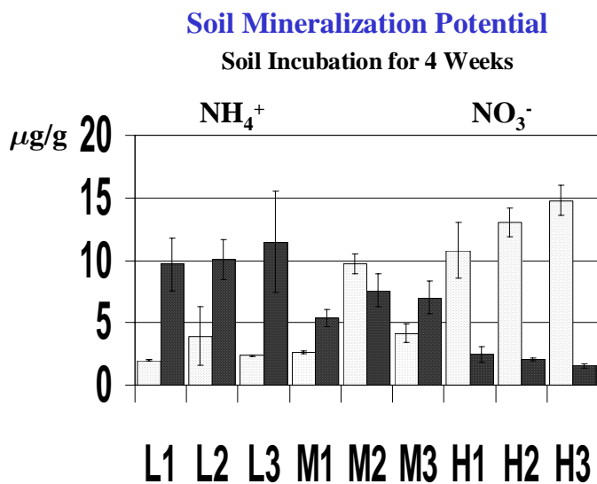
Figure 5-19. Soil Mineralization Potential for soil samples incubated in the laboratory for four weeks. Note that ammonium (NH 4 + ) is more concentrated in the Low disturbance sites, while nitrate (NO 3 - ) is more concentrated in the High disturbance sites.
