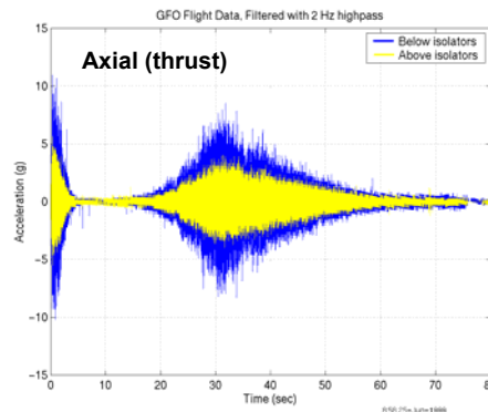
Figure 7 GFO flight data – below and above isolators
