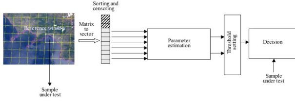
Fig. 1. Scheme of the CFAR detector.
