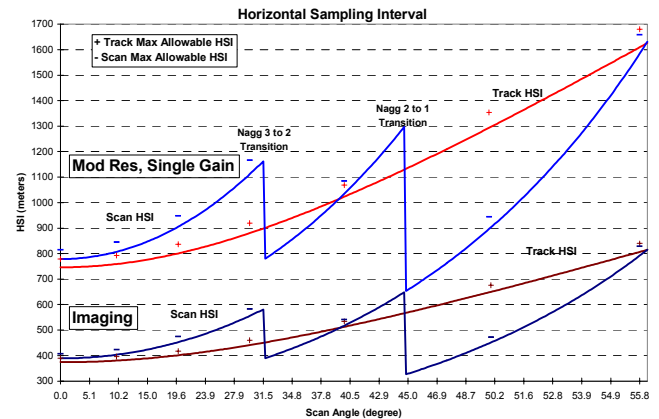
Figure 3. Track and scan HSI for moderate and imaging bands.
