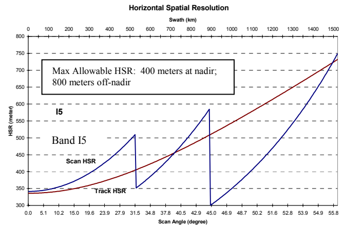
Figure 4. Track and scan HSR for imaging band I5.
