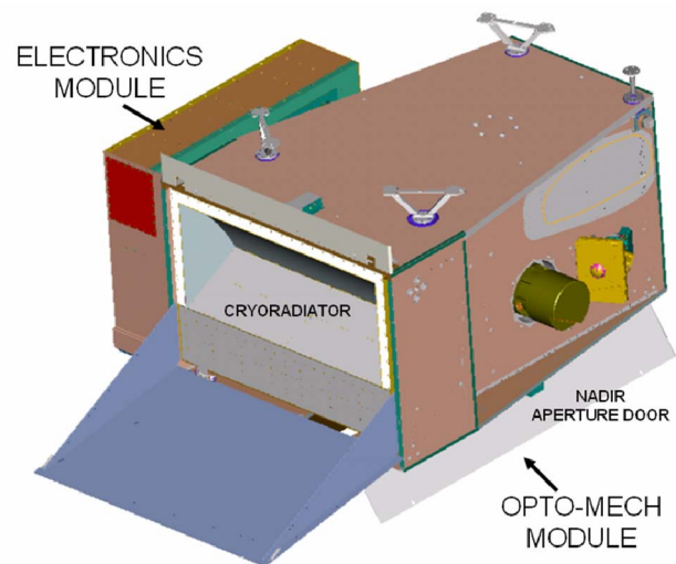
Fig. 1. General configuration of VIIRS instrument
