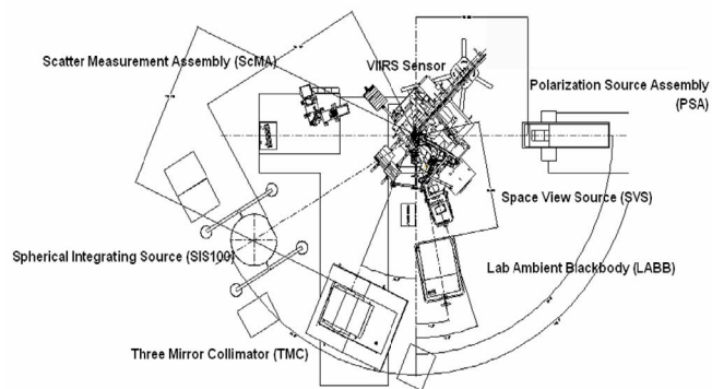
Fig. 2. VIIRS ambient testing laboratory plan view
