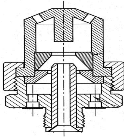
Figure 4 Simulant Dispersal Atomizing Spray Nozzle
