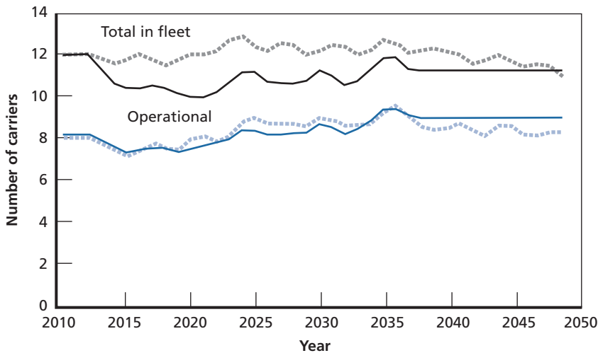
Figure 2.12 Fleet Size Sustained by Build-New Strategy with No RCOH After CVN 71 (24/71)
