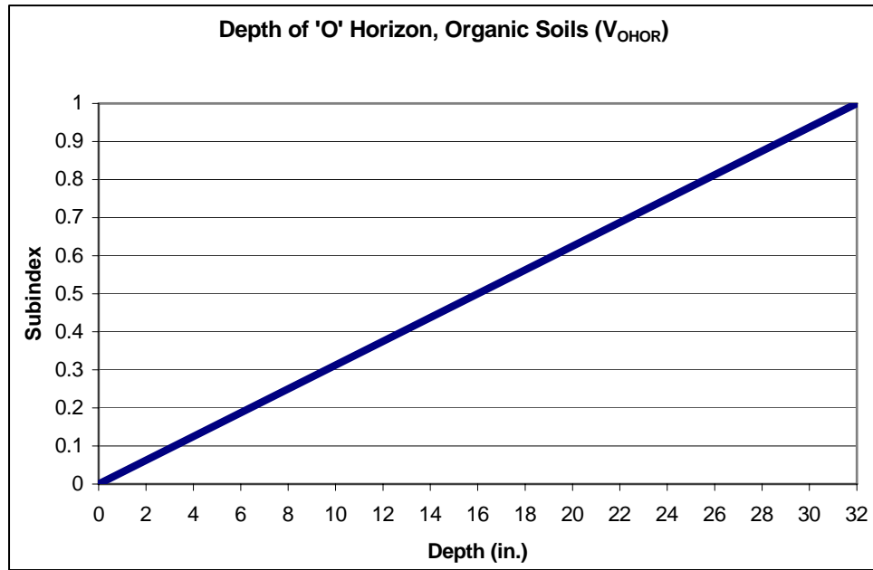
Figure 27. Relationship between 'O' horizon depth and subindex score in organic soils in Isolated Depressions and Floodplain Depressions
