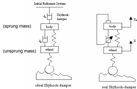
Figure 8: Principle of sky-hook damping [52]
