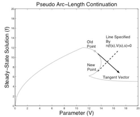
Figure 2: Arclength Continuation
