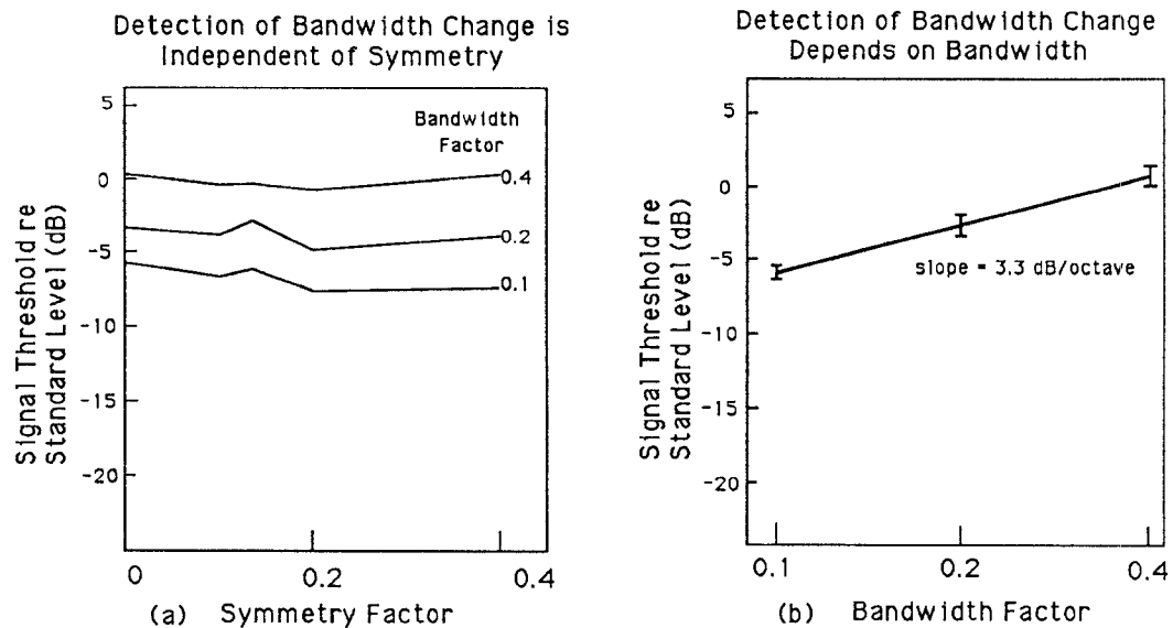
Fig. 8. (a) Detection threshold of bandwidth change as a function of SF for three different BWF's. (b) Average detection thresholds as a function of BWF of the standard .
