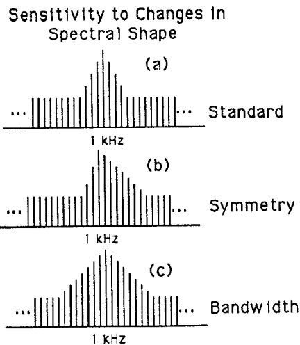
Fig. 5. (a) Complex waveform consists of an equal amplitude base and a peak added to it. Peak takes different symmetries (b) and bandwidths (c).
