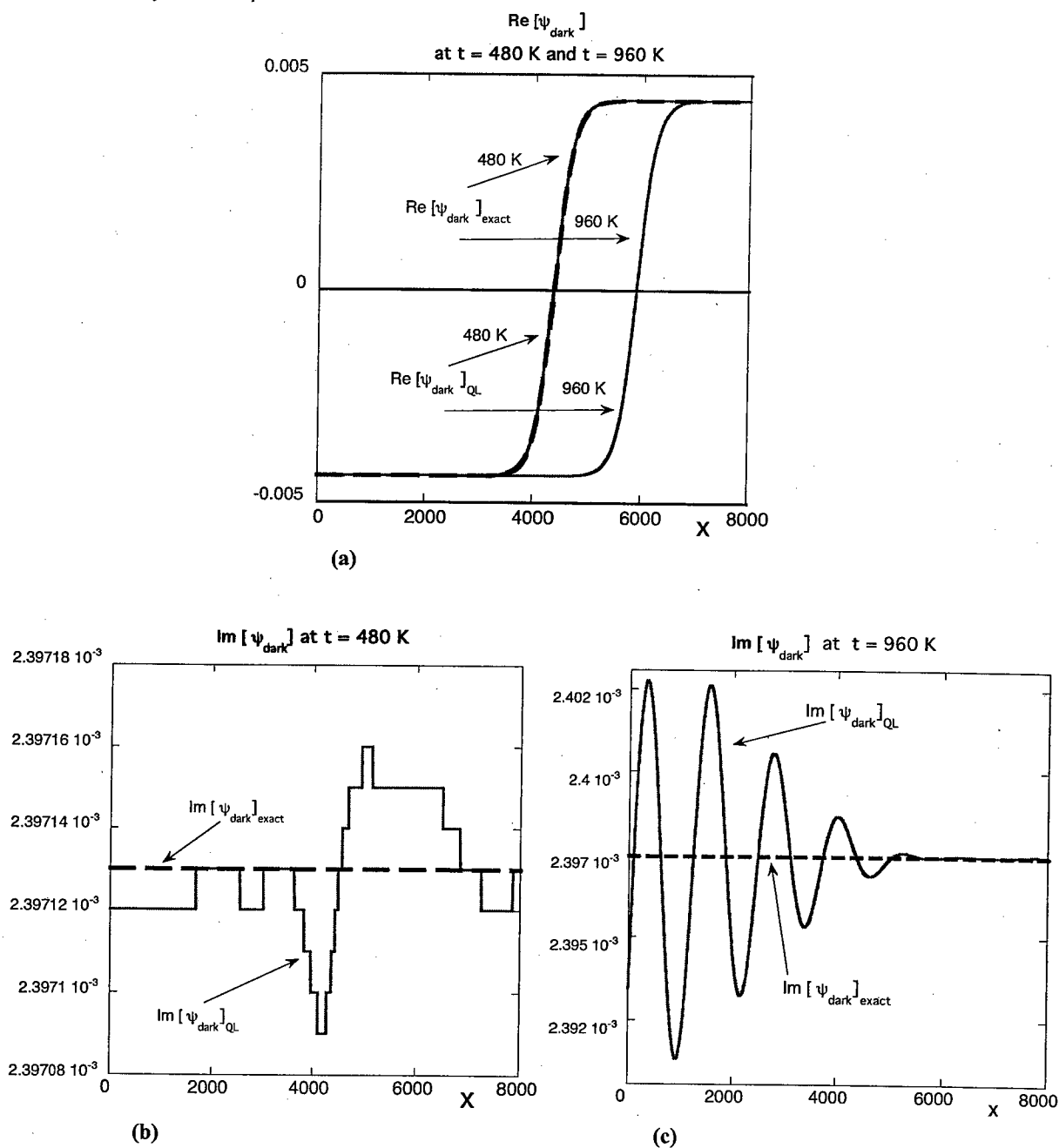
Fig. 6 A plot of (a) \text{Re}[\psi_{\text{dark}}]_{\text{QL}} and \text{Re}[\psi_{\text{dark}}]_{\text{exact}} at t = 480 K and t = 960 K. Even at t = 960 K, the relative error is less than 0.07%. \text{Im}[\psi_{\text{dark}}]_{\text{QL}} and \text{Im}[\psi_{\text{dark}}]_{\text{exact}} = \text{const.} at (b) t = 480 K, (c) t = 960 K. The extremely low numerical noise at t = 480 K (errors < 0.002%) has been amplified to structured oscillations with errors < 0.2%. The (theoretical) phase discontinuity of \psi_{\text{dark}} about its minimum is 0.71\pi [see (a) – (c)].
