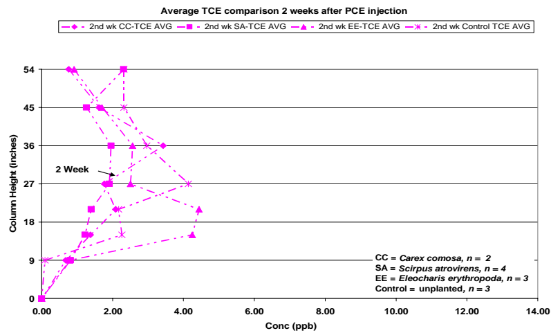
Figure 4.11 TCE data 2 weeks after injections began
