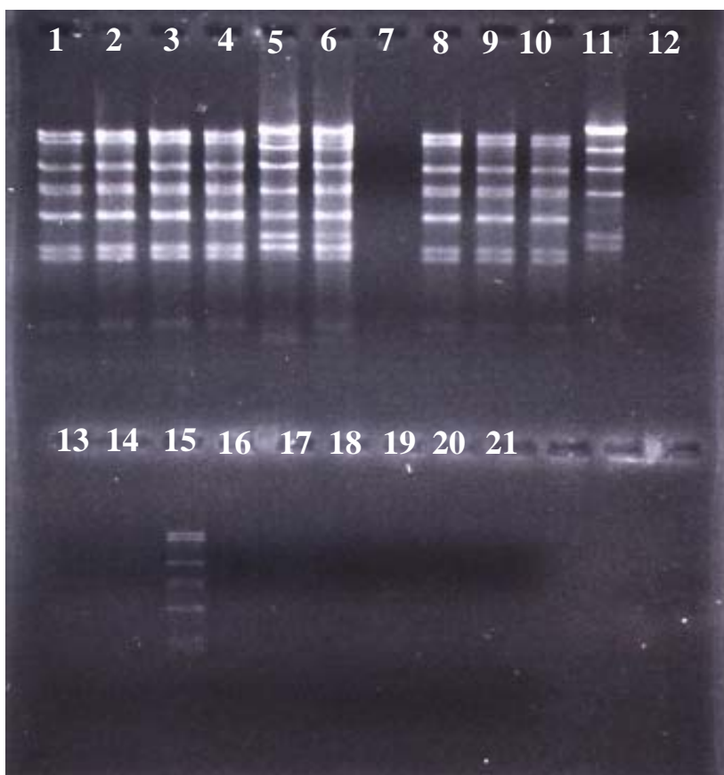
FIGURE 4. Effects of Chlorine Exposure at 85°C for 1 Minute on Lambda Bacteriophage DNA ( Hind III Digest) as Observed by Agarose Gel Electrophoresis.
