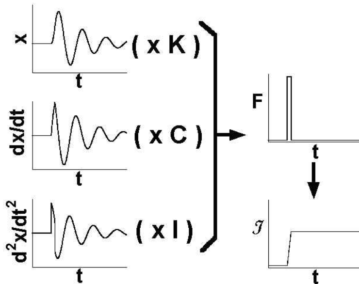
FIGURE 2. Schematic representation of the process for deriving the time-varying impulse or force from the balance's deflection and its derivatives.
