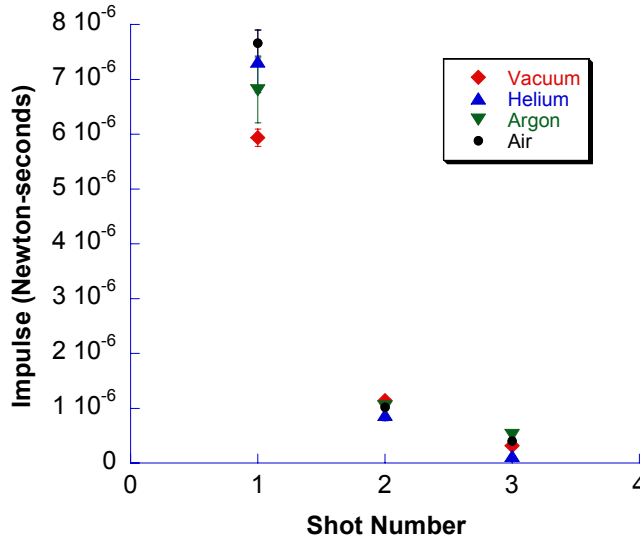
FIGURE 6. Impulse as a function of the number of laser pulses at a particular material site in various environments.
