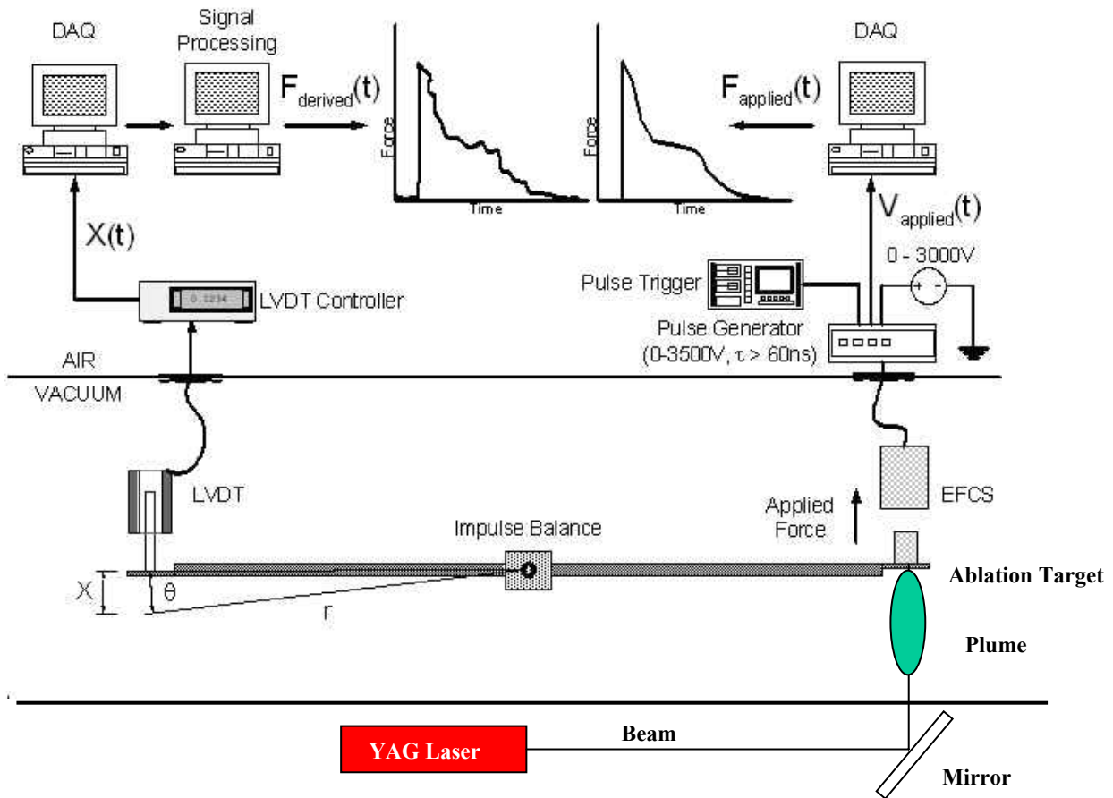
FIGURE 1. Experimental set up for time resolved impulse and laser ablation measurements.
