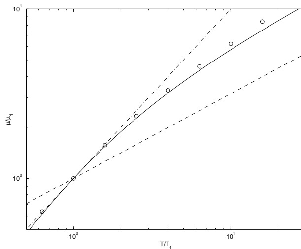
FIGURE 1. Viscosity for: —, Sutherland, Eq. 1; --, hard sphere \mu/\mu_1 = (T/T_1)^{\frac{1}{2}} ; · - ·, linear law \mu/\mu_1 = T/T_1 . \circ argon data Kestin et al. [1] T_1 = T_3 = 142 K, \mu_1 = 1.129 \times 10^{-5} Nm -1 s -1 .
