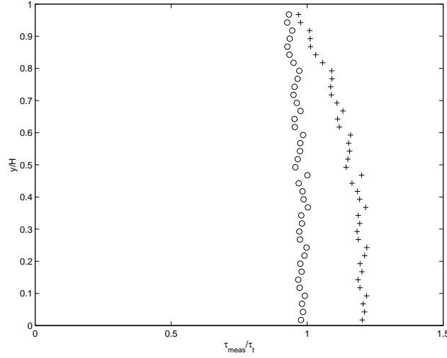
FIGURE 2. Measured shear stress in Couette flow simulation using \mu -DSMC and Sutherland viscosity, compared with theoretical shear stress \tau_t = \mu_t (T_{meas}) du_x/dy_{meas} . o, \mu_t from Eq. 1 (Sutherland); +, \mu_t = (T/T_1)^{1/2} (hard sphere). Origin of y -axis mid-way between the plates. Distance between plates 2H . Nominal Knudsen number 2\mu_1/(\rho_1 \bar{c}_1 H) = 0.01 , \bar{c} = (8RT_1/\pi)^{1/2} , subscript 1 denotes undisturbed gas state. Wall temperature T_w = T_1 . Wall speed V_w = 3(2RT_1)^{1/2} . Only 1 in 5 points shown. From Ref. [11].
