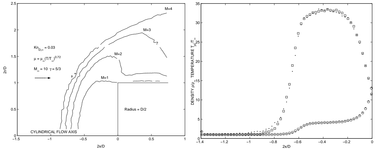
FIGURE 5. Antisymmetric flow about a blunt-faced cylinder. \nu -DSMC compared with standard VHS model. M_\infty = 10 , T_w/T_\infty = 0.26 , \gamma = 5/3 , \mu/\mu_\infty = (T/T_\infty)^{0.72} , Kn_{D,\infty} = 2\mu_\infty/(\rho_\infty \bar{c}_\infty D) = 0.03 . (a) Mach number contours: --, VHS; —, \nu -DSMC. (b) Temperature T_x and density \rho in cells adjacent to the stagnation streamline. \square , VHS; \bullet , \nu -DSMC.
