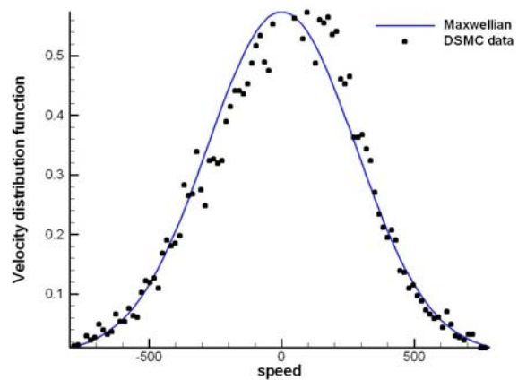
FIGURE 5. Velocity distribution curves at Kn = 5
