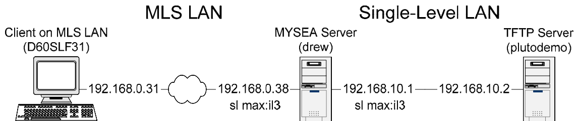
Figure 8. Test Network Topology
