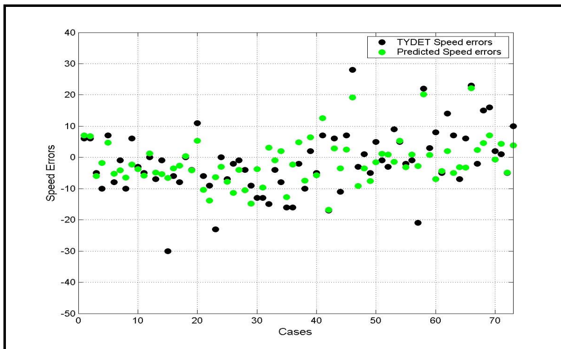
Figure 48. The original 48-h TYDET speed errors (kt) (black) and the speed errors (kt) predicted by the linear regression (green) procedure for all TC cases in which Kadena AB was in the right-front quadrant.
