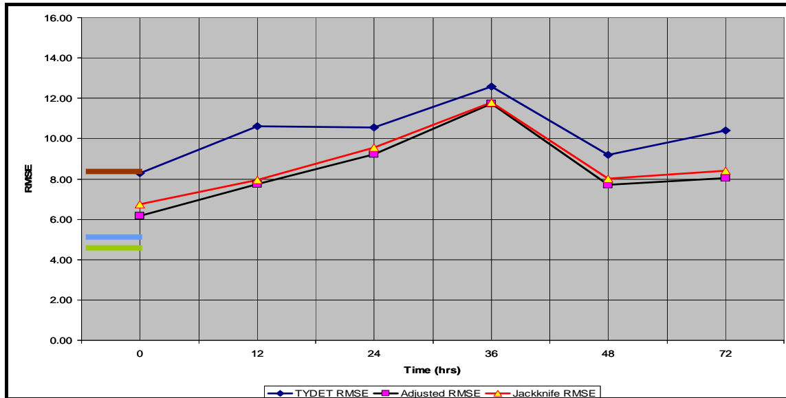
Figure 61. Cross-wind RMSE (kt) for the original TYDET winds (blue), adjusted winds (black)), and the jackknife winds (red) based on the speed regression for the storms in which Kadena AB is in the right-front quadrant. The values for the time 0 h that are derived from best-track values are shown to the left as a baseline for these results of regressions based on JTWC forecasts at the times (h) shown.
