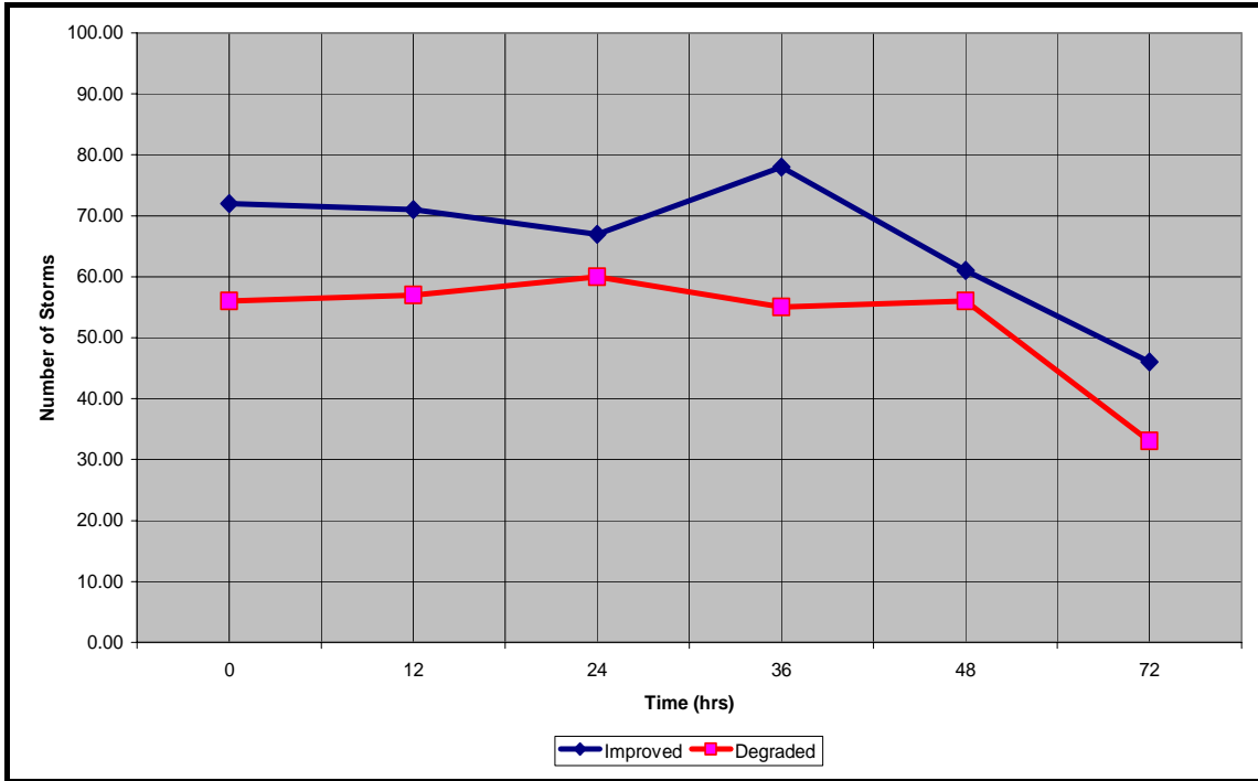
Figure 65. Numbers of cross-wind forecasts improved (blue) and degraded (red) for the cases in which the values from the speed regression were used. The values were calculated for the combined sample of storms in which Kadena AB was in the right-front and right-rear quadrant storms affecting Kadena AB using JTWC forecast data.
