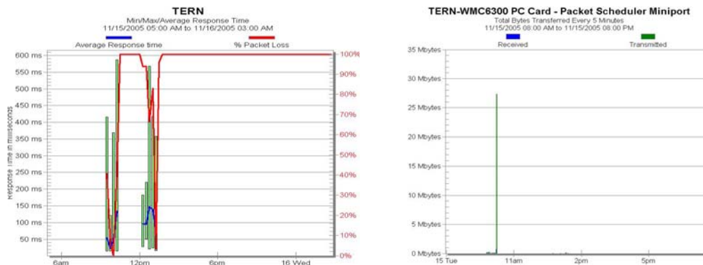
Figure 40. TERN UAV Response Time
