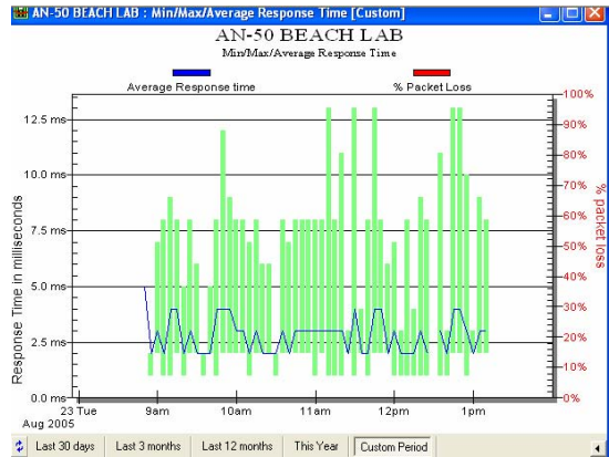
Figure 30. NPS-Camp Roberts Link
