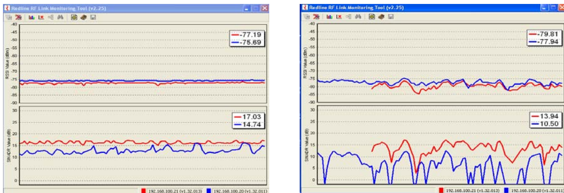
Figure 34. Normal RSSI and Irregularities for the REAL AN-50
