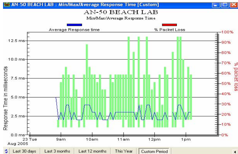
Figure 21. Backbone Latency
