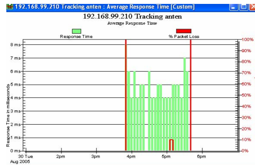
Figure 27. Tracking Antenna
