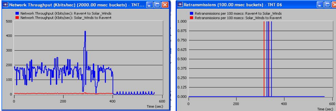
Figure 51. Network Throughput and Retransmissions
