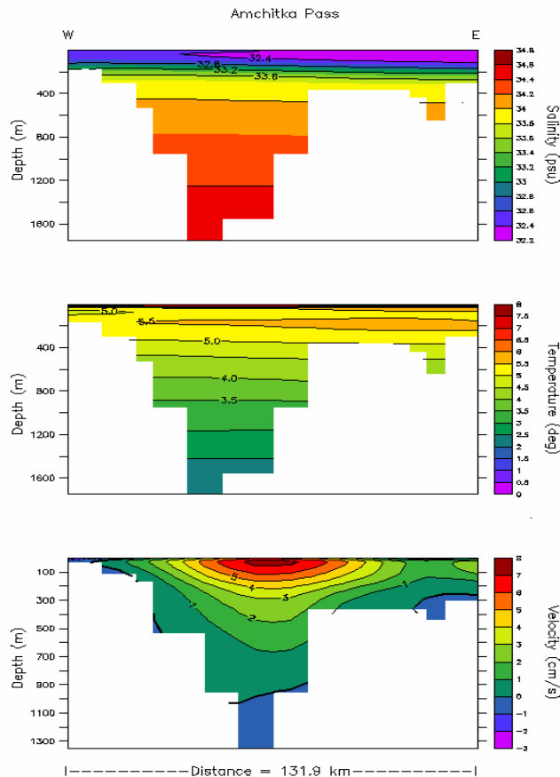
Figure 41. Twenty-five-year mean (1979-2003) profile of salinity (psu), temperature (deg), and velocity (cm s ^{-1} ) for Amchitka Pass. Positive velocity is directed northward.
