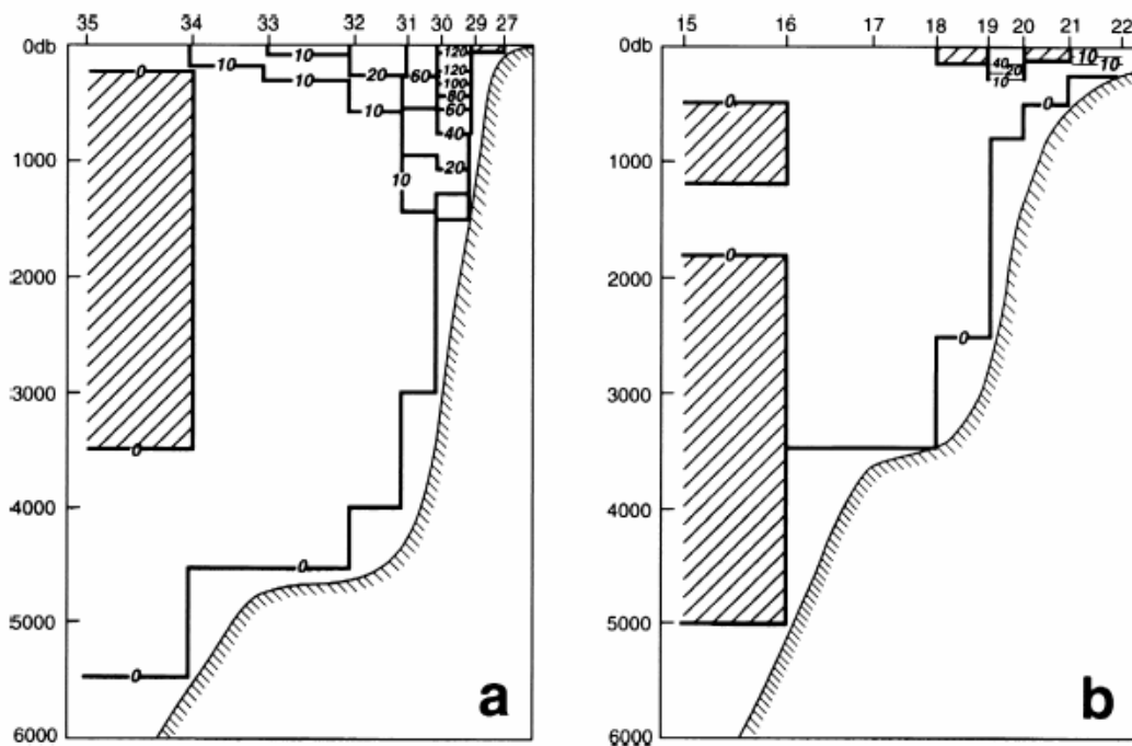
Figure 18. Vertical sections of geostrophic speed ( \text{cm s}^{-1} ). Figure 17(a) is located at 173.5^\circ\text{W} , and measured during the time period 24-25 May 1997. Figure 17(b) is located at \sim 170^\circ\text{W} , and measured during 22-23 May 1997. Hatched areas indicate eastward flow [from Reed and Stabeno, 1999]
