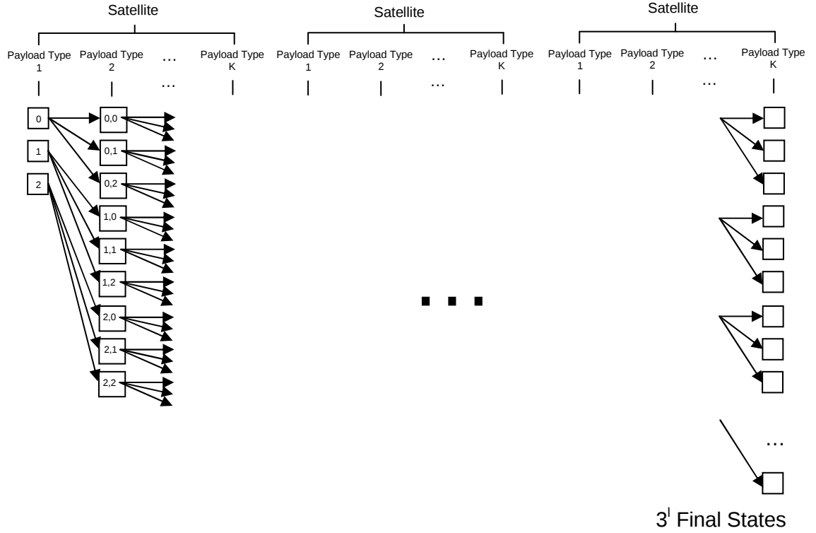
Figure 3.1 Graphical depiction of a dynamic programming solution ( \xi = 2 ).
