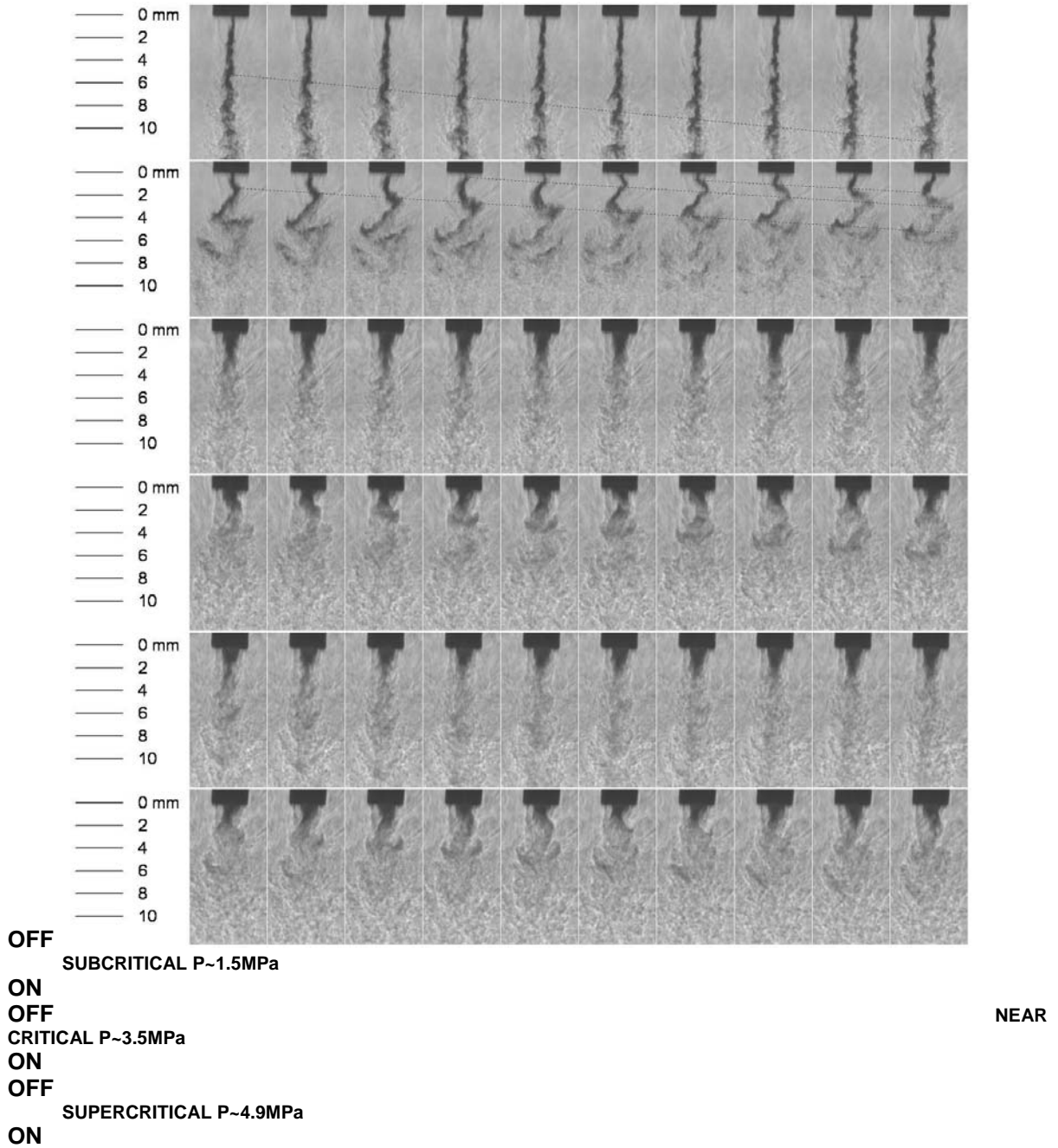
Figure 3. Consecutive frames from high-speed shadowgraph images with the acoustic driver turned off and on at ~3kHz. Time increases from left to right with an interval of 55.6 \mu\text{s} between frames. The first two rows are at a subcritical chamber pressure (~ 1.5 MPa), the third and fourth rows are at a near-critical chamber pressure (~ 3.5 MPa), and the fifth and sixth rows are at a supercritical chamber pressure (~ 4.9 MPa). The acoustic driver is turned off for the first, third, and fifth rows and on for the second, fourth, and sixth at ~ 3 kHz. The light gray lines in the first and second rows connect fluid structure as they evolve in time.
