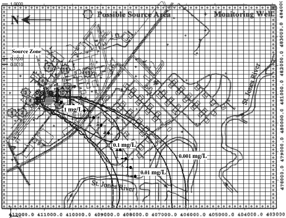
Figure 30. PCE Plume
