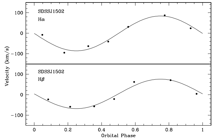
FIG. 3.—H \alpha velocity curve of SDSSJ 1502 with the best-fit sinusoid (Table 4) superposed.
