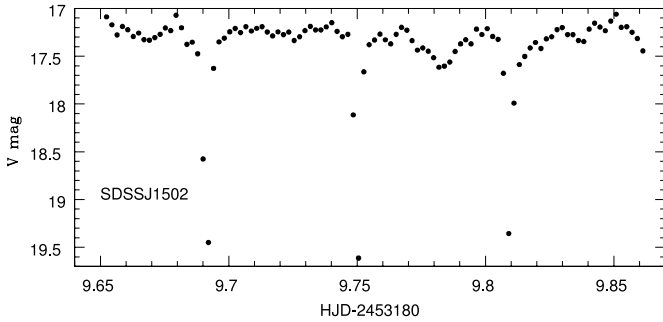
FIG. 2.—Light curve of SDSSJ 1502 showing three eclipses. Error bars are \leq 0.02 mag, except during eclipses, when they are up to 0.09 mag.
