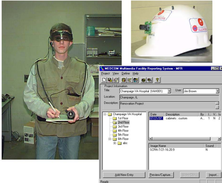
Figure 3. The Digital Hardhat System
