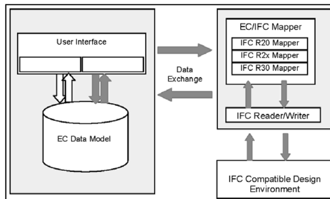
Figure 2. Building Commissioning based IFC Test Rig
