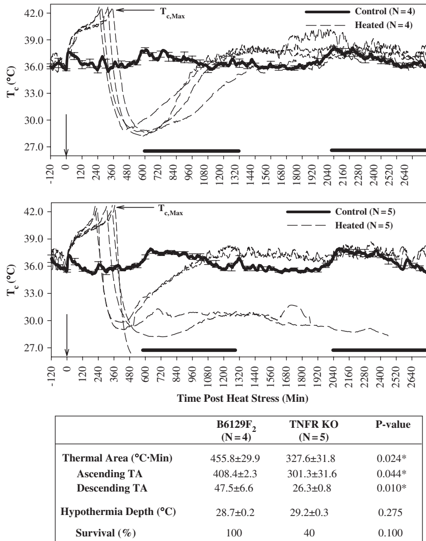
Fig. 6. 48 h core temperature ( T_c ) response of male B6129F 2 (wild-type; top) and TNFR knockout (bottom) mice during heat exposure ( T_a = 39.5 \pm 0.2^\circ\text{C} ) to a maximum T_c ( T_{c,\text{Max}} ) of 42.7^\circ\text{C} and recovery at T_a of 25 \pm 2^\circ\text{C} . Note that TNFR knockout mice had significantly lower total, ascending (thermal load) and descending TA (slower cooling rate) compared to wild-type mice. Hypothermia depth and survival did not differ between groups. Sample sizes are indicated in parentheses. T_c was collected at 1-min intervals using the intraperitoneal implantation of a radiotelemetry device. Arrow at time 0 represents start of heat exposure. Black horizontal bars represent lights-off period on a 12:12 h L:D cycle (lights on at 0700 h).
