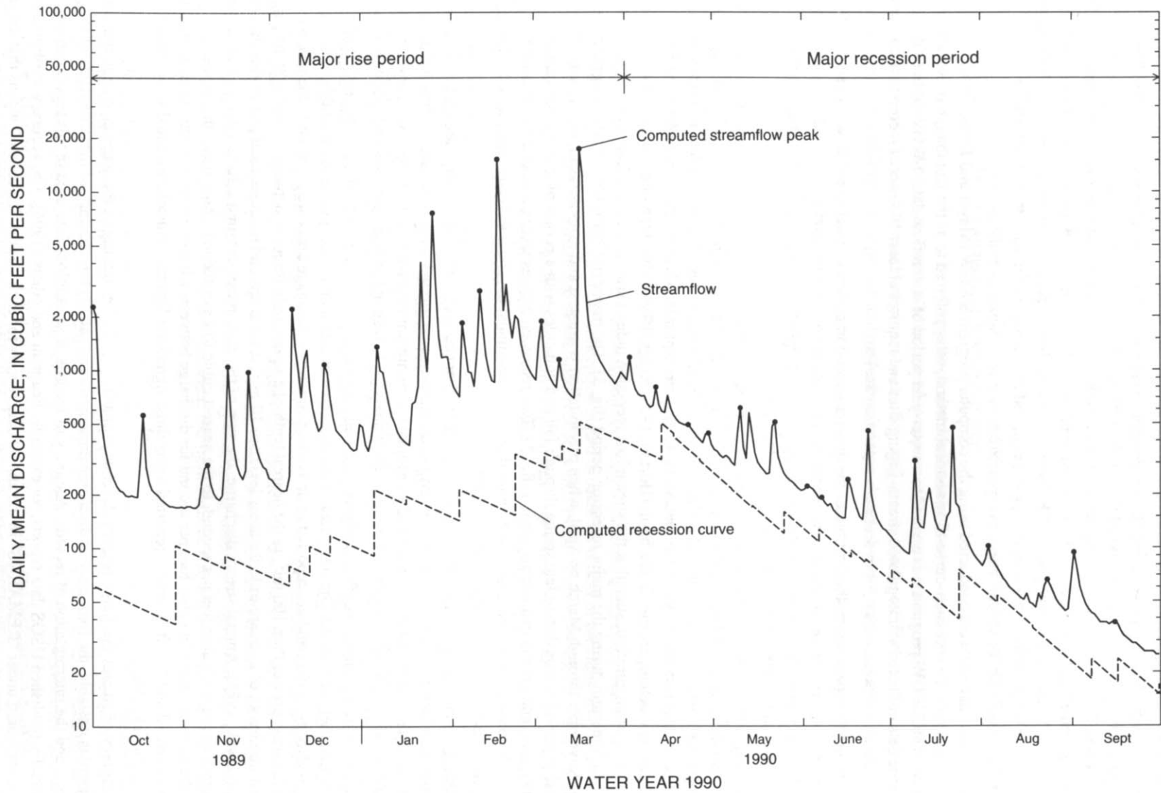
Figure 3. Streamflow hydrograph, separated by program SWGW.
