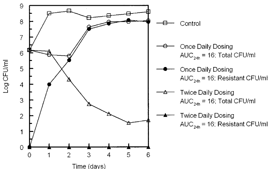
FIG. 5. Effect of dose schedule on efficacy of ciprofloxacin against B. anthracis . A ciprofloxacin exposure of an AUC_{24} of \text{mg} \cdot \text{h}/\text{liter} ( AUC_{24}/\text{MIC} = 256 ) was given as two equal doses at 12-h intervals or as a single dose at 24-h intervals. The twice-daily regimen substantially reduced the total culture density and no resistant organisms were observed. Daily dosing prevented culture growth for 2 days, but the culture density increased to near control levels thereafter. Resistant organisms emerged after 1 day and replaced the susceptible organisms in the culture by day 2. The growth of an untreated control is also shown.
