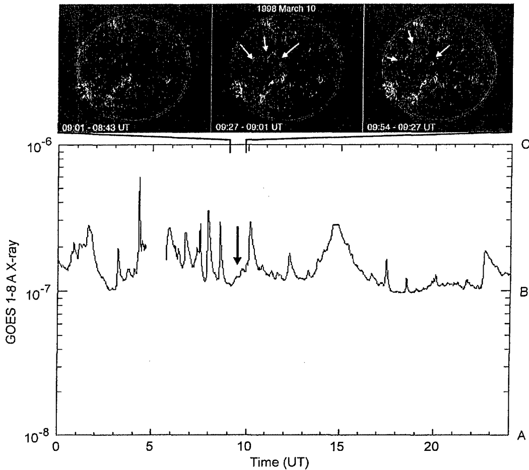
FIG. 2.—Top: EIT running difference images showing the development of the wave on 1998 March 10. White arrows are used to indicate the leading edge of the wave. Bottom: GOES 1–8 Å plot for 1998 March 10, with the B1 soft X-ray flare associated with the wave indicated by an arrow. “A,” “B,” and “C” in the right-hand margin indicate GOES peak soft X-ray classes.
