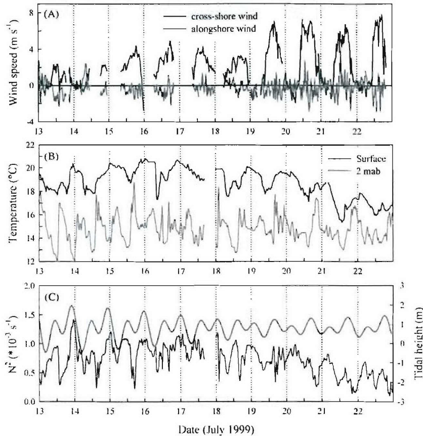
Fig. 3. Wind speed (A), water temperature (B) and mean stratification of the water column (C) during the drifter deployments at Bahia Salsipuedes in July 1999. Tidal heights predicted for the port of Ensenada, Baja California, are also shown in C (gray line).
