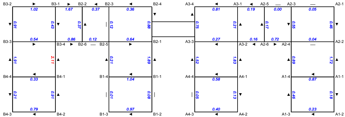
Figure 10. Predicted elevation differences (in inches) between adjacent support columns of the Elevated Station on 1 January 2006. (Arrows indicate downslope direction of grade beam. If a dash is present instead of an arrow, the grade beam is at or very near level. Values in red indicate column pairs that exceed design limits for differential elevation.)
