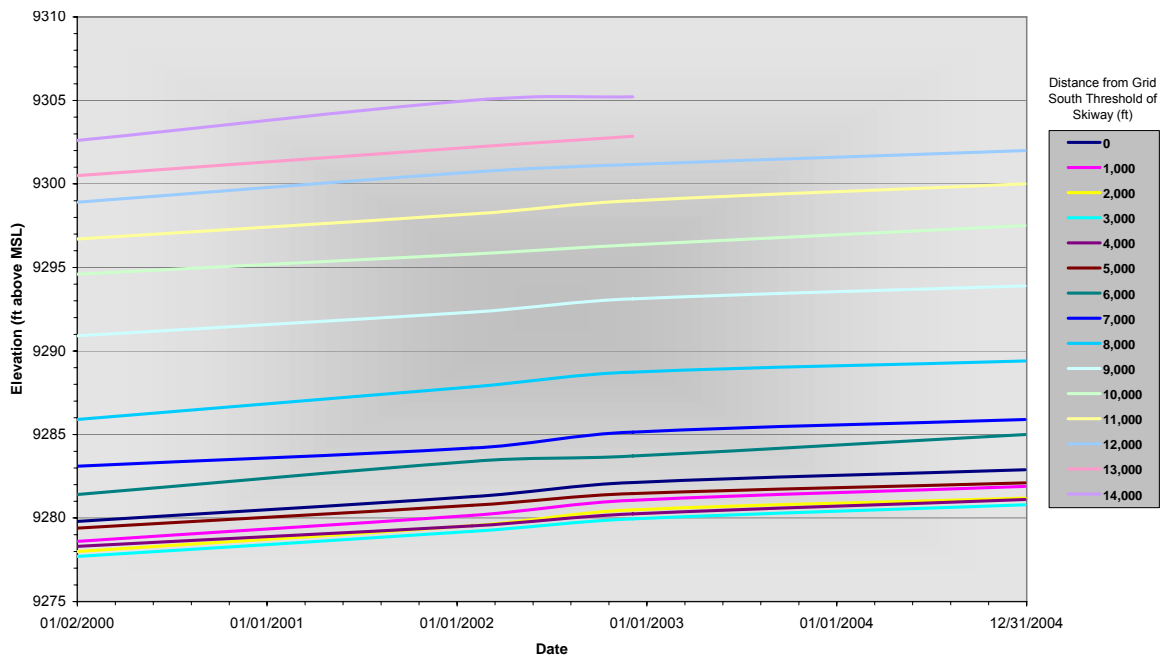
Figure 16. History of South Pole skiway elevation for 1000-ft stations along its centerline.
