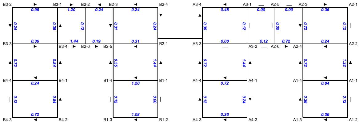
Figure 9. Elevation differences (in inches) between adjacent support columns of the Elevated Station based on survey data collected on 31 December 2004. (Arrows indicate downslope direction of grade beam. If a dash is present instead of an arrow, the grade beam is at or very near level.)
