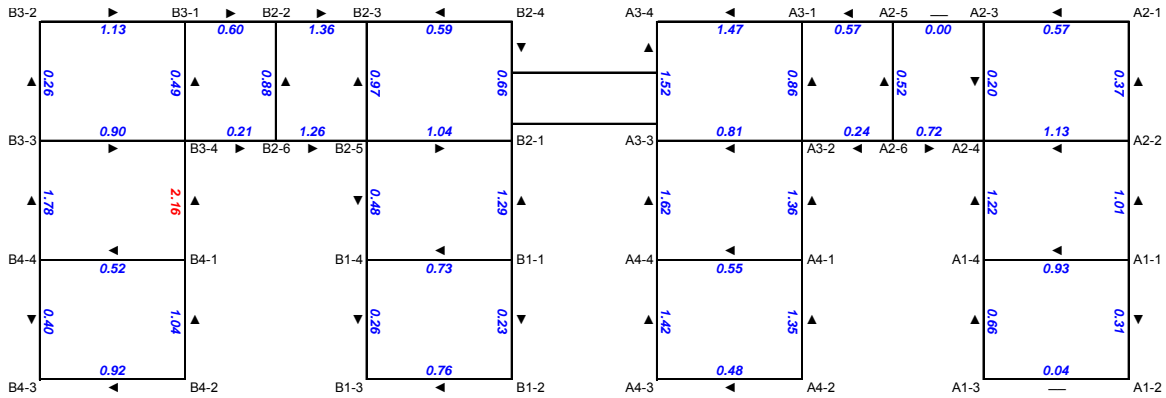
Figure 15. Predicted elevation differences (in inches) between adjacent support columns of the Elevated Station on 1 January 2008 following recommended shimming (Table 3). (Arrows indicate downslope direction of grade beam. If a dash is present instead of an arrow, the grade beam is at or very near level. Values in red indicate column pairs that exceed design limits for differential elevation.)
