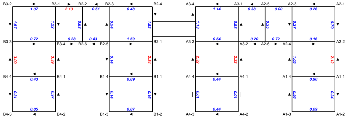
Figure 11. Predicted elevation differences (in inches) between adjacent support columns of the Elevated Station on 1 January 2007. (Arrows indicate downslope direction of grade beam. If a dash is present instead of an arrow, the grade beam is at or very near level. Values in red indicate column pairs that exceed design limits for differential elevation.)
