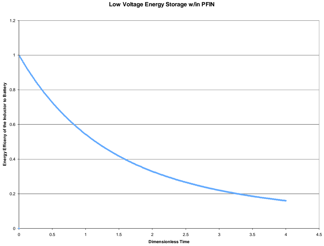
Figure 23. Ratio of inductor energy to battery energy, \frac{W_L}{W_B} , versus dimensionless time,
