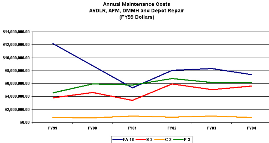
Figure 5. Aircraft Annual Maintenance Costs (FY99 dollars)
